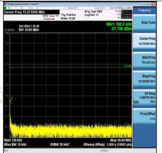
Band26(824-849)-3MHz-QPSK-26915-15RB#0-0 .15~30-PASS
