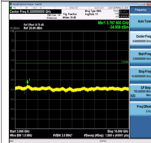
Band26(824-849)-3MHz-16QAM-26915-1RB#14 -3000~10000-PASS
