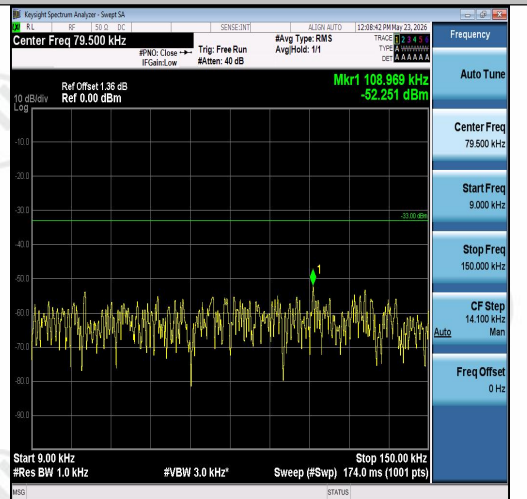
Band26(824-849)-3MHz-16QAM-26915-15RB#0 -0.009~0.15-PASS
