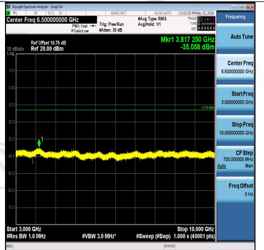
Band26(824-849)-3MHz-16QAM-26805-15RB#0 -3000~10000-PASS
