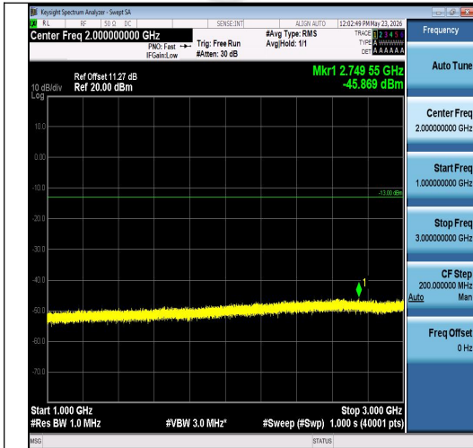
Band26(824-849)-3MHz-16QAM-26805-15RB#0 -1000~3000-PASS
