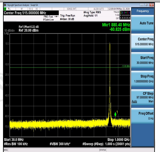
Band26(824-849)-3MHz-16QAM-26915-15RB#0 -30~1000-PASS
