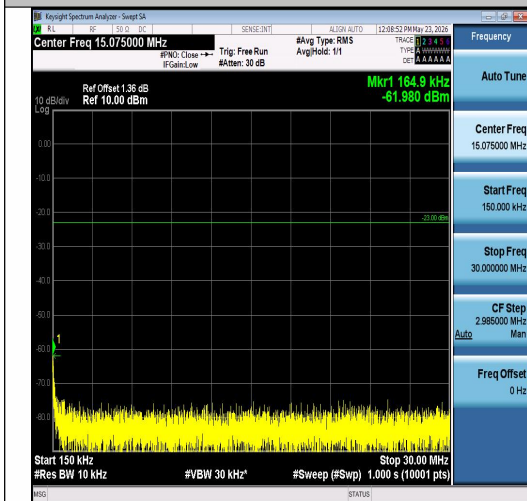
Band26(824-849)-3MHz-16QAM-26915-15RB#0 -0.15~30-PASS
