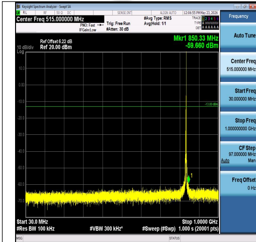
Band26(824-849)-3MHz-16QAM-26915-1RB#14 -30~1000-PASS
