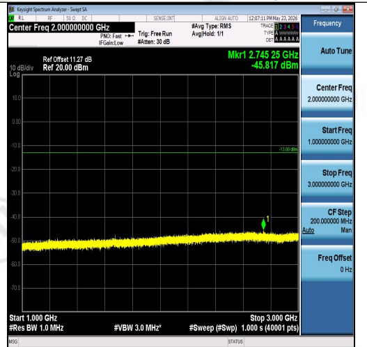
Band26(824-849)-3MHz-16QAM-26915-1RB#14 -1000~3000-PASS
