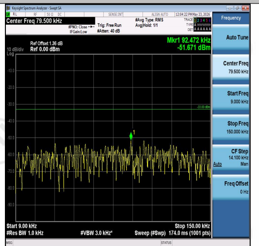
Band26(824-849)-3MHz-16QAM-26915-1RB#0-0 0.009~0.15-PASS
