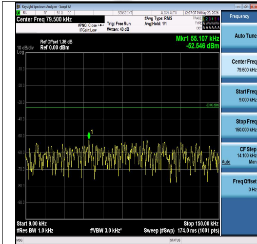
Band26(824-849)-3MHz-QPSK-26915-15RB#0-0 .009~0.15-PASS
