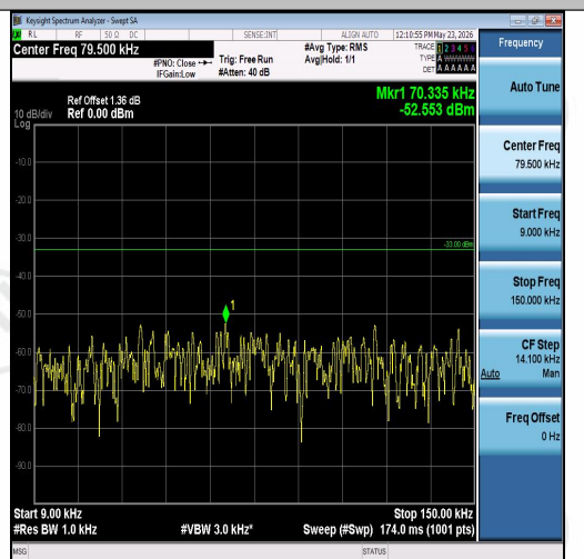
Band26(824-849)-3MHz-16QAM-27025-1RB#0- 0.009~0.15-PASS
