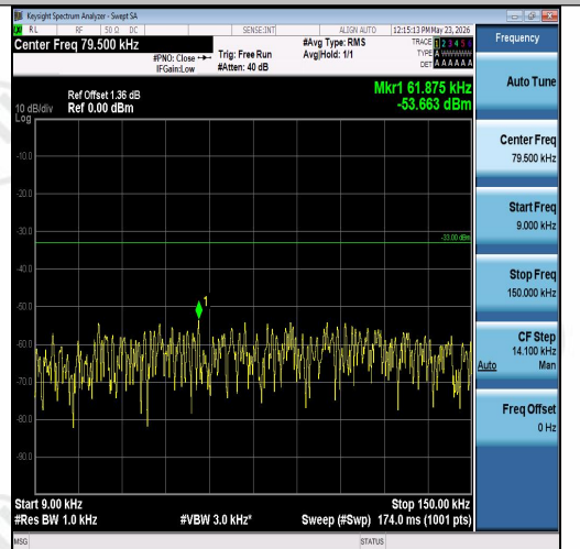
Band26(824-849)-3MHz-16QAM-27025-15RB#0 -0.009~0.15-PASS
