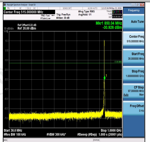
Band26(824-849)-3MHz-16QAM-27025-15RB#0 -30~1000-PASS
