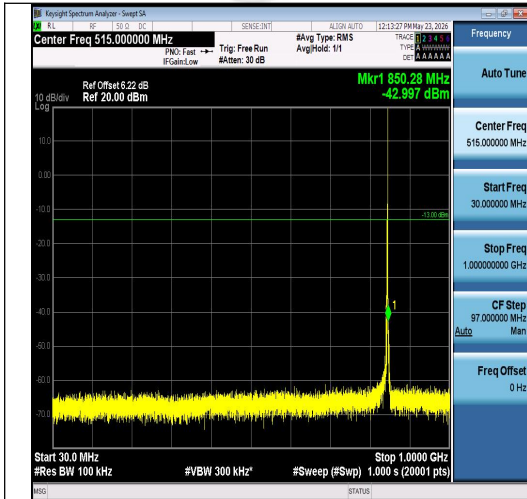
Band26(824-849)-3MHz-16QAM-27025-1RB#14 -30~1000-PASS
