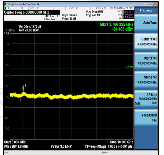
Band26(824-849)-3MHz-16QAM-26915-15RB#0 -3000~10000-PASS
