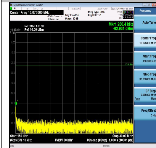
Band26(824-849)-3MHz-16QAM-27025-15RB#0 -0.15~30-PASS
