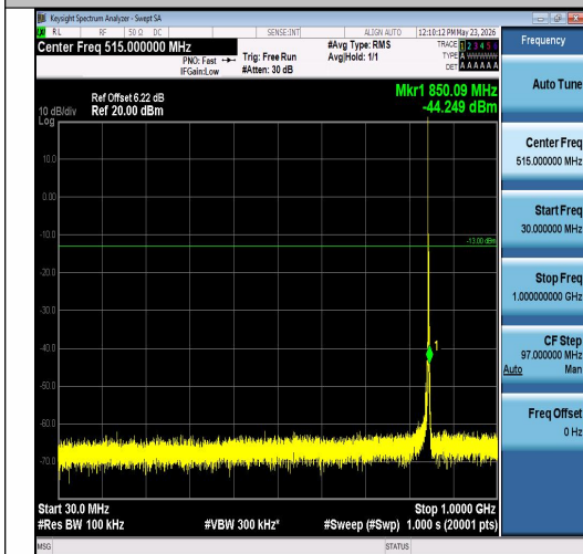
Band26(824-849)-3MHz-QPSK-27025-1RB#0-30 ~1000-PASS
