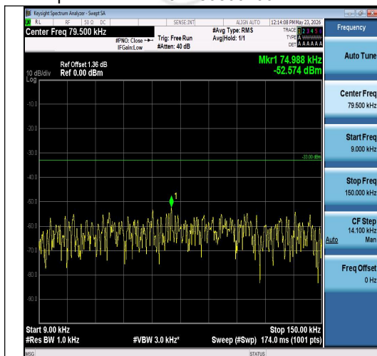
Band26(824-849)-3MHz-QPSK-27025-15RB#0-0 .009~0.15-PASS
