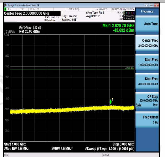
Band26(824-849)-5MHz-QPSK-26815-1RB#0-10 00~3000-PASS
