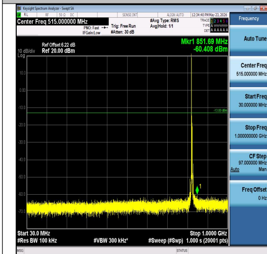
Band26(824-849)-5MHz-QPSK-26815-1RB#0-30 ~1000-PASS
