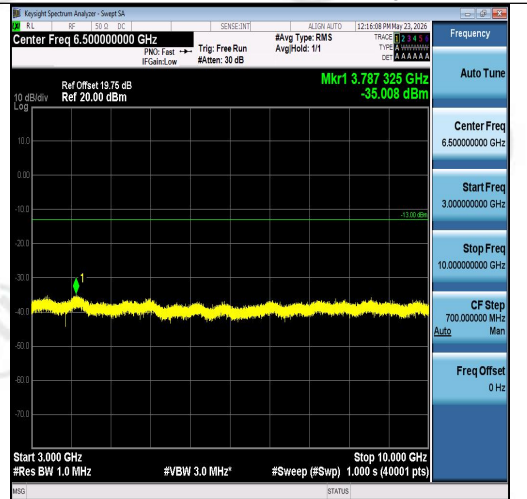
Band26(824-849)-3MHz-16QAM-27025-15RB#0 -3000~10000-PASS
