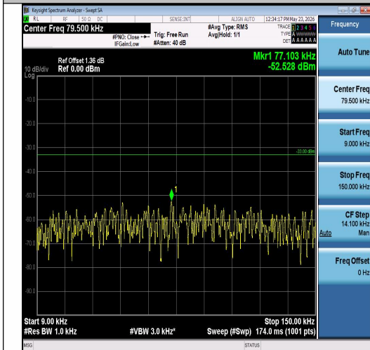
Band26(824-849)-5MHz-QPSK-26815-1RB#0-0. 009~0.15-PASS
