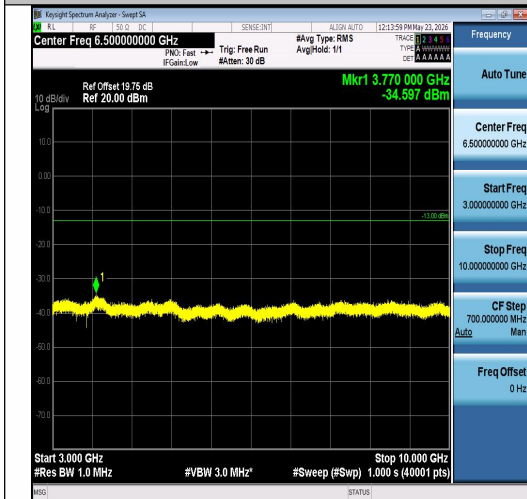
Band26(824-849)-3MHz-16QAM-27025-1RB#14 -3000~10000-PASS
