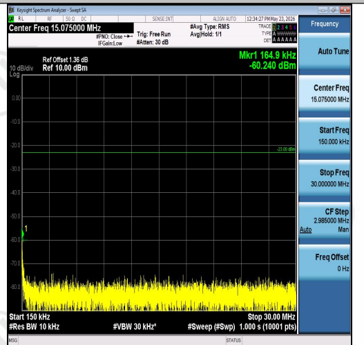
Band26(824-849)-5MHz-QPSK-26815-1RB#0-0. 15~30-PASS
