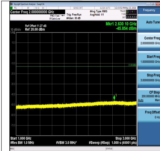
Band26(824-849)-3MHz-16QAM-27025-15RB#0 -1000~3000-PASS
