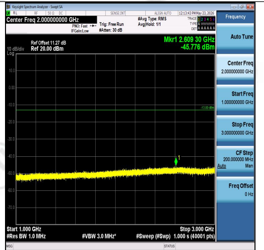
Band26(824-849)-3MHz-16QAM-27025-1RB#14 -1000~3000-PASS
