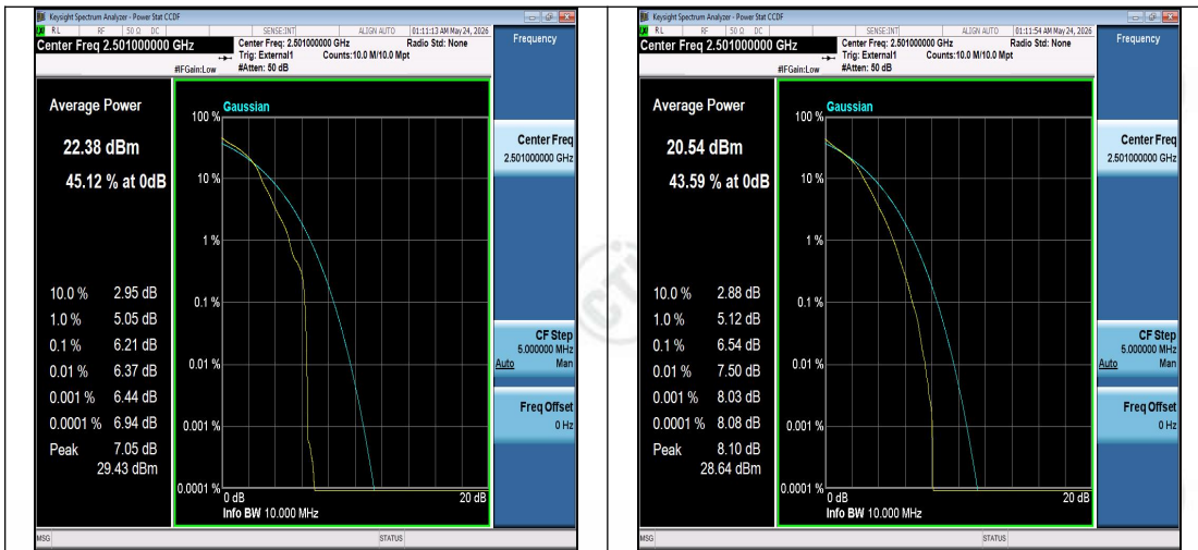
Band41-10MHz-16QAM-39700-1RB#0-PASS
