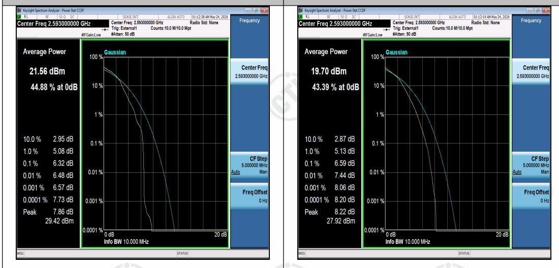
Band41-10MHz-QPSK-40620-1RB#0-PASS
