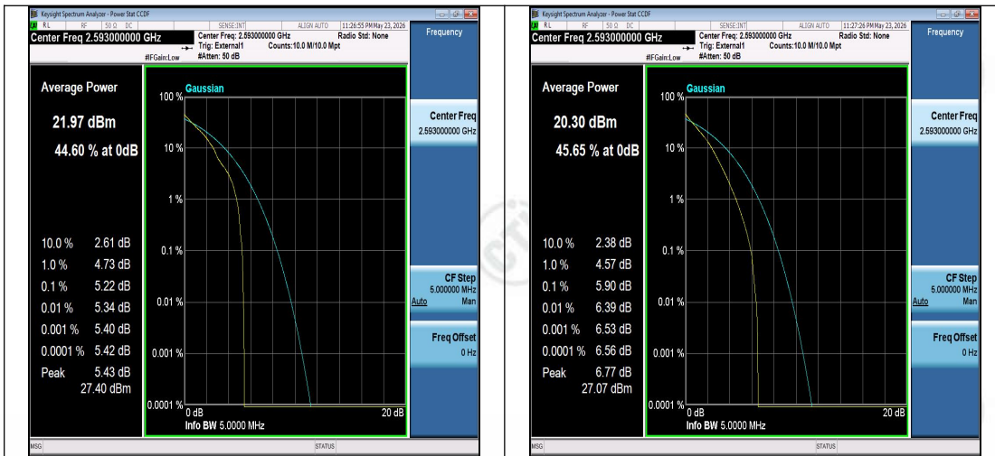
Band41-5MHz-QPSK-40620-1RB#0-PASS
