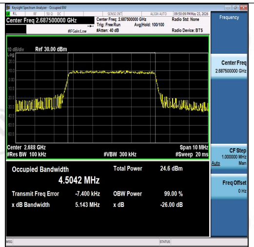
Band41-5MHz-16QAM-41565-25RB#0-PASS
