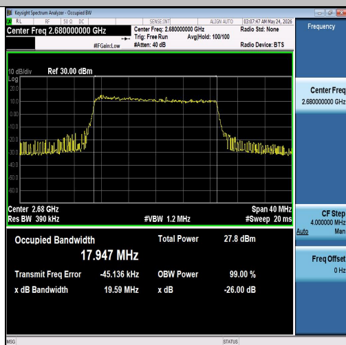
Band41-20MHz-QPSK-41490-100RB#0-PASS
