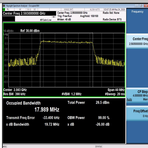
Band41-20MHz-QPSK-40620-100RB#0-PASS
