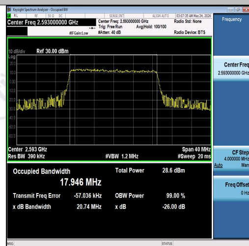
Band41-20MHz-16QAM-40620-100RB#0-PASS
