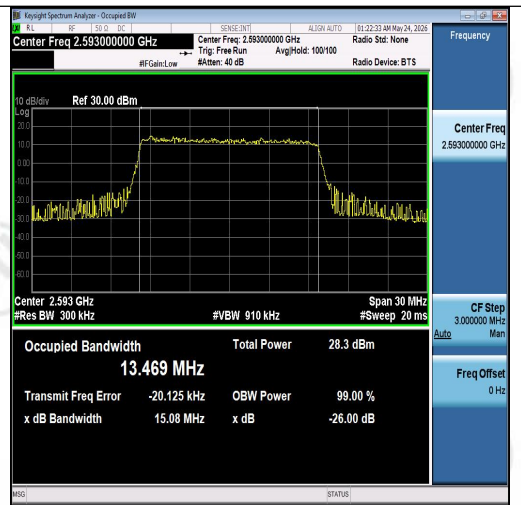
Band41-15MHz-16QAM-40620-75RB#0-PASS
