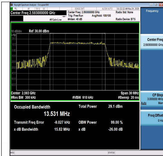
Band41-15MHz-QPSK-40620-75RB#0-PASS
