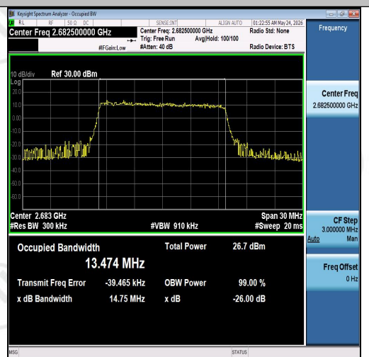
Band41-15MHz-16QAM-41515-75RB#0-PASS
