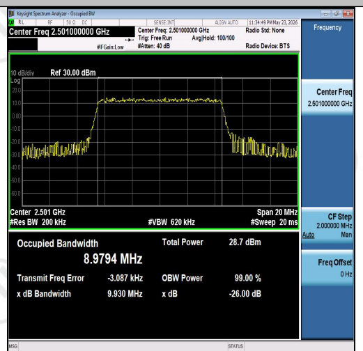
Band41-10MHz-16QAM-39700-50RB#0-PASS
