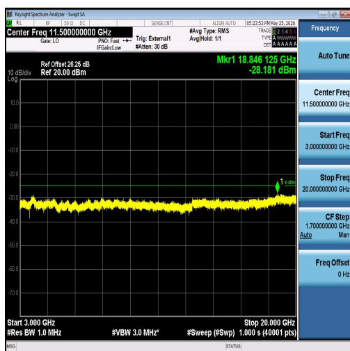
Band41-5MHz-16QAM-40620-1RB#24-3000~20000-PASS
