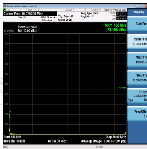
Band41-5MHz-16QAM-40620-25RB#0-0.15~30-PASS
