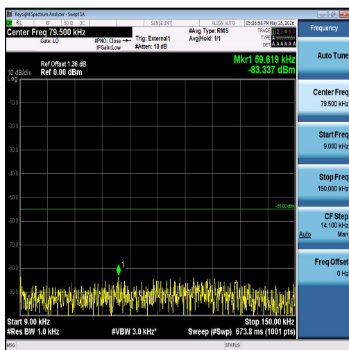
Band41-5MHz-16QAM-40620-25RB#0-0.009~0.15-PASS
