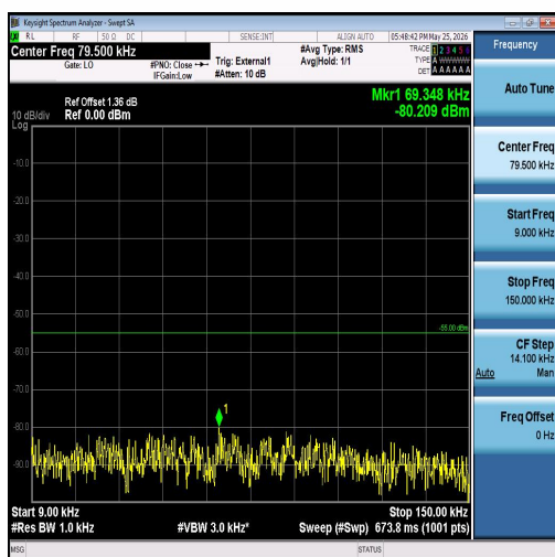
Band41-10MHz-16QAM-39700-1RB#0-0.009~0.015-PASS
