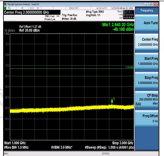
Band5-10MHz-QPSK-20450-50RB#0-1000~300 0-PASS
