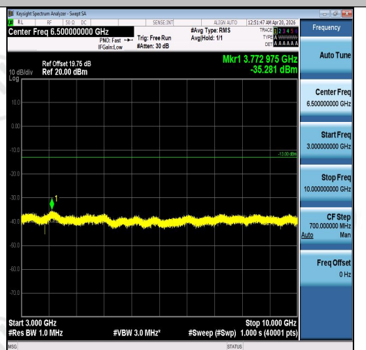
Band5-10MHz-QPSK-20450-1RB#49-3000~100 00-PASS
