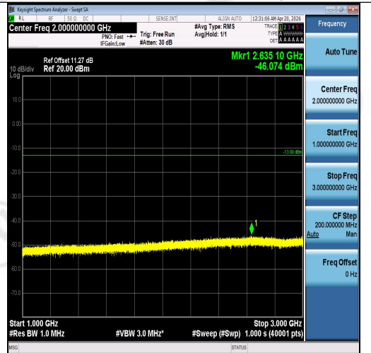
Band5-5MHz-QPSK-20625-25RB#0-1000~3000- PASS
