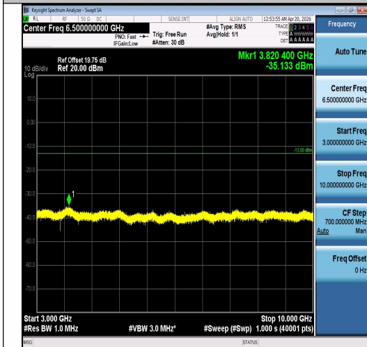
Band5-10MHz-QPSK-20450-50RB#0-3000~100 00-PASS
