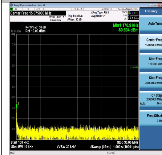
Band5-5MHz-16QAM-20625-1RB#0-0.15~30-PA SS
