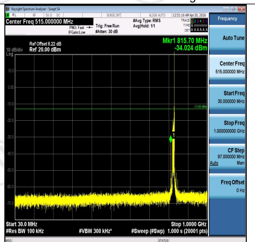
Band5-10MHz-QPSK-20450-1RB#49-30~1000-P ASS
