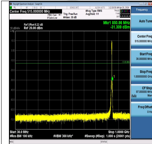
Band5-5MHz-QPSK-20625-25RB#0-30~1000-P ASS
