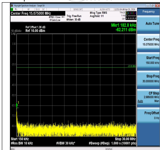
Band5-10MHz-QPSK-20450-1RB#49-0.15~30-P ASS
