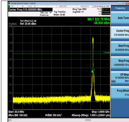
Band5-10MHz-QPSK-20450-50RB#0-30~1000-P ASS
