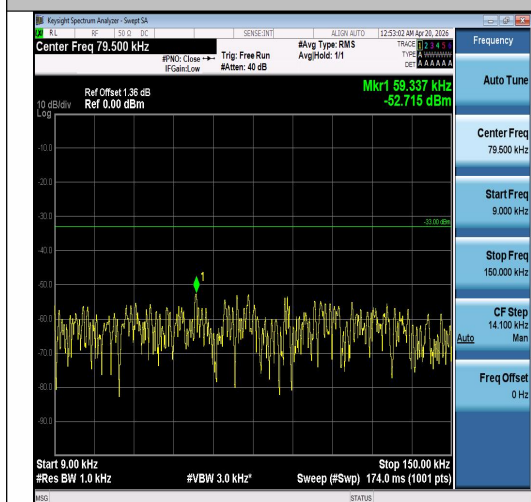
Band5-10MHz-QPSK-20450-50RB#0-0.009~0.1 5-PASS
