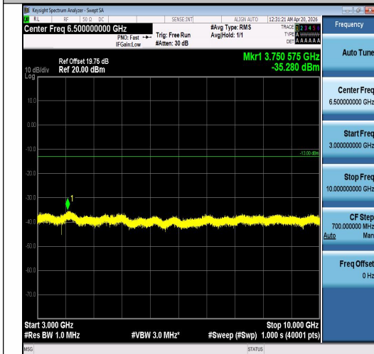
Band5-5MHz-QPSK-20625-25RB#0-3000~1000 0-PASS
