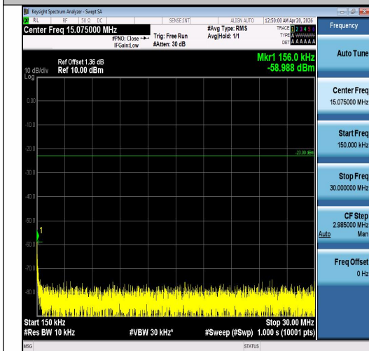
Band5-10MHz-16QAM-20450-1RB#0-0.15~30-P ASS
