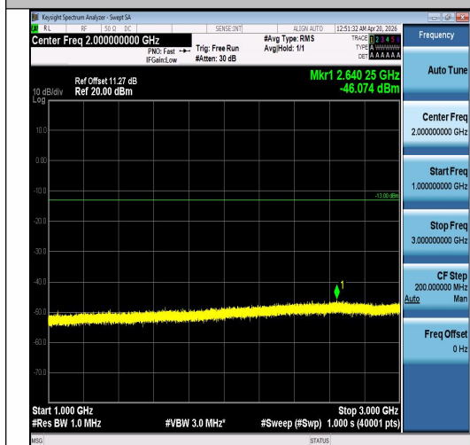
Band5-10MHz-QPSK-20450-1RB#49-1000~300 0-PASS
