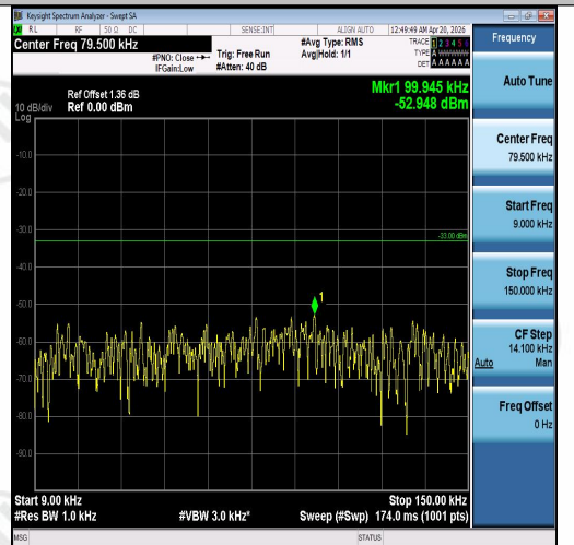
Band5-10MHz-16QAM-20450-1RB#0-0.009~0.1 5-PASS
