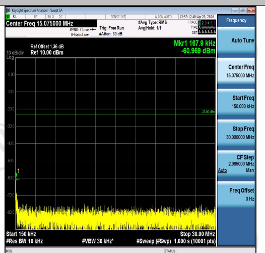
Band5-10MHz-QPSK-20450-50RB#0-0.15~30-P ASS
