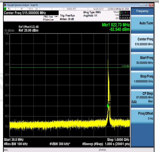
Band5-10MHz-16QAM-20450-1RB#0-30~1000-P ASS
