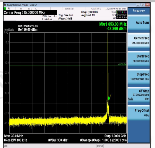
Band5-5MHz-16QAM-20625-1RB#0-30~1000-P ASS
