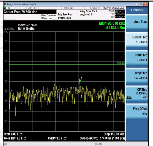
Band5-5MHz-16QAM-20625-1RB#0-0.009~0.15- PASS
