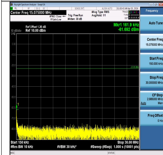
Band5-10MHz-16QAM-20525-50RB#0-0.15~30-PASS
