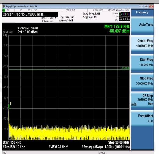
Band5-10MHz-QPSK-20525-50RB#0-0.15~30-P ASS
