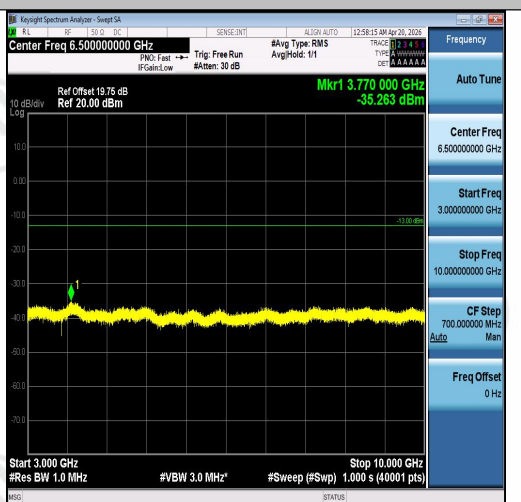
Band5-10MHz-QPSK-20525-1RB#49-3000~100 00-PASS
