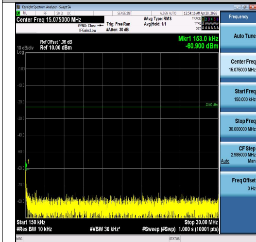
Band5-10MHz-16QAM-20450-50RB#0-0.15~30-PASS
