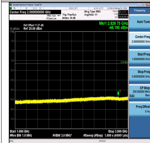
Band5-10MHz-16QAM-20450-50RB#0-1000~3000-PASS
