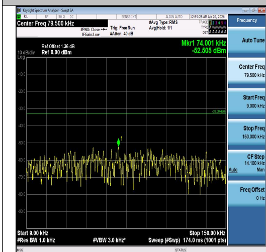
Band5-10MHz-QPSK-20525-50RB#0-0.009~0.1 5-PASS
