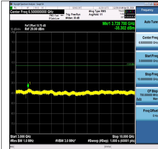
Band5-10MHz-16QAM-20525-1RB#49-3000~10000-PASS
