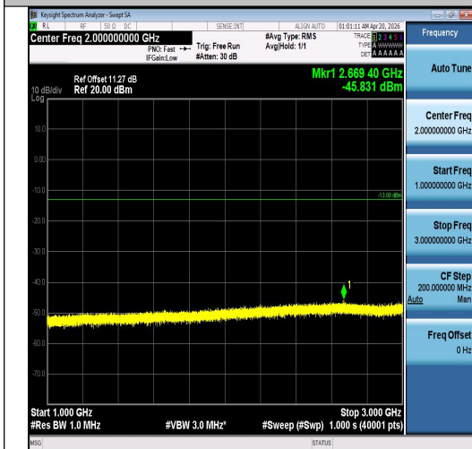
Band5-10MHz-16QAM-20525-50RB#0-1000~3000-PASS
