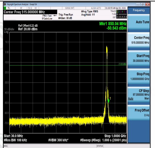
Band5-10MHz-16QAM-20525-50RB#0-30~1000-PASS
