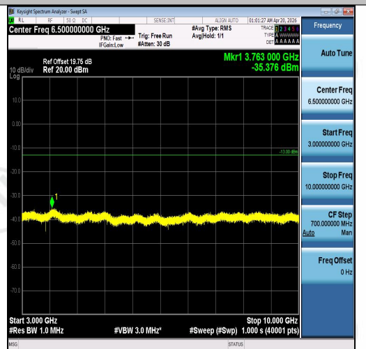
Band5-10MHz-16QAM-20525-50RB#0-3000~10000-PASS
