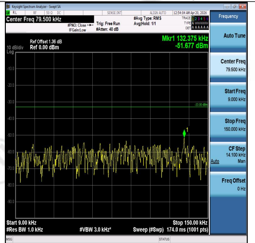
Band5-10MHz-16QAM-20450-50RB#0-0.009~0.15-PASS
