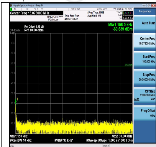
Band5-10MHz-QPSK-20525-1RB#49-0.15~30-P ASS
