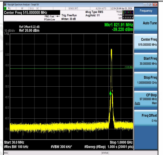
Band5-10MHz-16QAM-20450-50RB#0-30~1000-PASS
