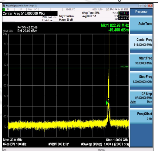
Band5-10MHz-QPSK-20525-1RB#49-30~1000-P ASS
