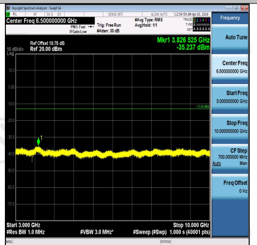
Band5-10MHz-16QAM-20450-50RB#0-3000~10000-PASS
