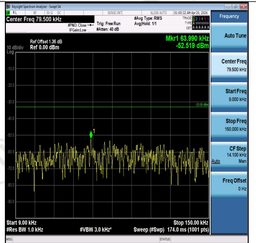
Band5-10MHz-16QAM-20525-50RB#0-0.009~0.15-PASS
