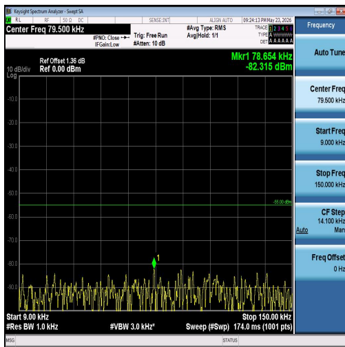
Band7-20MHz-QPSK-21100-100RB#0-0.009~0.15-PASS
