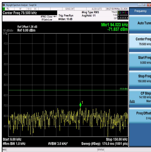
Band7-20MHz-QPSK-21350-1RB#0-0.009~0.15-PASS
