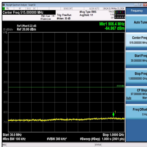
Band7-20MHz-QPSK-21100-100RB#0-30~1000-PASS
