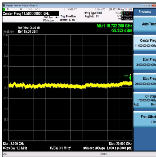
Band7-20MHz-16QAM-21100-100RB#0-3000~20000-PASS
