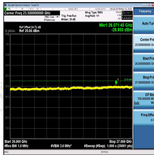
Band7-20MHz-16QAM-21100-100RB#0-20000~27000-PASS
