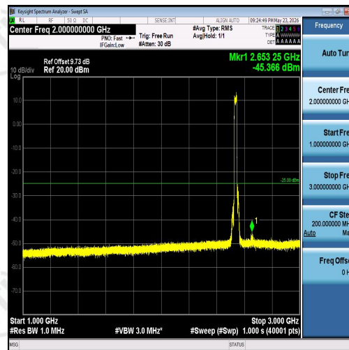
Band7-20MHz-QPSK-21100-100RB#0-1000~3000-PASS
