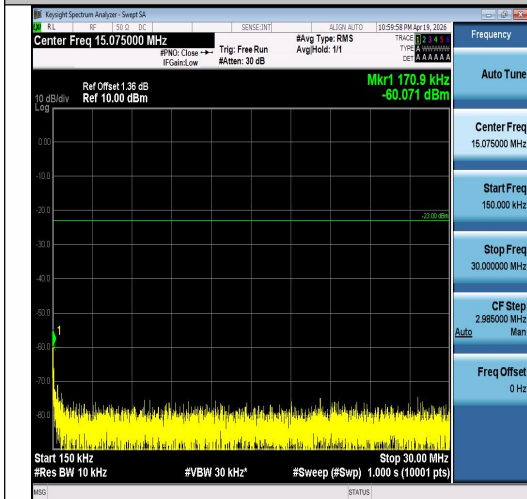
Band5-1.4MHz-16QAM-20525-6RB#0-0.15~30-P ASS
