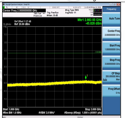
Band5-1.4MHz-QPSK-20643-6RB#0-1000~3000 -PASS
