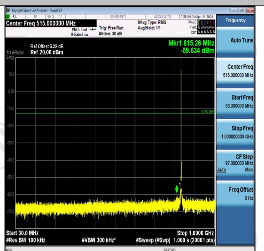
Band5-1.4MHz-16QAM-20525-1RB#0-30~1000-P PASS
