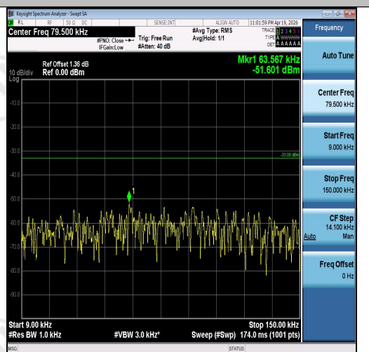
Band5-1.4MHz-16QAM-20643-1RB#0-0.009~0.1 5-PASS
