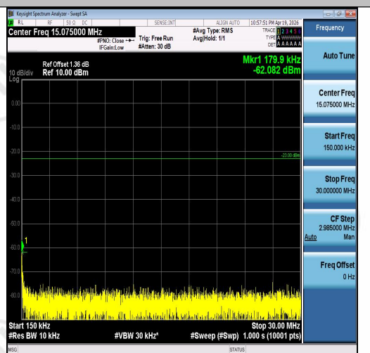
Band5-1.4MHz-16QAM-20525-1RB#5-0.15~30-P ASS
