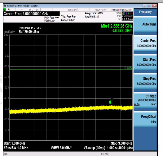
Band5-1.4MHz-16QAM-20525-1RB#5-1000~300 0-PASS
