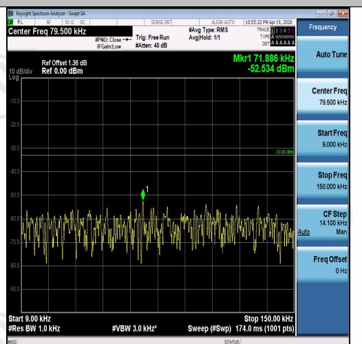
Band5-1.4MHz-16QAM-20525-1RB#0-0.009~0.1 5-PASS
