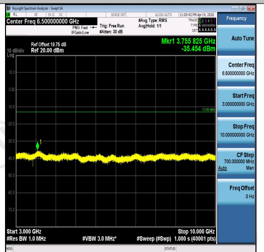
Band5-1.4MHz-16QAM-20525-6RB#0-3000~100 00-PASS
