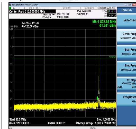
Band5-1.4MHz-QPSK-20525-6RB#0-30~1000-P ASS
