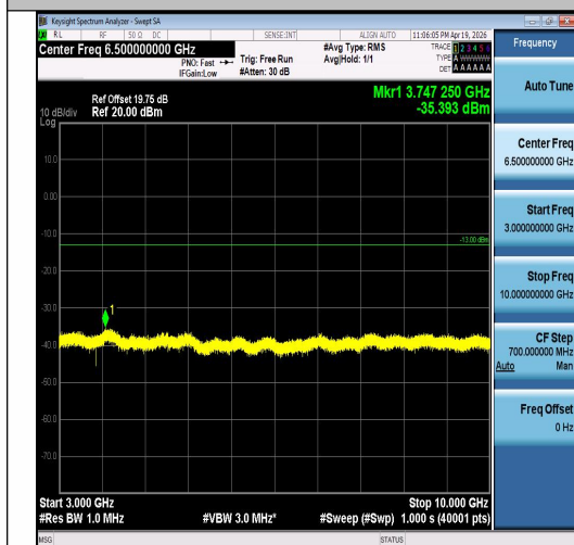
Band5-1.4MHz-QPSK-20643-6RB#0-3000~1000 0-PASS
