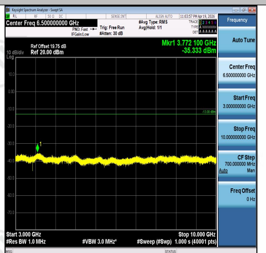
Band5-1.4MHz-QPSK-20643-1RB#5-3000~1000 0-PASS
