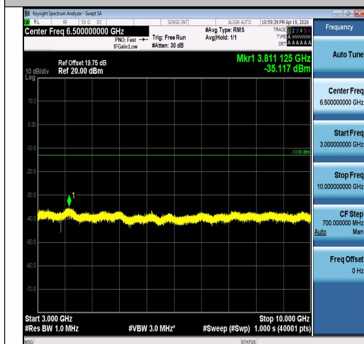
Band5-1.4MHz-QPSK-20525-6RB#0-3000~1000 0-PASS
