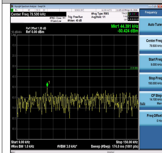
Band5-1.4MHz-QPSK-20643-6RB#0-0.009~0.15 -PASS
