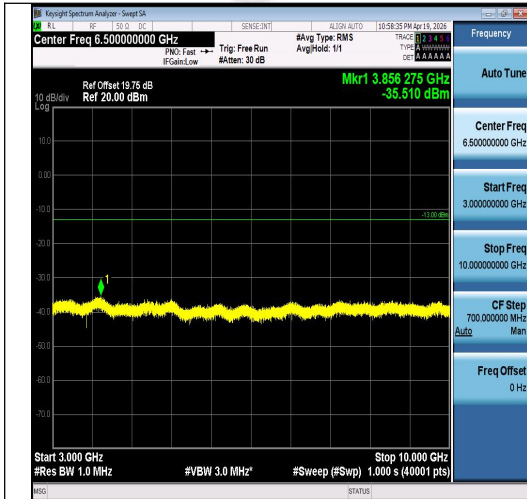
Band5-1.4MHz-16QAM-20525-1RB#5-3000~100 00-PASS
