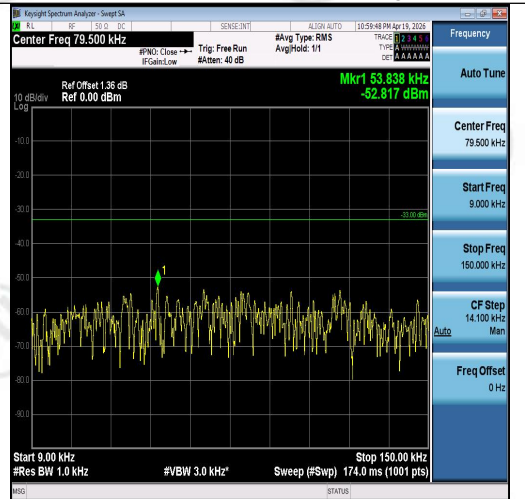
Band5-1.4MHz-16QAM-20525-6RB#0-0.009~0.1 5-PASS
