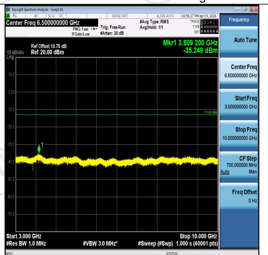
Band5-1.4MHz-16QAM-20525-1RB#0-3000~100 00-PASS
