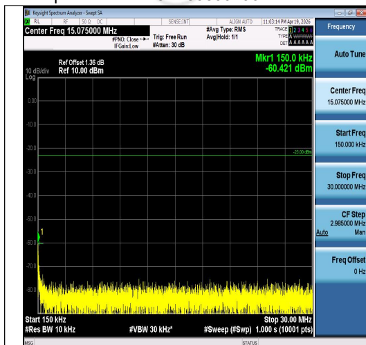
Band5-1.4MHz-QPSK-20643-1RB#5-0.15~30-P ASS
