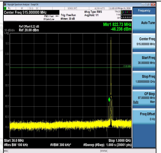
Band5-1.4MHz-16QAM-20525-6RB#0-30~1000- PASS
