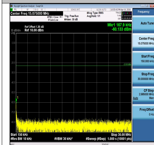
Band5-1.4MHz-16QAM-20525-1RB#0-0.15~30-P ASS
