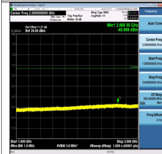
Band5-1.4MHz-16QAM-20525-6RB#0-1000~300 0-PASS
