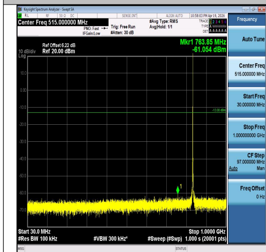
Band5-1.4MHz-16QAM-20525-1RB#5-30~1000- PASS
