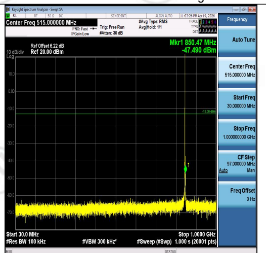
Band5-1.4MHz-QPSK-20643-1RB#5-30~1000-P ASS
