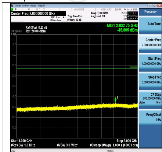
Band5-1.4MHz-16QAM-20525-1RB#0-1000~300 0-PASS
