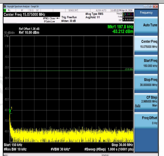
Band5-1.4MHz-QPSK-20643-6RB#0-0.15~30-P ASS
