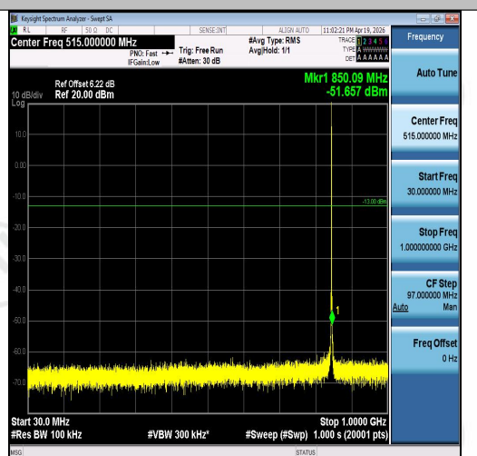
Band5-1.4MHz-16QAM-20643-1RB#0-30~1000-P PASS
