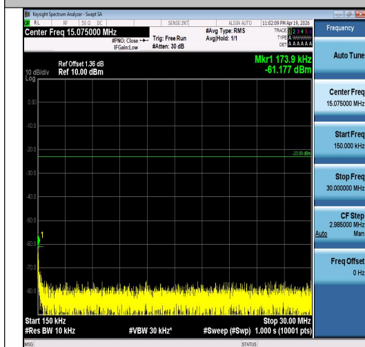
Band5-1.4MHz-16QAM-20643-1RB#0-0.15~30-P ASS
