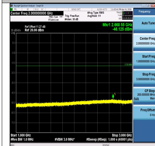
Band5-1.4MHz-QPSK-20643-1RB#5-1000~3000 -PASS
