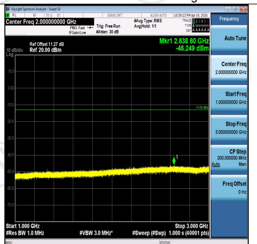
Band5-1.4MHz-QPSK-20525-6RB#0-1000~3000 -PASS
