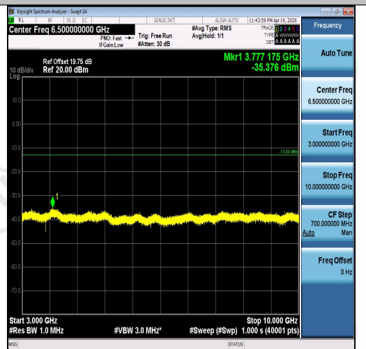
Band5-3MHz-16QAM-20415-15RB#0-3000~100 00-PASS
