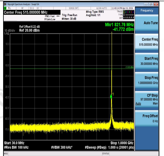
Band5-3MHz-QPSK-20415-1RB#14-30~1000-P ASS
