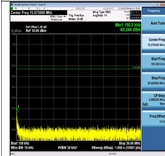
Band5-1.4MHz-16QAM-20643-6RB#0-0.15~30-P ASS
