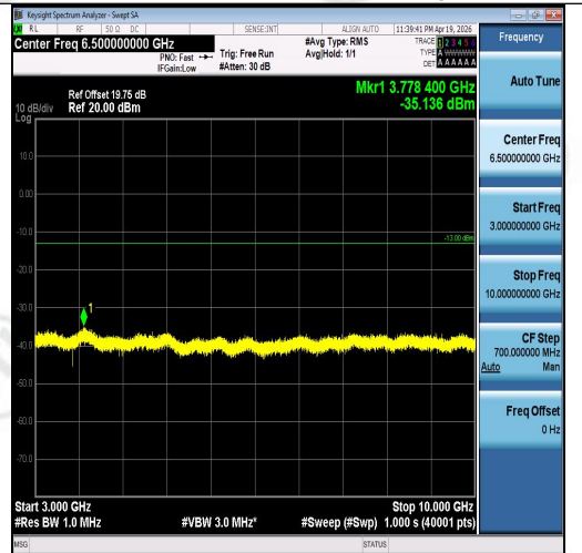
Band5-3MHz-16QAM-20415-1RB#0-3000~1000 0-PASS
