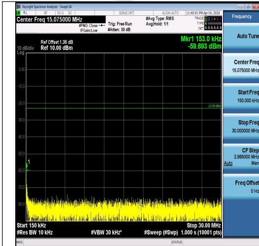
Band5-3MHz-QPSK-20415-1RB#14-0.15~30-PA SS
