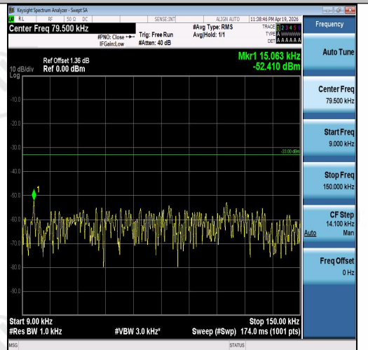
Band5-3MHz-16QAM-20415-1RB#0-0.009~0.15- PASS
