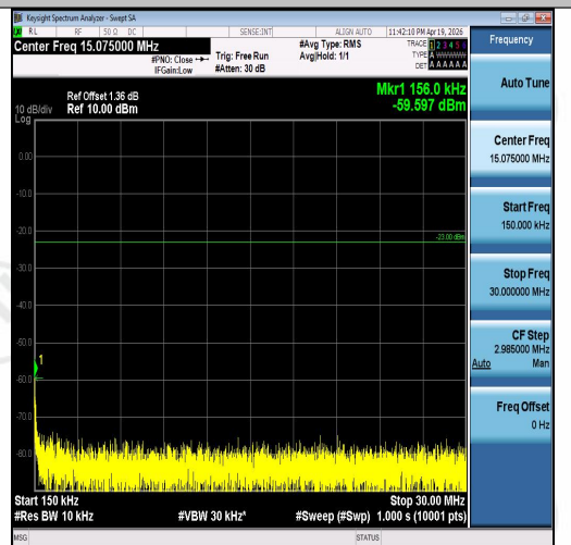
Band5-3MHz-QPSK-20415-15RB#0-0.15~30-PA SS
