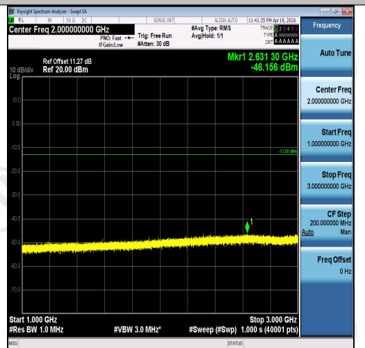
Band5-3MHz-16QAM-20415-1RB#14-1000~300 0-PASS
