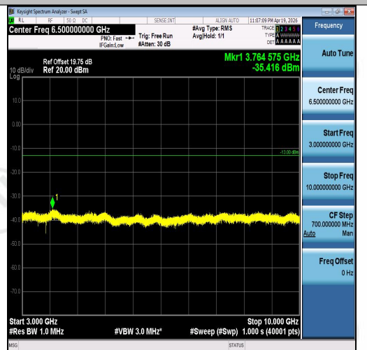
Band5-1.4MHz-16QAM-20643-6RB#0-3000~100 00-PASS
