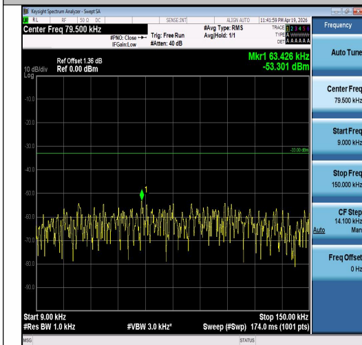
Band5-3MHz-QPSK-20415-15RB#0-0.009~0.15- PASS
