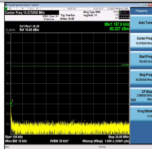
Band5-3MHz-16QAM-20415-1RB#0-0.15~30-PA SS
