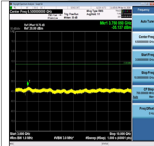
Band5-1.4MHz-16QAM-20643-1RB#5-3000~100 00-PASS
