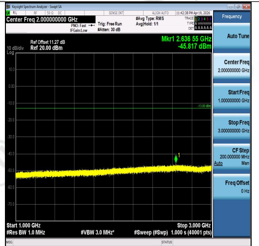
Band5-3MHz-QPSK-20415-15RB#0-1000~3000- PASS
