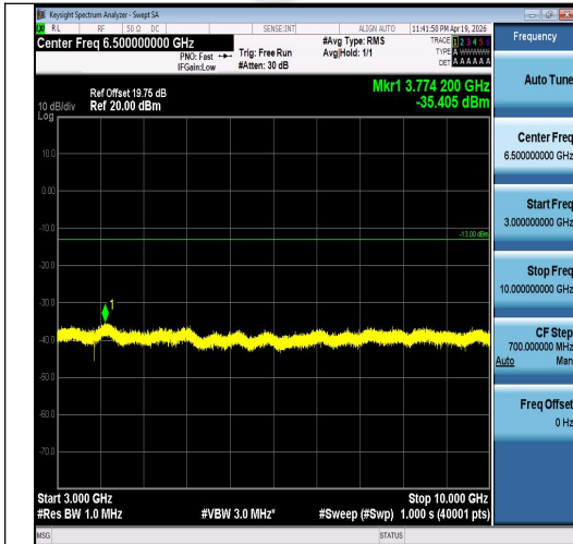
Band5-3MHz-16QAM-20415-1RB#14-3000~100 00-PASS
