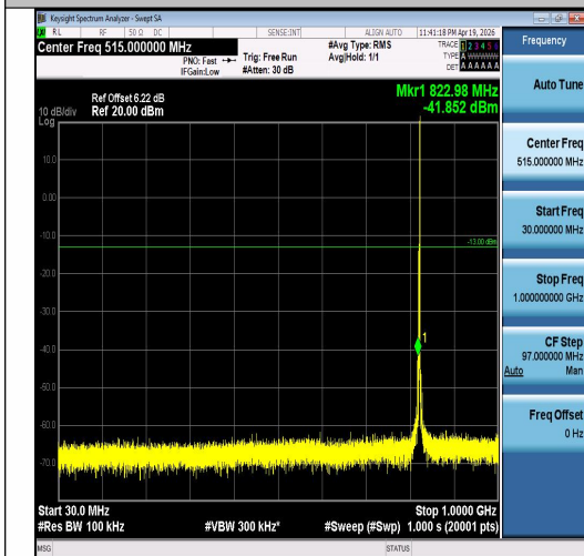
Band5-3MHz-16QAM-20415-1RB#14-30~1000-P ASS
