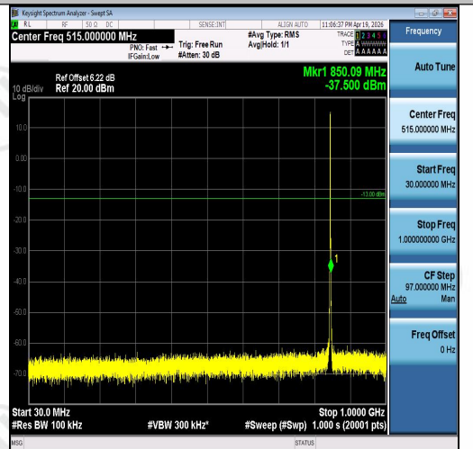
Band5-1.4MHz-16QAM-20643-6RB#0-30~1000- PASS
