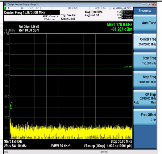
Band5-3MHz-16QAM-20415-1RB#14-0.15~30-P ASS
