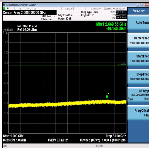
Band5-3MHz-16QAM-20415-15RB#0-1000~300 0-PASS
