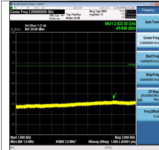
Band5-3MHz-16QAM-20415-1RB#0-1000~3000- PASS
