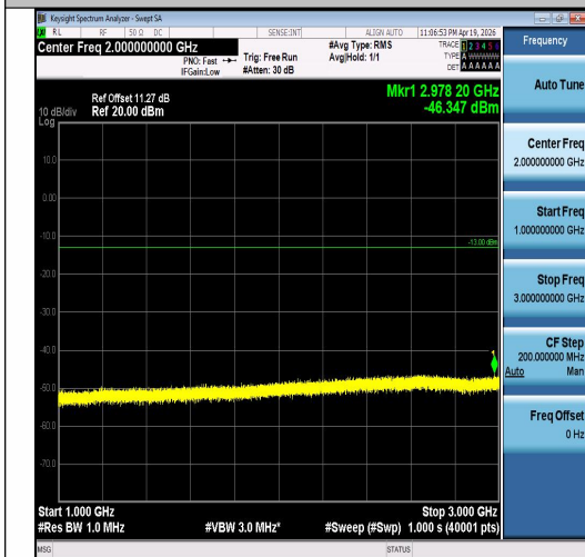
Band5-1.4MHz-16QAM-20643-6RB#0-1000~300 0-PASS
