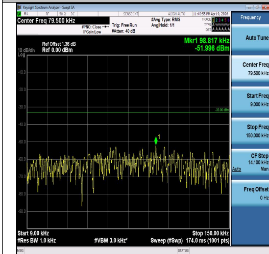
Band5-3MHz-16QAM-20415-1RB#14-0.009~0.1 5-PASS
