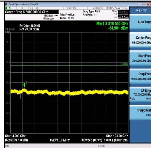
Band5-3MHz-QPSK-20415-15RB#0-3000~1000 0-PASS
