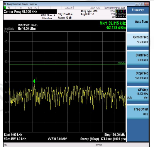
Band5-1.4MHz-16QAM-20643-6RB#0-0.009~0.1 5-PASS
