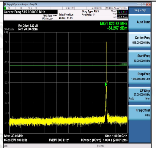
Band5-3MHz-16QAM-20415-15RB#0-30~1000-P ASS
