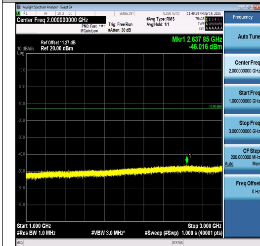
Band5-3MHz-QPSK-20415-1RB#14-1000~3000- PASS
