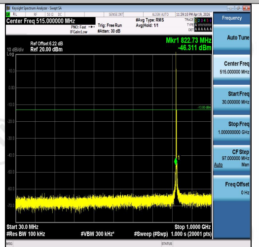
Band5-3MHz-16QAM-20415-1RB#0-30~1000-P ASS
