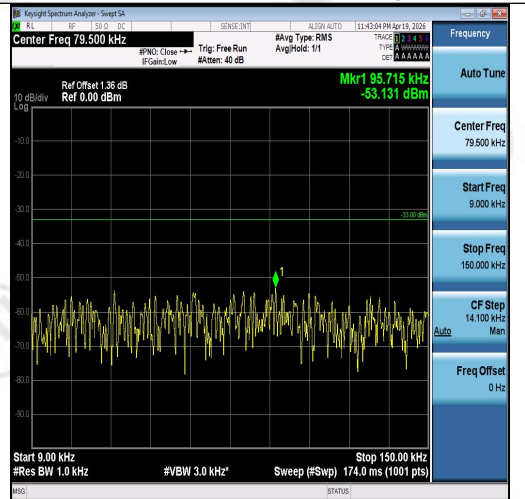
Band5-3MHz-16QAM-20415-15RB#0-0.009~0.1 5-PASS
