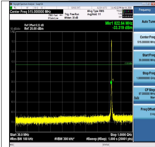
Band5-3MHz-QPSK-20415-15RB#0-30~1000-P ASS
