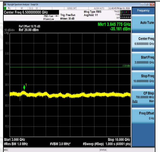
Band5-3MHz-QPSK-20415-1RB#14-3000~10000- PASS
