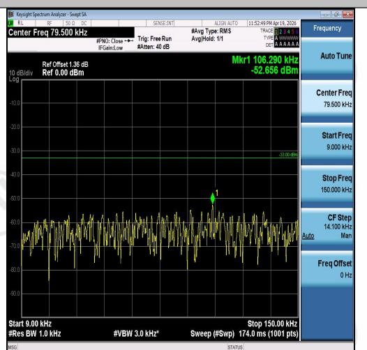
Band5-3MHz-QPSK-20635-1RB#14-0.009~0.15- PASS
