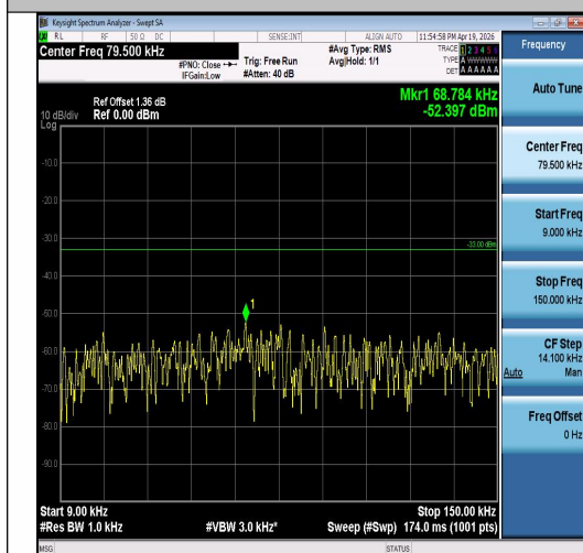
Band5-3MHz-QPSK-20635-15RB#0-0.009~0.15- PASS
