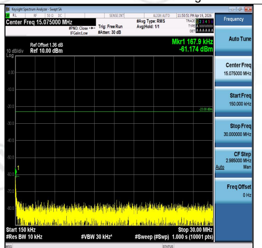
Band5-3MHz-QPSK-20635-1RB#0-0.15~30-PAS S
