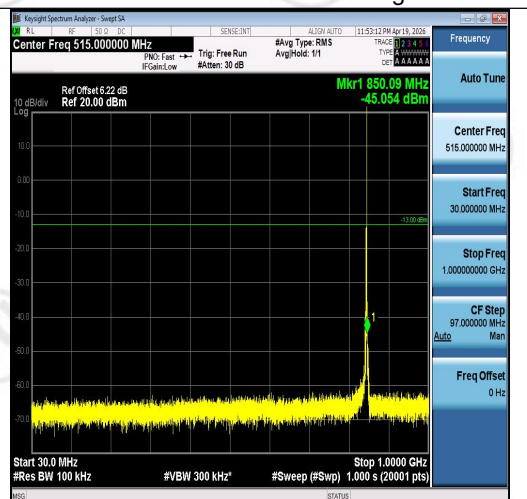
Band5-3MHz-QPSK-20635-1RB#14-30~1000-P ASS
