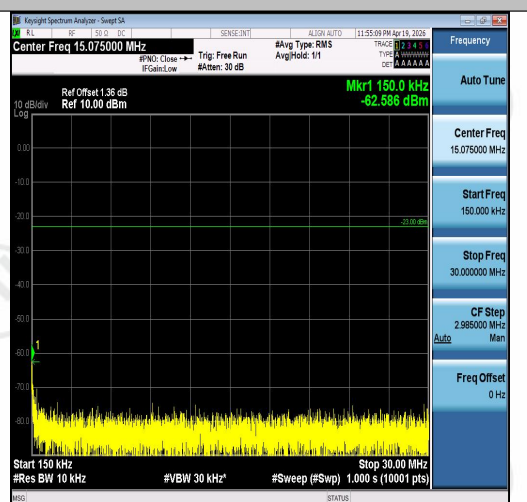
Band5-3MHz-QPSK-20635-15RB#0-0.15~30-PA SS
