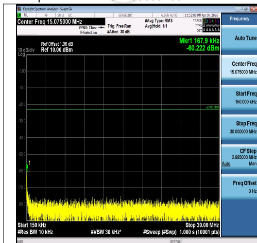
Band5-3MHz-QPSK-20635-1RB#14-0.15~30-PA SS
