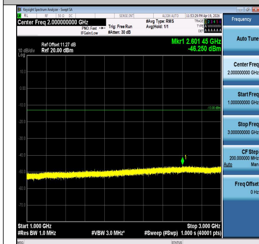
Band5-3MHz-QPSK-20635-1RB#14-1000~3000- PASS
