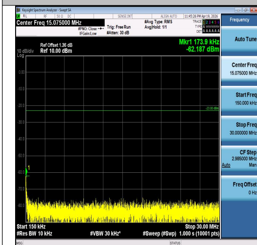
Band5-3MHz-16QAM-20525-1RB#0-0.15~30-PA SS
