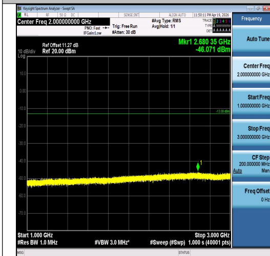
Band5-3MHz-16QAM-20525-15RB#0-1000~300 0-PASS
