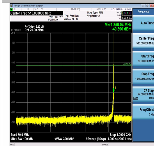
Band5-3MHz-QPSK-20635-1RB#0-30~1000-PA SS
