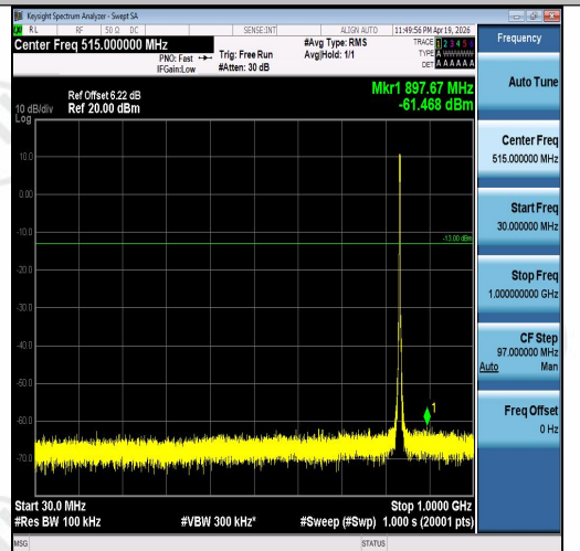
Band5-3MHz-16QAM-20525-15RB#0-30~1000-P ASS
