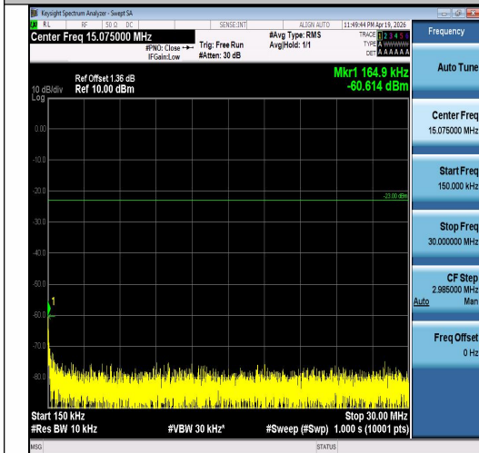
Band5-3MHz-16QAM-20525-15RB#0-0.15~30-P ASS
