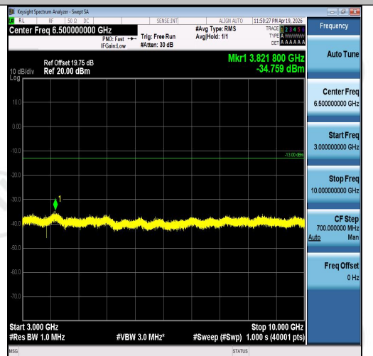
Band5-3MHz-16QAM-20525-15RB#0-3000~100 00-PASS
