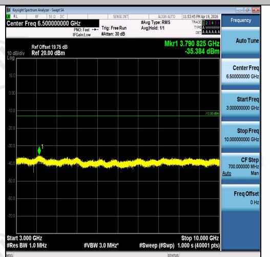
Band5-3MHz-QPSK-20635-1RB#14-3000~10000- PASS
