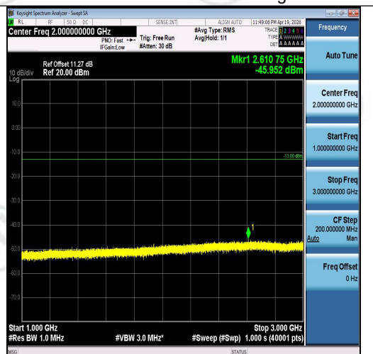
Band5-3MHz-QPSK-20525-15RB#0-1000~3000- PASS
