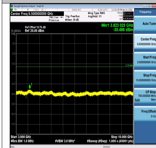
Band5-3MHz-QPSK-20635-1RB#0-3000~10000- PASS
