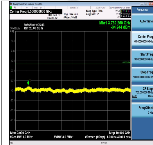
Band5-3MHz-16QAM-20525-1RB#14-3000~100 00-PASS
