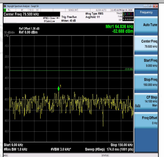
Band5-3MHz-16QAM-20525-1RB#0-0.009~0.15- PASS
