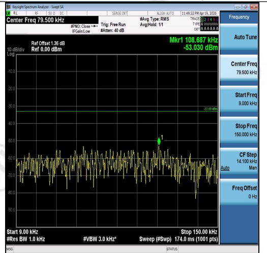
Band5-3MHz-16QAM-20525-15RB#0-0.009~0.1 5-PASS
