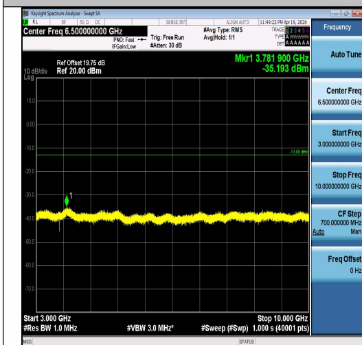
Band5-3MHz-QPSK-20525-15RB#0-3000~1000 0-PASS
