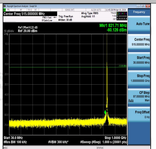
Band5-3MHz-16QAM-20525-1RB#0-30~1000-P ASS
