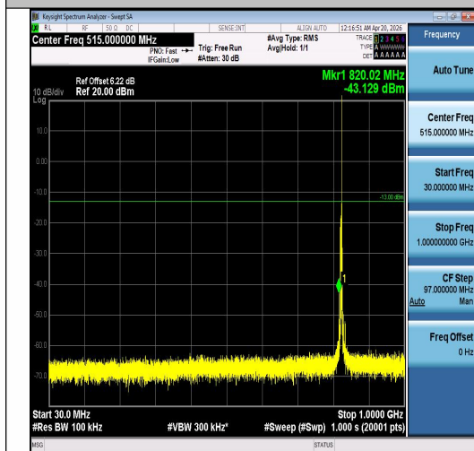
Band5-5MHz-16QAM-20425-1RB#24-30~1000-P ASS
