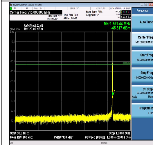
Band5-3MHz-16QAM-20635-1RB#14-30~1000-P ASS
