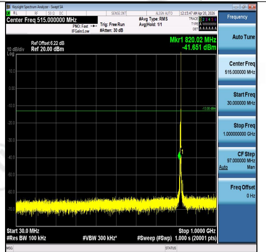
Band5-5MHz-QPSK-20425-1RB#24-30~1000-P ASS
