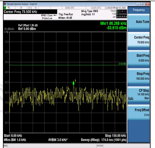
Band5-3MHz-16QAM-20635-15RB#0-0.009~0.1 5-PASS
