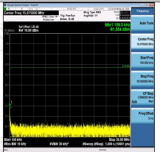
Band5-5MHz-16QAM-20425-1RB#24-0.15~30-P ASS
