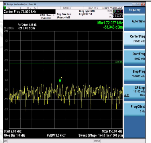
Band5-3MHz-16QAM-20635-1RB#0-0.009~0.15-P PASS
