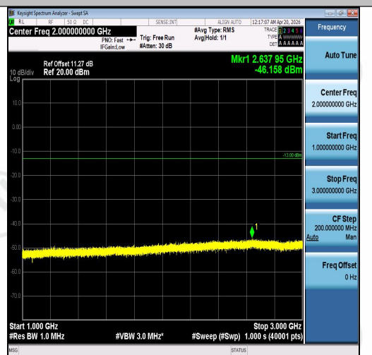
Band5-5MHz-16QAM-20425-1RB#24-1000~300 0-PASS
