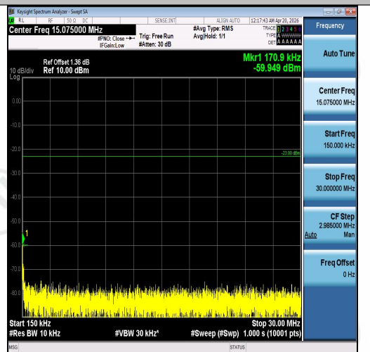
Band5-5MHz-QPSK-20425-25RB#0-0.15~30-PA SS
