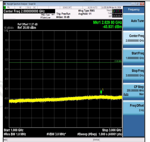
Band5-3MHz-QPSK-20635-15RB#0-1000~3000-P PASS
