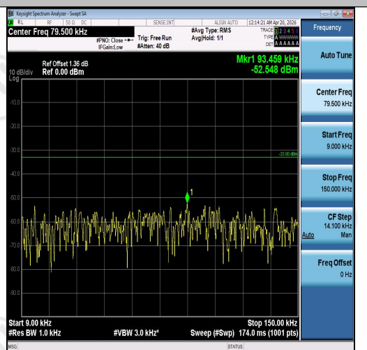
Band5-5MHz-16QAM-20425-1RB#0-0.009~0.15- PASS
