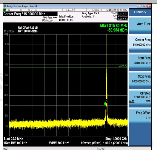
Band5-5MHz-16QAM-20425-1RB#0-30~1000-P ASS
