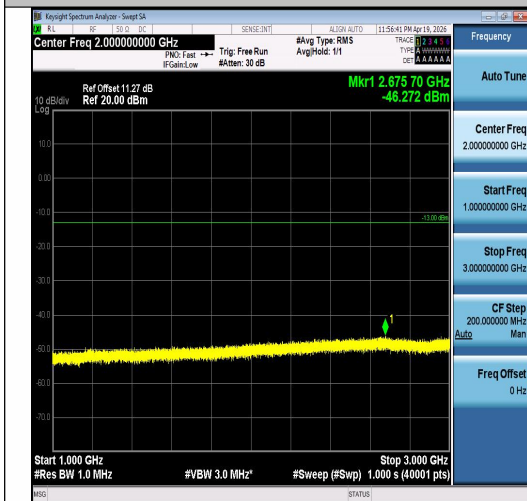
Band5-3MHz-16QAM-20635-15RB#0-1000~300 0-PASS
