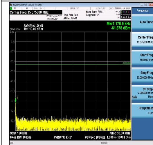
Band5-3MHz-16QAM-20635-1RB#0-0.15~30-PA SS
