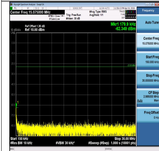
Band5-3MHz-16QAM-20635-15RB#0-0.15~30-P ASS
