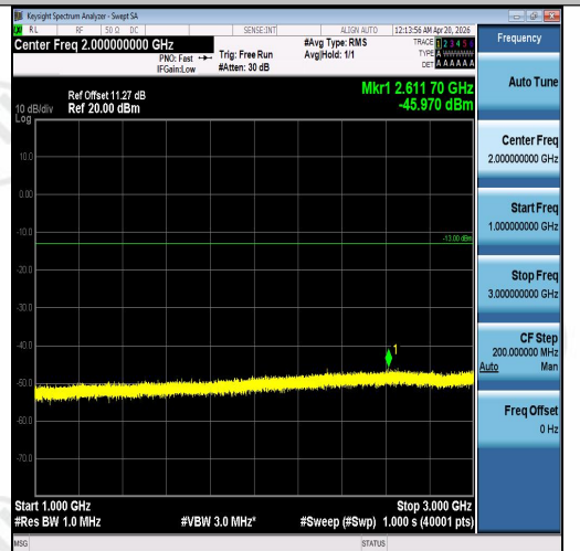
Band5-5MHz-QPSK-20425-1RB#0-1000~3000-P ASS
