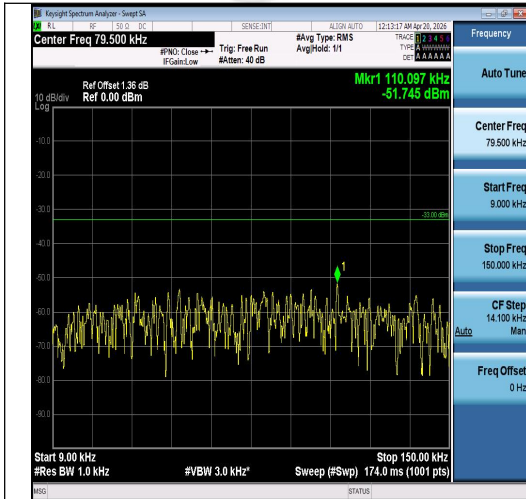
Band5-5MHz-QPSK-20425-1RB#0-0.009~0.15-P ASS
