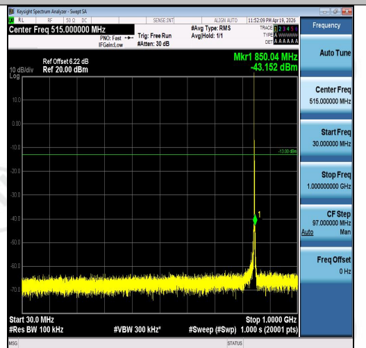
Band5-3MHz-16QAM-20635-1RB#0-30~1000-P ASS
