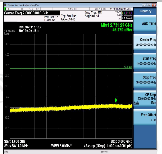
Band5-3MHz-16QAM-20635-1RB#14-1000~300 0-PASS
