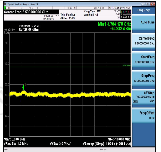
Band5-5MHz-16QAM-20425-1RB#0-3000~1000 0-PASS
