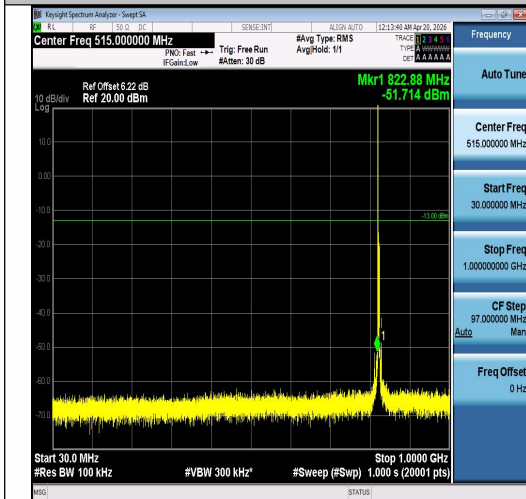
Band5-5MHz-QPSK-20425-1RB#0-30~1000-PA SS
