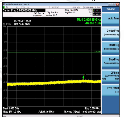
Band5-5MHz-QPSK-20425-25RB#0-1000~3000- PASS
