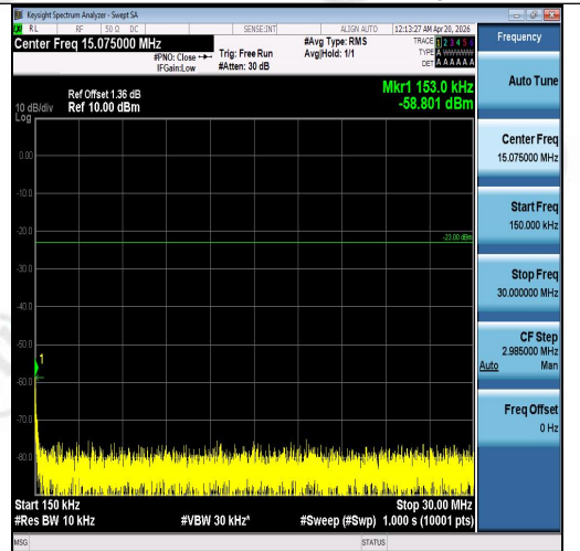
Band5-5MHz-QPSK-20425-1RB#0-0.15~30-PAS S
