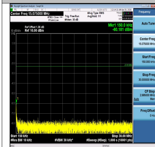
Band5-5MHz-16QAM-20425-1RB#0-0.15~30-PA SS
