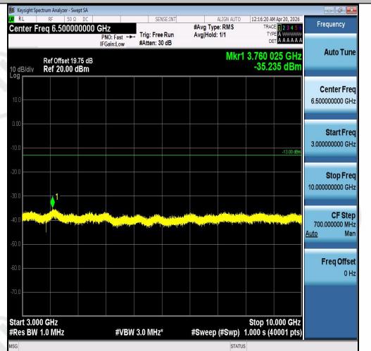
Band5-5MHz-QPSK-20425-1RB#24-3000~10000- PASS
