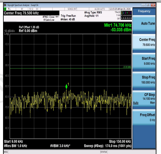
Band5-5MHz-QPSK-20425-1RB#24-0.009~0.15- PASS
