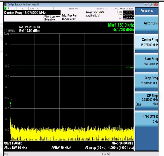
Band5-3MHz-16QAM-20635-1RB#14-0.15~30-P ASS
