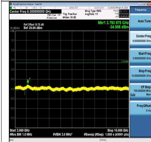
Band5-3MHz-QPSK-20635-15RB#0-3000~1000 0-PASS
