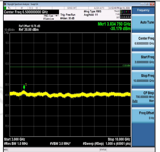
Band5-3MHz-16QAM-20635-1RB#0-3000~1000 0-PASS
