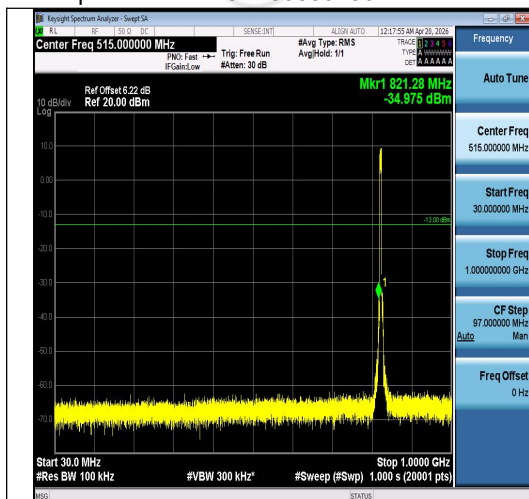
Band5-5MHz-QPSK-20425-25RB#0-30~1000-P ASS
