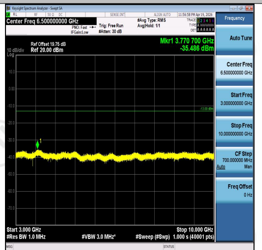
Band5-3MHz-16QAM-20635-15RB#0-3000~100 00-PASS
