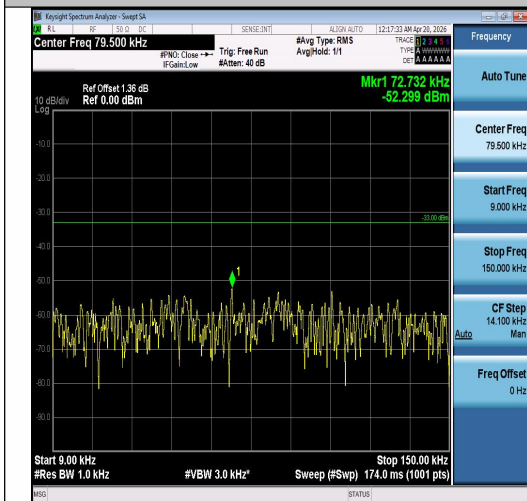
Band5-5MHz-QPSK-20425-25RB#0-0.009~0.15- PASS
