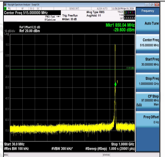
Band5-3MHz-16QAM-20635-15RB#0-30~1000-P ASS
