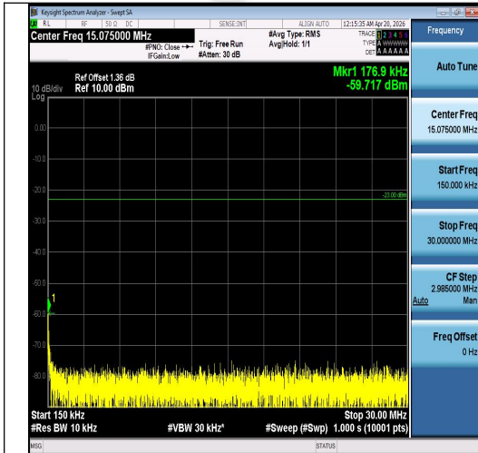
Band5-5MHz-QPSK-20425-1RB#24-0.15~30-PA SS
