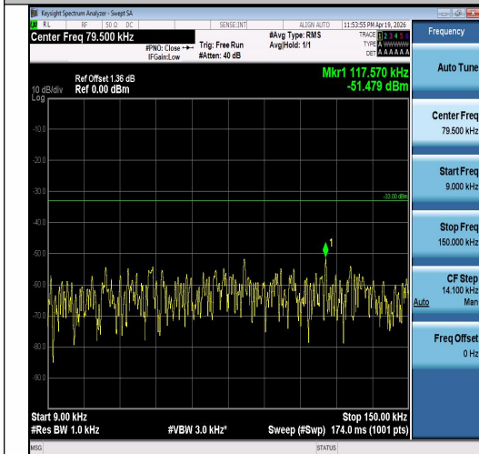
Band5-3MHz-16QAM-20635-1RB#14-0.009~0.1 5-PASS
