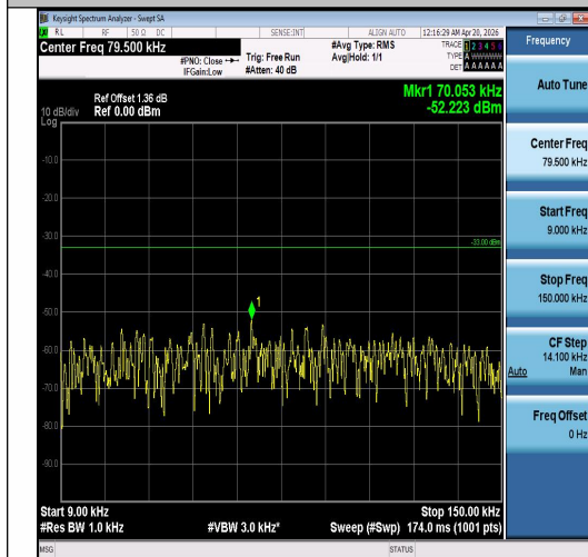
Band5-5MHz-16QAM-20425-1RB#24-0.009~0.1 5-PASS
