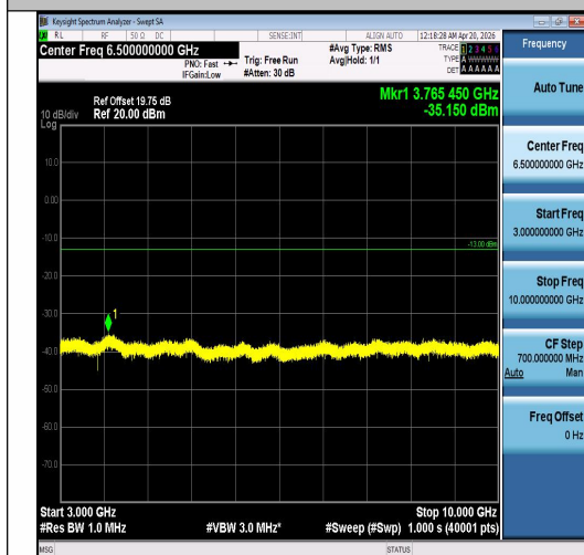
Band5-5MHz-QPSK-20425-25RB#0-3000~1000 0-PASS
