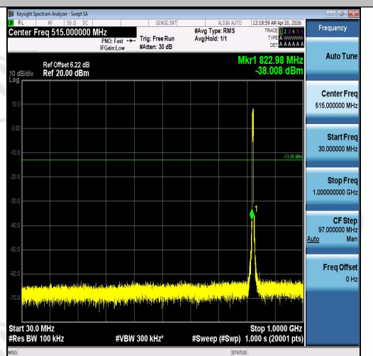
Band5-5MHz-16QAM-20425-25RB#0-30~1000-P ASS
