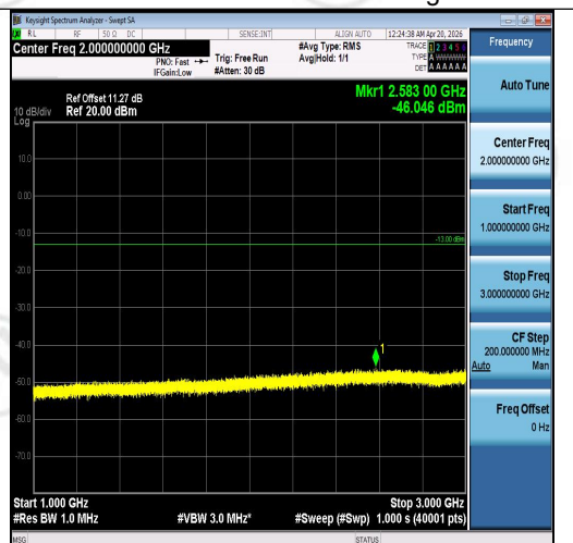
Band5-5MHz-QPSK-20525-25RB#0-1000~3000- PASS
