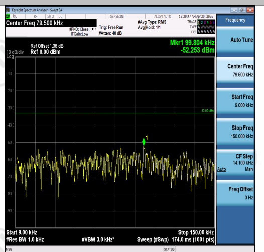
Band5-5MHz-16QAM-20525-1RB#0-0.009~0.15- PASS
