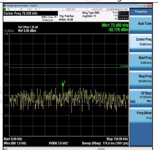
Band5-5MHz-16QAM-20425-25RB#0-0.009~0.1 5-PASS
