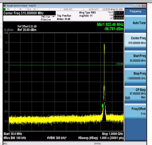
Band5-5MHz-16QAM-20525-25RB#0-30~1000-P ASS
