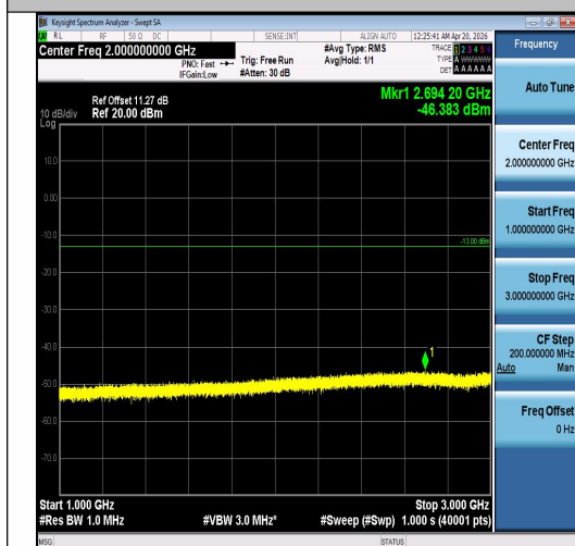
Band5-5MHz-16QAM-20525-25RB#0-1000~300 0-PASS
