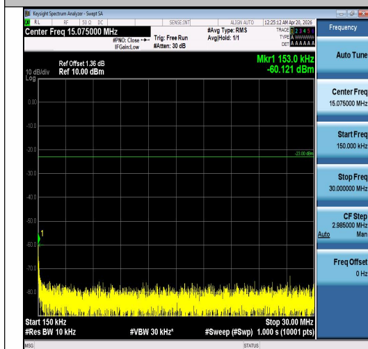
Band5-5MHz-16QAM-20525-25RB#0-0.15~30-P ASS
