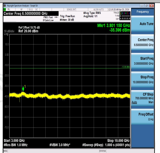
Band5-5MHz-16QAM-20425-25RB#0-3000~100 00-PASS
