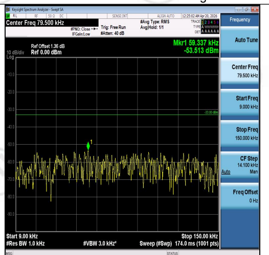
Band5-5MHz-16QAM-20525-25RB#0-0.009~0.1 5-PASS
