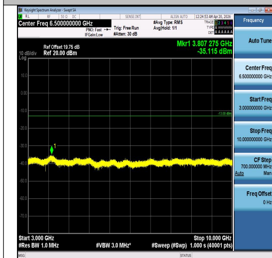
Band5-5MHz-QPSK-20525-25RB#0-3000~1000 0-PASS
