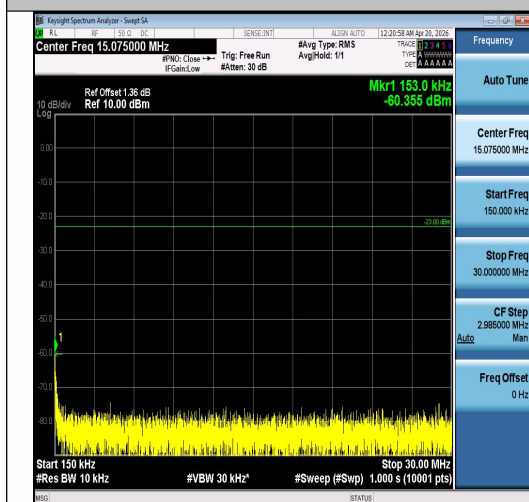
Band5-5MHz-16QAM-20525-1RB#0-0.15~30-PA SS
