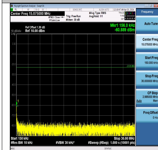
Band5-5MHz-16QAM-20425-25RB#0-0.15~30-P ASS
