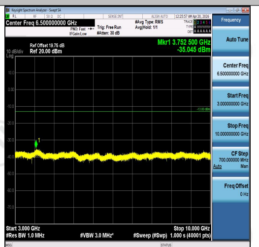
Band5-5MHz-16QAM-20525-25RB#0-3000~100 00-PASS
