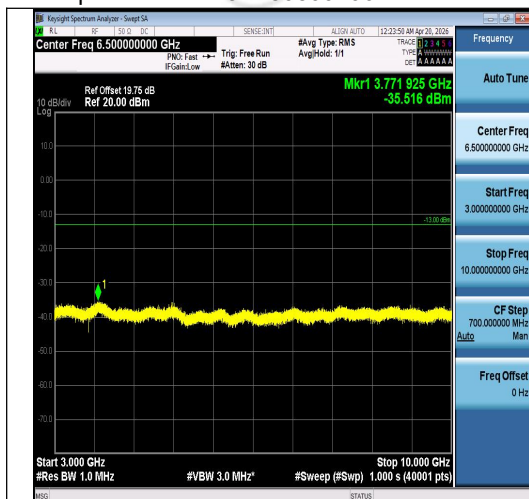
Band5-5MHz-16QAM-20525-1RB#24-3000~100 00-PASS
