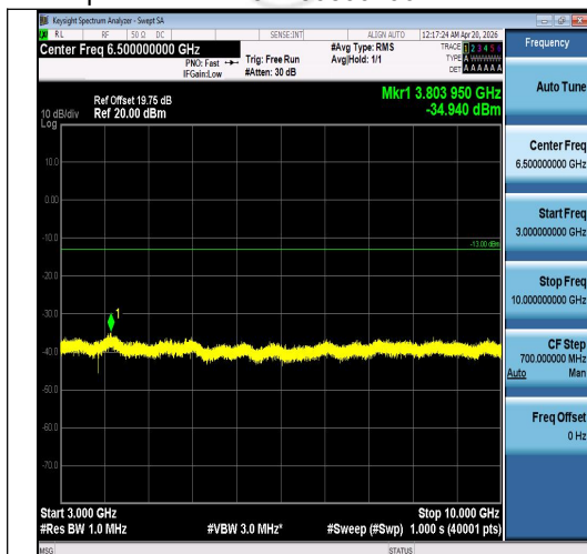
Band5-5MHz-16QAM-20425-1RB#24-3000~100 00-PASS
