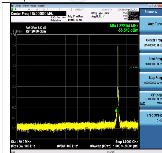
Band5-5MHz-QPSK-20525-25RB#0-30~1000-P ASS
