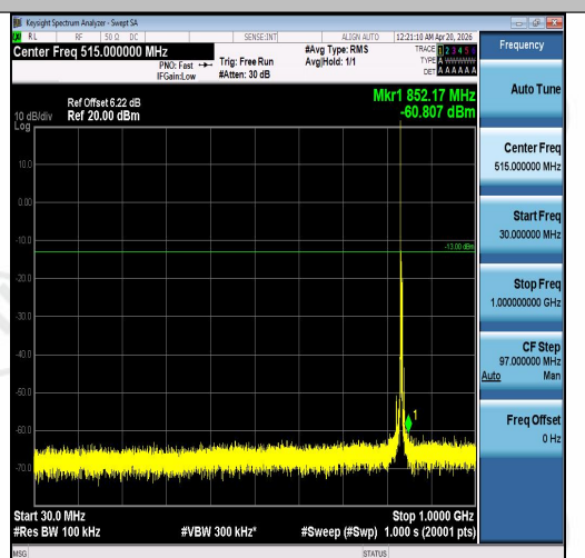
Band5-5MHz-16QAM-20525-1RB#0-30~1000-P ASS
