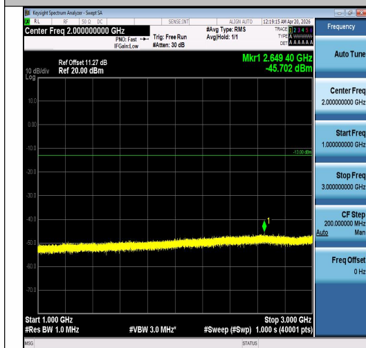
Band5-5MHz-16QAM-20425-25RB#0-1000~300 0-PASS
