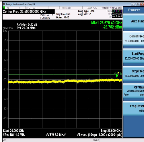
Band7-15MHz-QPSK-20825-75RB#0-20000~27 000-PASS
