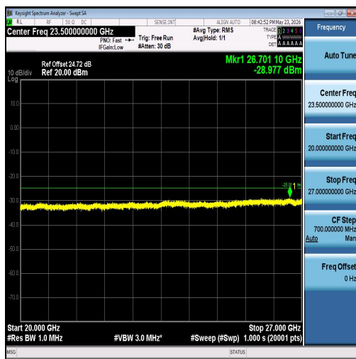
Band7-10MHz-16QAM-21400-50RB#0-20000~27000-PASS
