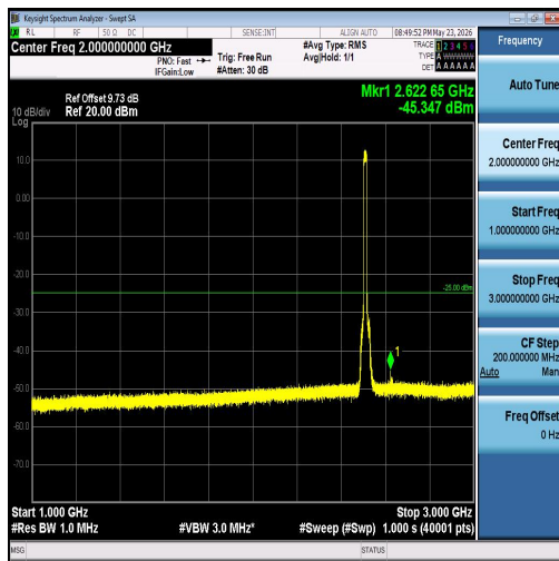
Band7-15MHz-QPSK-20825-75RB#0-1000~300 0-PASS
