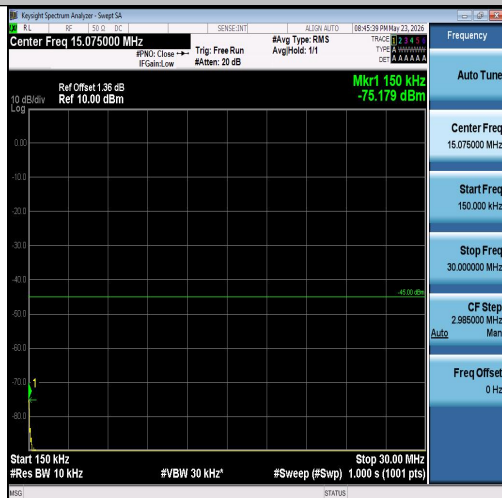
Band7-15MHz-16QAM-20825-1RB#0-0.15~30-P ASS
