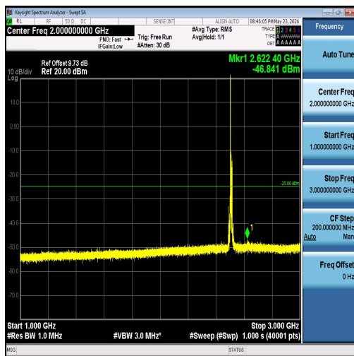
Band7-15MHz-16QAM-20825-1RB#0-1000~300 0-PASS
