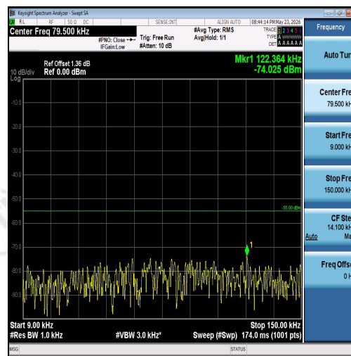
Band7-15MHz-QPSK-20825-1RB#0-0.009~0.15-PASS
