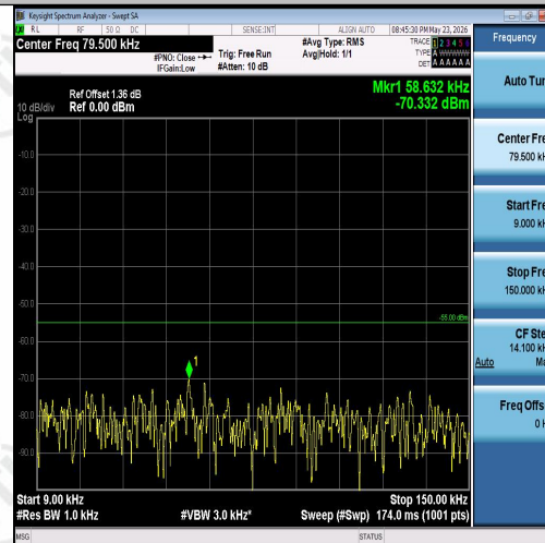
Band7-15MHz-16QAM-20825-1RB#0-0.009~0.1 5-PASS
