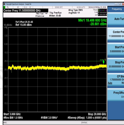
Band7-15MHz-16QAM-20825-1RB#0-3000~200 00-PASS
