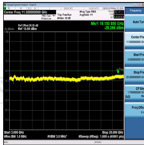
Band7-15MHz-QPSK-20825-75RB#0-3000~200 00-PASS
