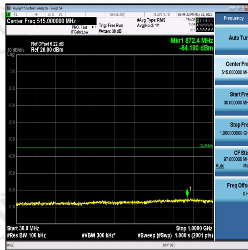
Band7-15MHz-QPSK-20825-1RB#0-30~1000-P ASS
