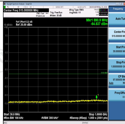
Band7-15MHz-16QAM-20825-1RB#0-30~1000-P ASS
