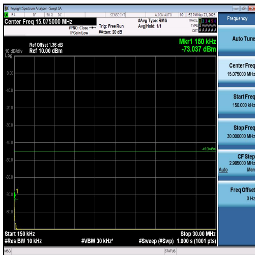
Band7-20MHz-16QAM-20850-1RB#0-0.15~30-P ASS
