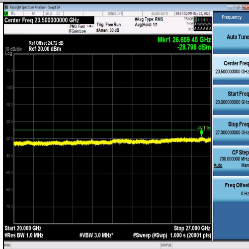
Band7-20MHz-16QAM-20850-100RB#0-20000~ 27000-PASS
