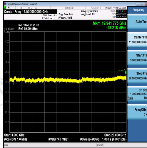
Band7-20MHz-QPSK-21100-1RB#0-3000~2000 0-PASS
