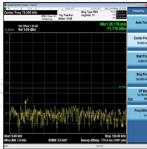
Band7-20MHz-16QAM-20850-1RB#0-0.009~0.1 5-PASS
