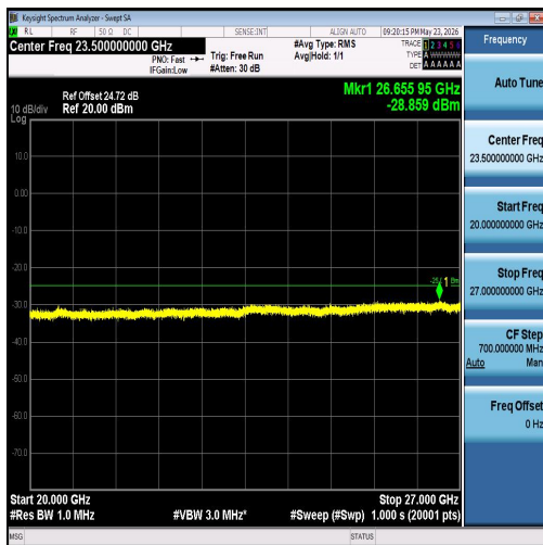
Band7-20MHz-QPSK-21100-1RB#0-20000~270 00-PASS
