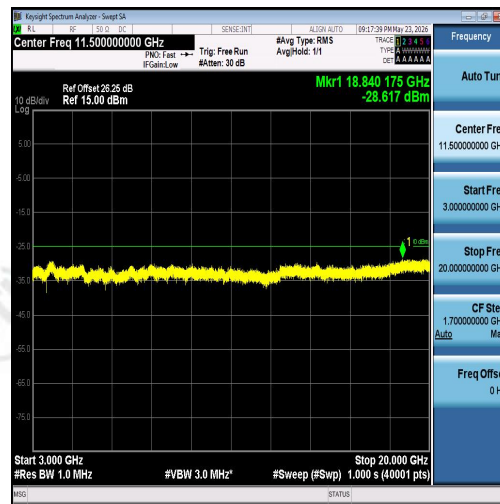
Band7-20MHz-16QAM-20850-100RB#0-3000~2 0000-PASS
