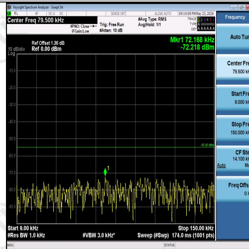
Band7-20MHz-QPSK-21100-1RB#0-0.009~0.15- PASS
