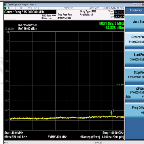
Band7-20MHz-QPSK-21100-1RB#0-30~1000-PA SS
