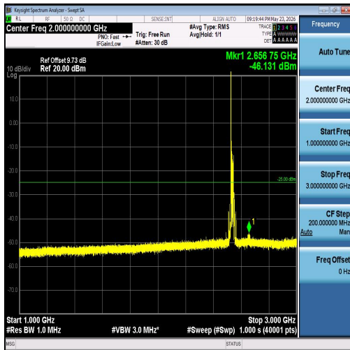
Band7-20MHz-QPSK-21100-1RB#0-1000~3000- PASS
