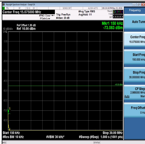
Band7-20MHz-QPSK-21100-1RB#0-0.15~30-PA SS
