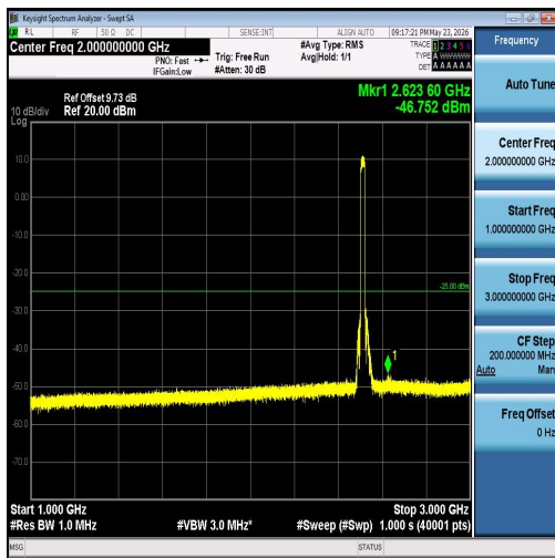
Band7-20MHz-16QAM-20850-100RB#0-1000~3 000-PASS
