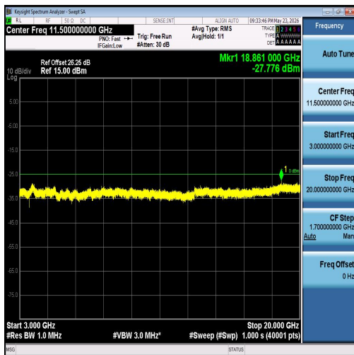
Band7-20MHz-QPSK-21350-100RB#0-3000~20000-PASS
