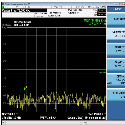
Band7-20MHz-16QAM-21350-100RB#0-0.009~0.15-PASS
