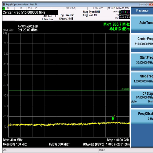
Band7-20MHz-QPSK-21350-100RB#0-30~1000-PASS
