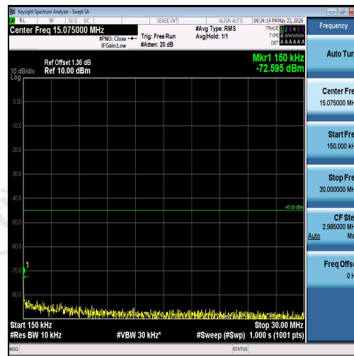
Band7-20MHz-16QAM-21350-100RB#0-0.15~30-PASS
