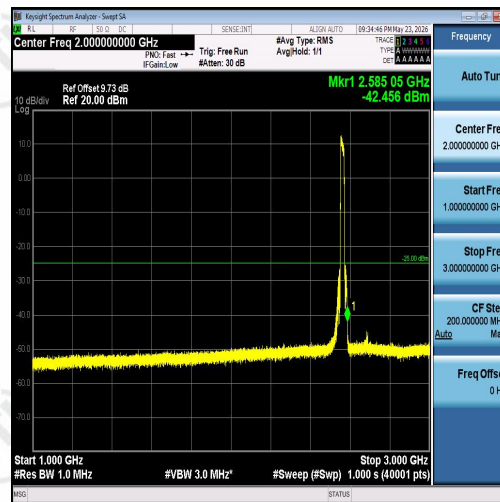
Band7-20MHz-16QAM-21350-100RB#0-1000~3000-PASS
