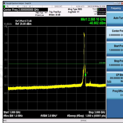
Band7-20MHz-QPSK-21350-100RB#0-1000~3000-PASS
