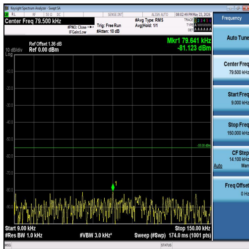
Band7-5MHz-16QAM-21100-25RB#0-0.009~0.1 5-PASS
