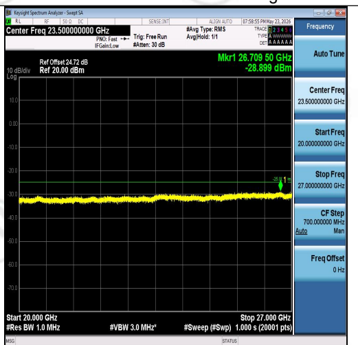
Band7-5MHz-16QAM-21100-1RB#0-20000~270 00-PASS
