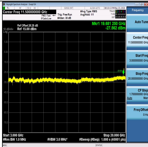
Band7-5MHz-QPSK-21425-1RB#24-3000~2000 0-PASS
