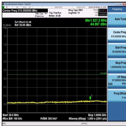
Band7-5MHz-QPSK-21425-1RB#24-30~1000-P ASS
