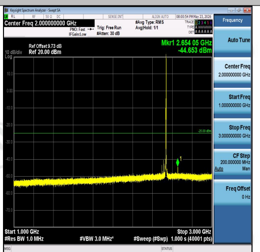
Band7-5MHz-16QAM-21100-1RB#24-1000~300 0-PASS
