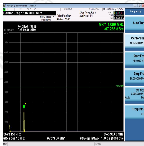
Band7-5MHz-16QAM-21425-1RB#0-0.15~30-PA
