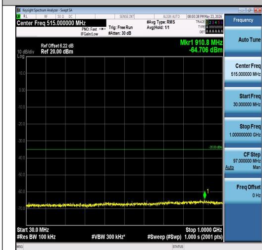
Band7-5MHz-16QAM-21100-1RB#24-30~1000-P ASS
