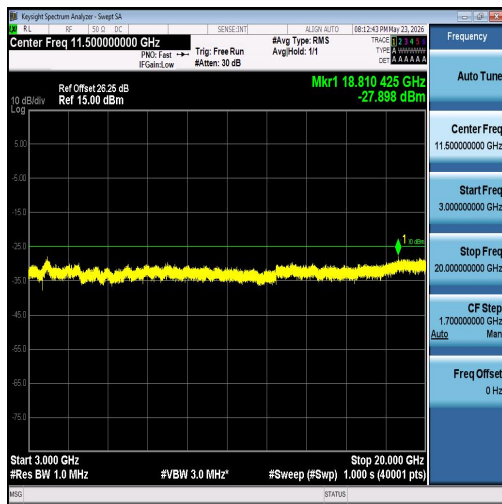
Band7-5MHz-QPSK-21425-25RB#0-3000~2000 0-PASS
