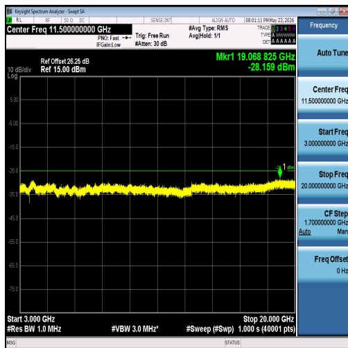
Band7-5MHz-16QAM-21100-1RB#24-3000~200 00-PASS
