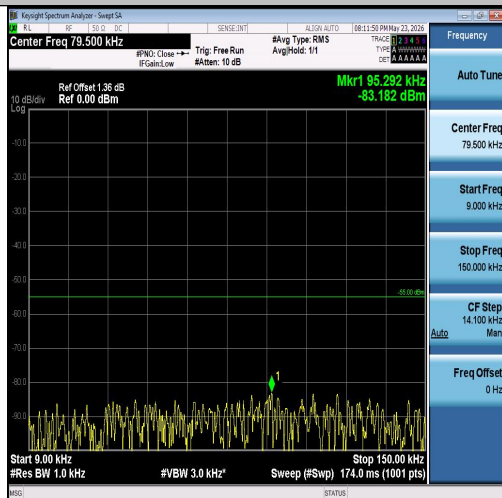
Band7-5MHz-QPSK-21425-25RB#0-0.009~0.15- PASS
