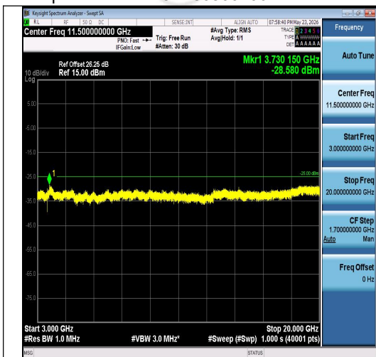
Band7-5MHz-16QAM-21100-1RB#0-3000~2000 0-PASS
