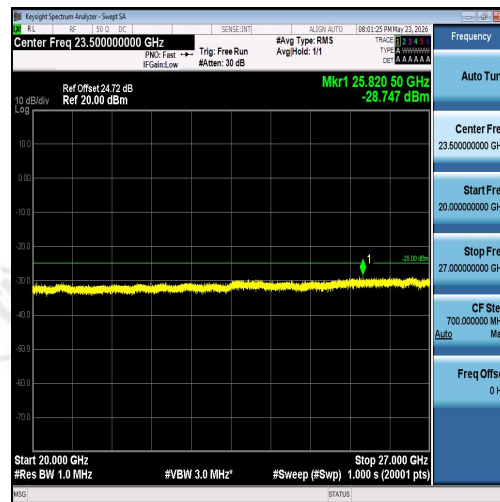
Band7-5MHz-16QAM-21100-1RB#24-20000~27 000-PASS
