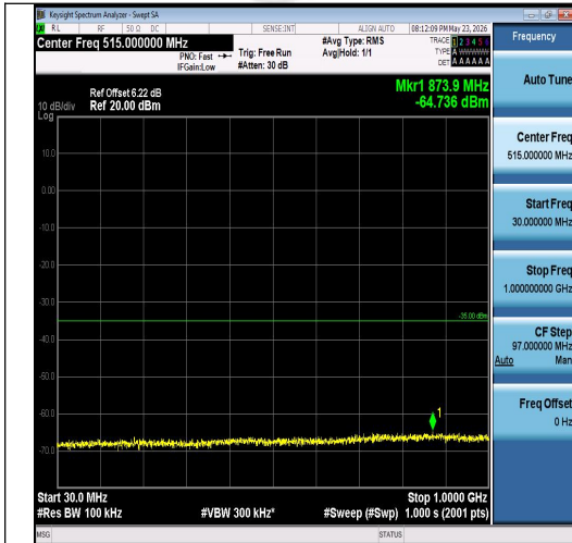
Band7-5MHz-QPSK-21425-25RB#0-30~1000-P ASS
