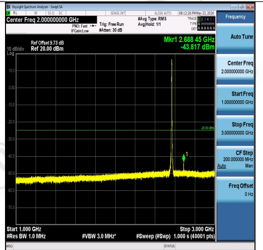
Band7-5MHz-QPSK-21425-25RB#0-1000~3000-P PASS
