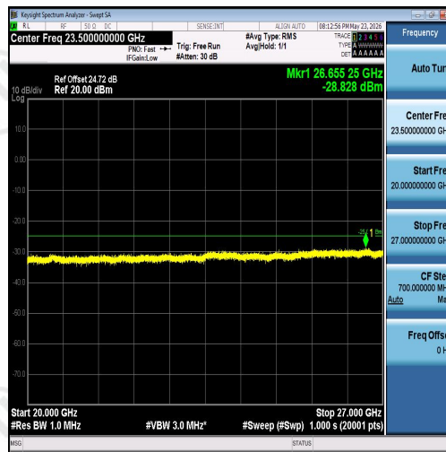
Band7-5MHz-QPSK-21425-25RB#0-20000~270 00-PASS
