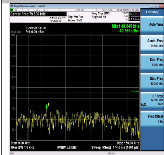
Band7-5MHz-16QAM-21100-1RB#24-0.009~0.1 5-PASS
