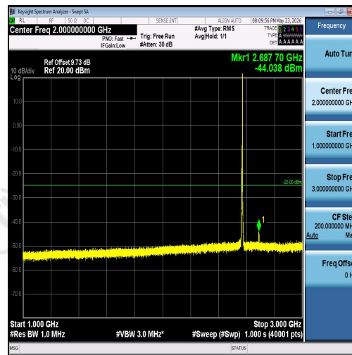
Band7-5MHz-QPSK-21425-1RB#24-1000~3000- PASS
