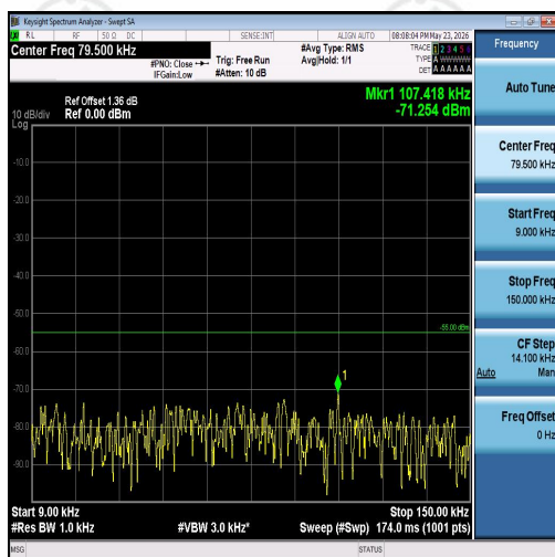
Band7-5MHz-16QAM-21425-1RB#0-0.009~0.15-
