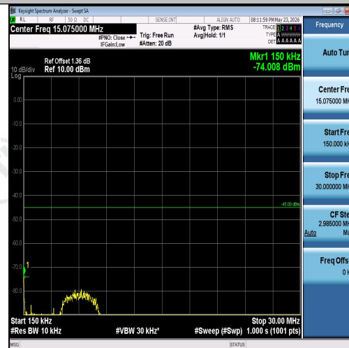
Band7-5MHz-QPSK-21425-25RB#0-0.15~30-PA SS
