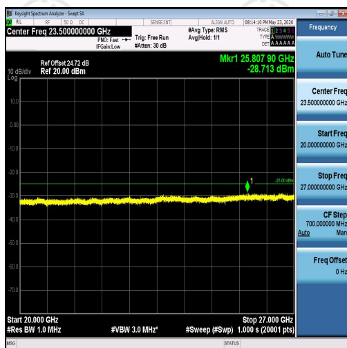
Band7-5MHz-16QAM-21425-25RB#0-20000~27
