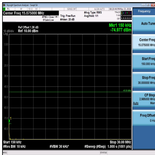
Band7-10MHz-QPSK-20800-50RB#0-0.15~30-PASS
