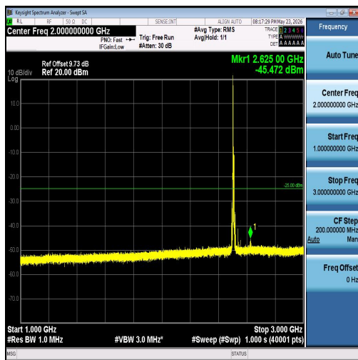
Band7-10MHz-16QAM-20800-1RB#0-1000~300 0-PASS
