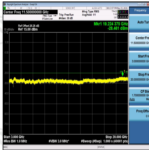
Band7-5MHz-16QAM-21425-25RB#0-3000~200 00-PASS
