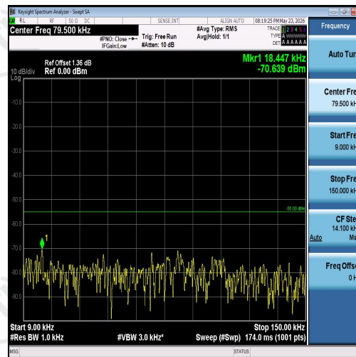
Band7-10MHz-16QAM-20800-1RB#49-0.009~0. 15-PASS
