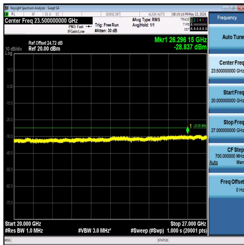
Band7-10MHz-QPSK-20800-1RB#49-20000~27000-PASS
