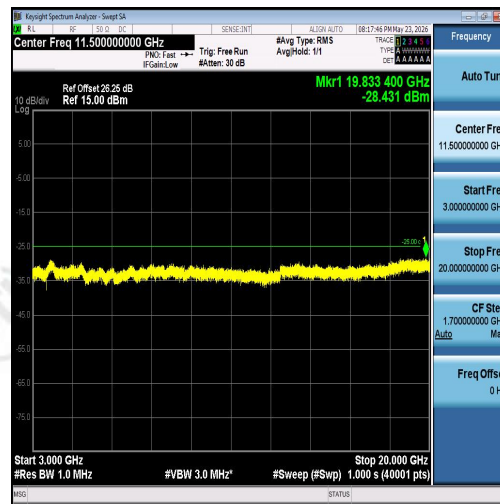
Band7-10MHz-16QAM-20800-1RB#0-3000~200 00-PASS
