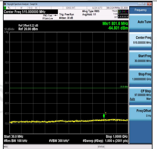
Band7-5MHz-16QAM-21425-25RB#0-30~1000-P ASS
