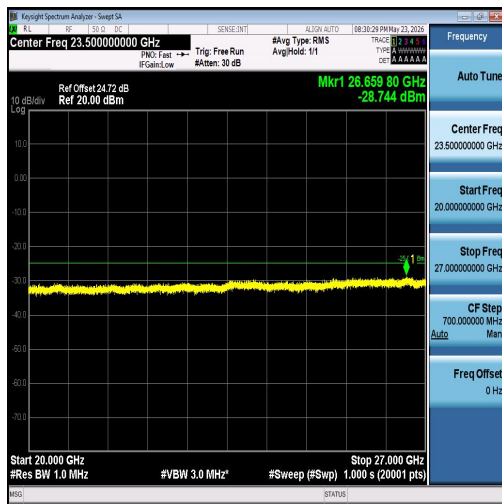
Band7-10MHz-QPSK-21100-1RB#49-20000~27000-PASS
