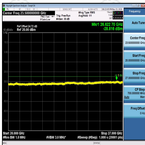
Band7-10MHz-16QAM-20800-50RB#0-20000~2
