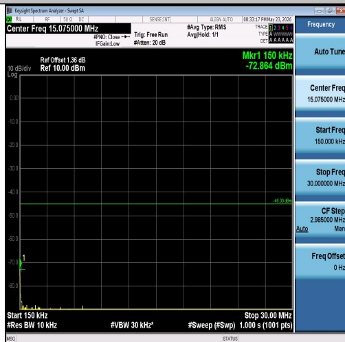
Band7-10MHz-16QAM-21100-50RB#0-0.15~30- PASS
