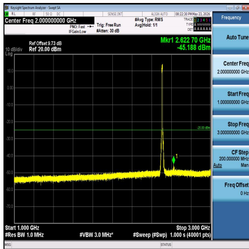
Band7-10MHz-16QAM-20800-50RB#0-1000~30 00-PASS
