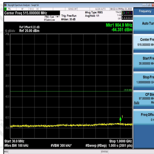
Band7-10MHz-QPSK-21100-50RB#0-30~1000-P ASS
