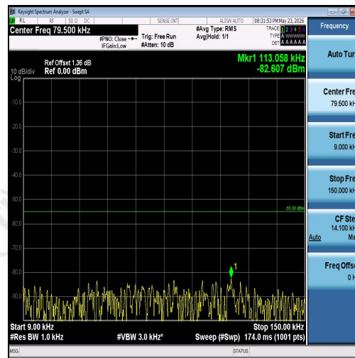
Band7-10MHz-QPSK-21100-50RB#0-0.009~0.15-PASS
