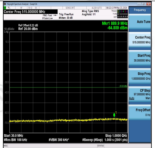
Band7-10MHz-16QAM-20800-50RB#0-30~1000- PASS
