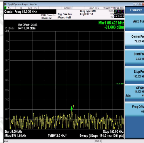
Band7-10MHz-16QAM-21100-50RB#0-0.009~0. 15-PASS
