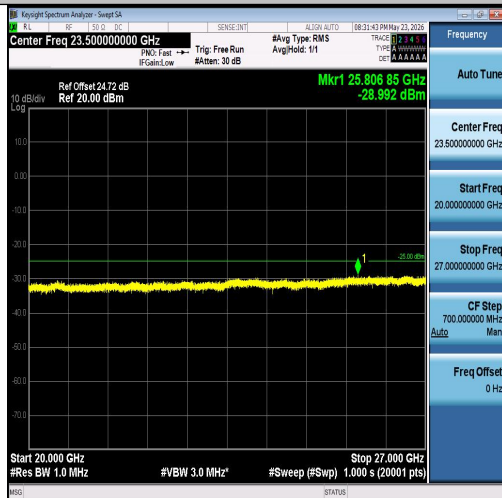
Band7-10MHz-16QAM-21100-1RB#49-20000~2 7000-PASS
