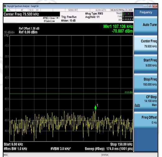
Band7-10MHz-QPSK-21100-1RB#0-0.009~0.15-
