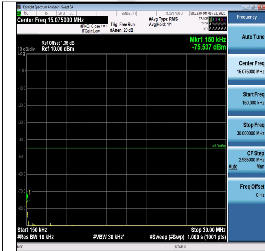
Band7-10MHz-16QAM-20800-50RB#0-0.15~30- PASS
