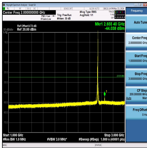
Band7-10MHz-16QAM-21100-1RB#49-1000~30 00-PASS
