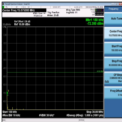
Band7-10MHz-QPSK-21100-50RB#0-0.15~30-P ASS
