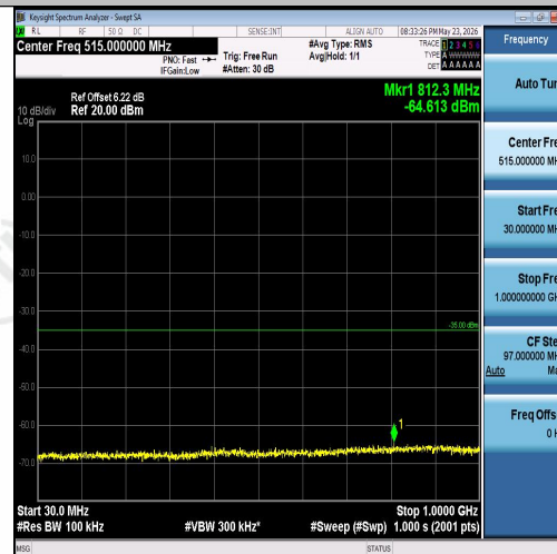
Band7-10MHz-16QAM-21100-50RB#0-30~1000- PASS
