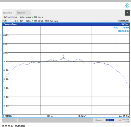
3DH5-Ant1-2441-0~Reference-PASS
