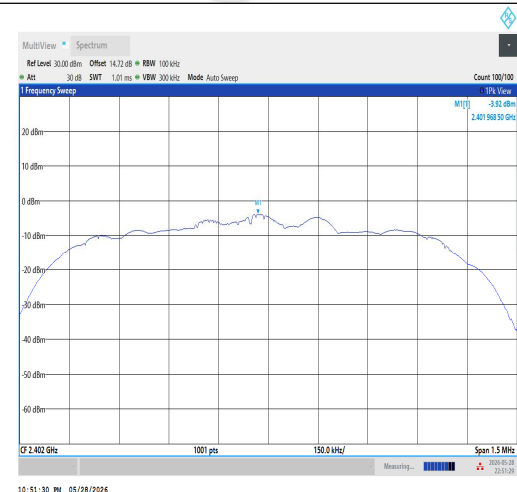
3DH5-Ant1-2402-0~Reference-PASS
