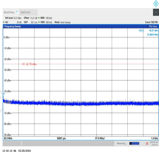
DH5-Ant1-2480-30~1000-PASS
