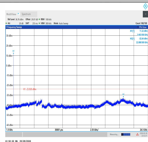
3DH5-Ant1-2402-1000~26500-PASS
