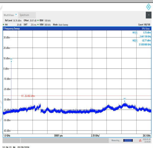
3DH5-Ant1-2441-1000~26500-PASS
