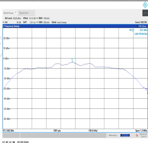
2DH5-Ant1-2402-0~Reference-PASS
