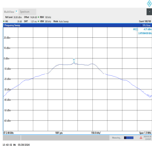
DH5-Ant1-2480-0~Reference-PASS
