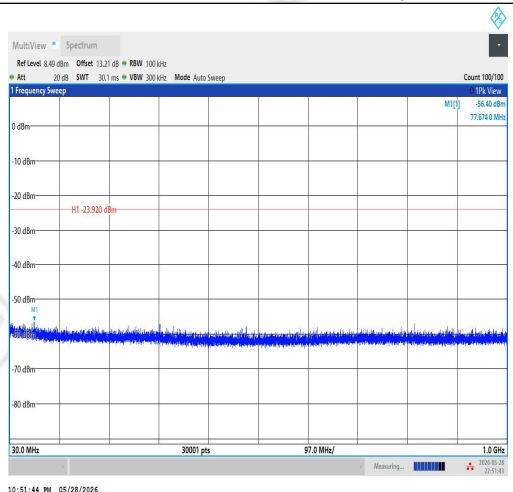
3DH5-Ant1-2402-30~1000-PASS
