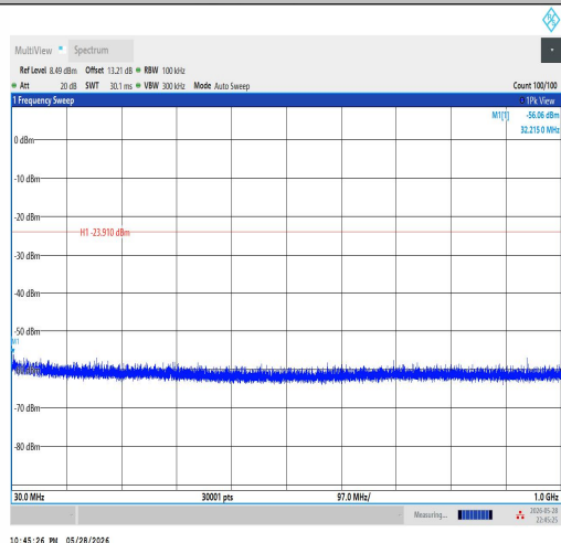
2DH5-Ant1-2402-30~1000-PASS
