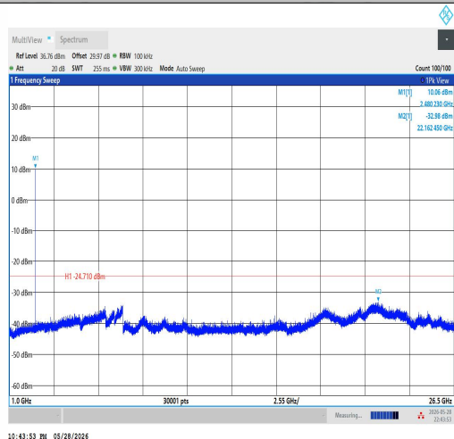
DH5-Ant1-2480-1000~26500-PASS
