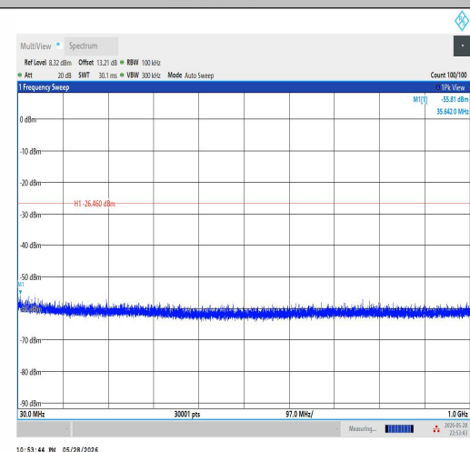
3DH5-Ant1-2441-30~1000-PASS
