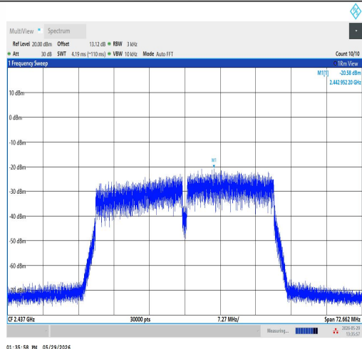
11N40SISO-Ant1-2437-PASS
