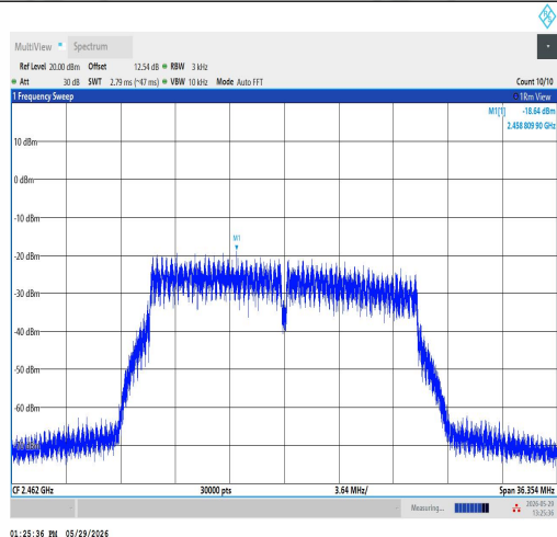
11N20SISO-Ant1-2462-PASS
