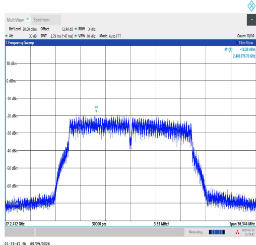
11N20SISO-Ant1-2412-PASS
