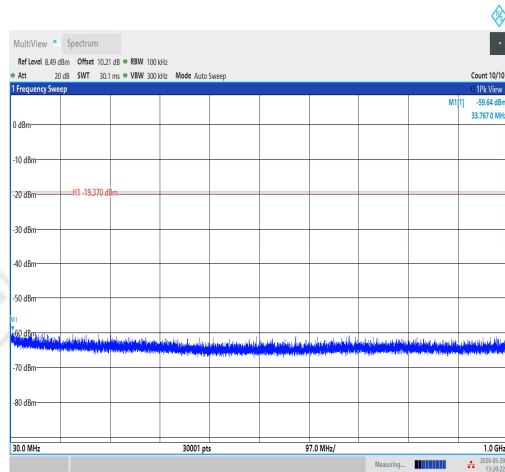
11N20SISO-Ant1-2412-30~1000-PASS
