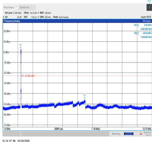
11N40SISO-Ant1-2422-1000~12750-PASS
