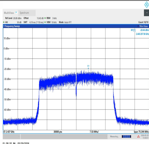
11AX40SISO-Ant1-2437-PASS
