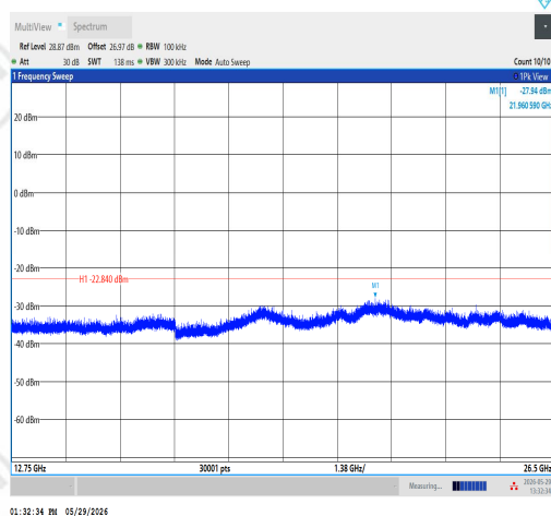
11N40SISO-Ant1-2422-12750~26500-PASS
