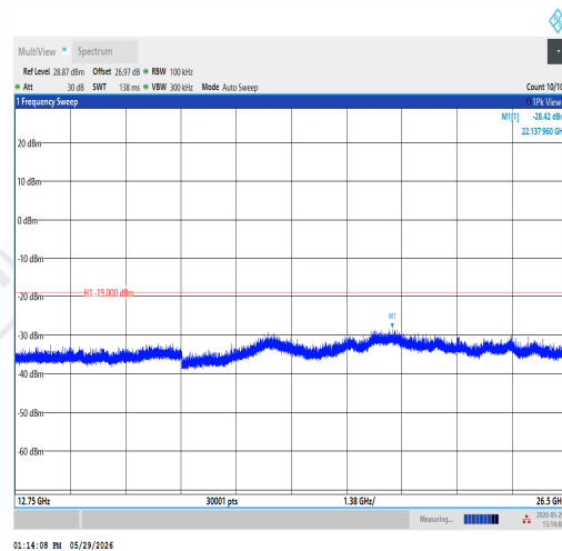
11G-Ant1-2462-12750~26500-PASS
