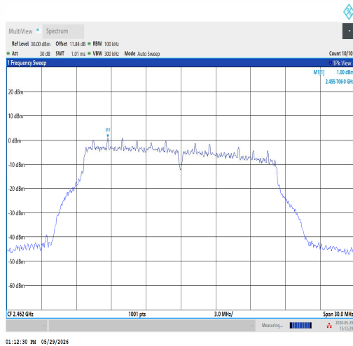
11G-Ant1-2462-0~Reference-PASS
