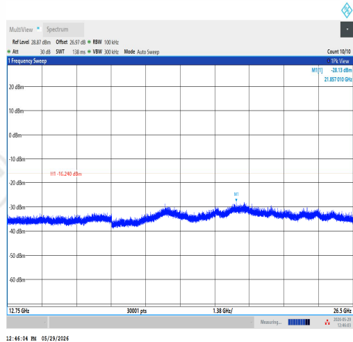
11B-Ant1-2462-12750~26500-PASS
