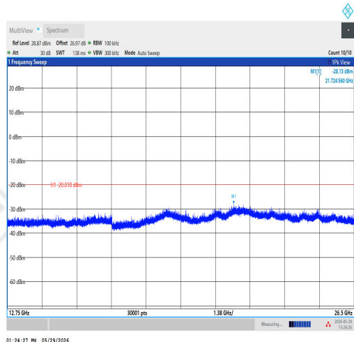
11N20SISO-Ant1-2437-12750~26500-PASS
