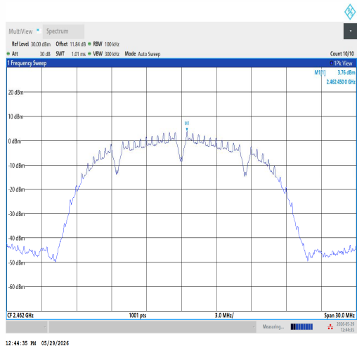
11B-Ant1-2462-0~Reference-PASS
