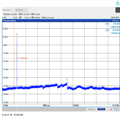
11B-Ant1-2462-1000~12750-PASS
