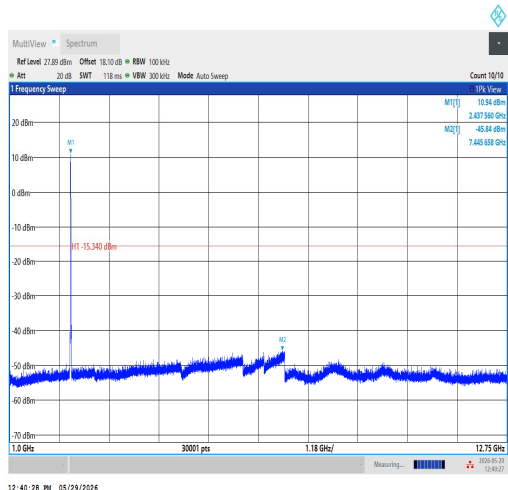
11B-Ant1-2437-1000~12750-PASS
