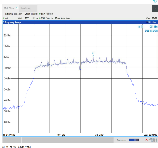
11N20SISO-Ant1-2437-0~Reference-PASS
