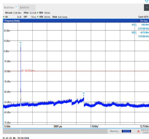
11N20SISO-Ant1-2412-1000~12750-PASS
