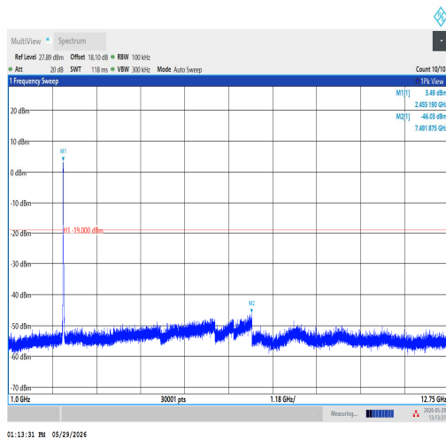
11G-Ant1-2462-1000~12750-PASS
