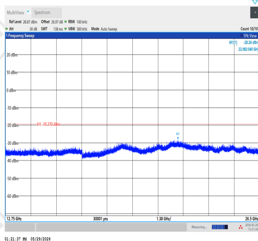
11N20SISO-Ant1-2412-12750~26500-PASS
