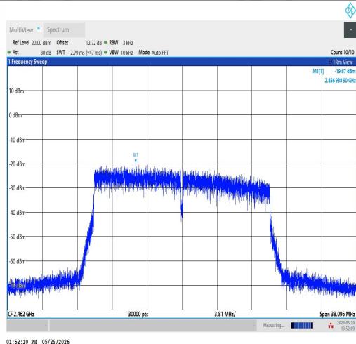
11AX20SISO-Ant1-2462-PASS
