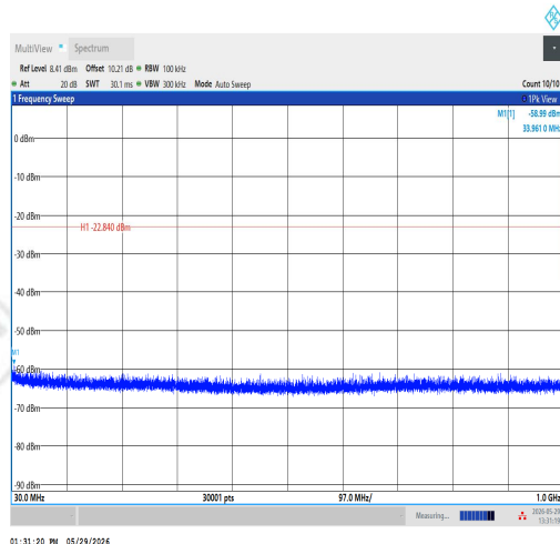
11N40SISO-Ant1-2422-30~1000-PASS
