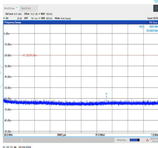
11N20SISO-Ant1-2437-30~1000-PASS
