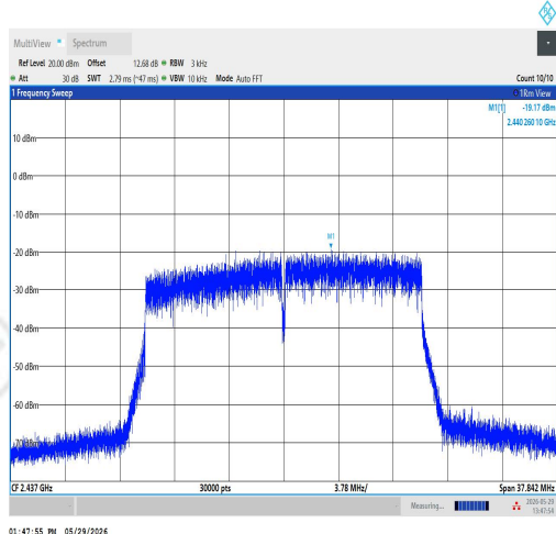
11AX20SISO-Ant1-2437-PASS
