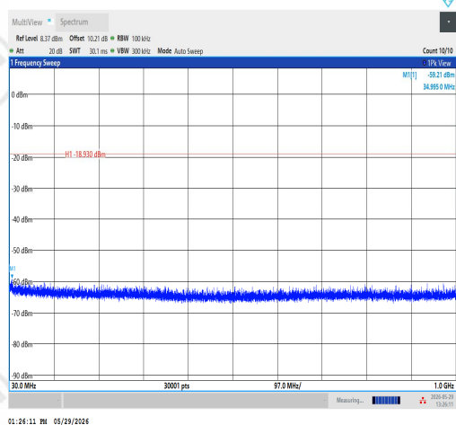
11N20SISO-Ant1-2462-30~1000-PASS
