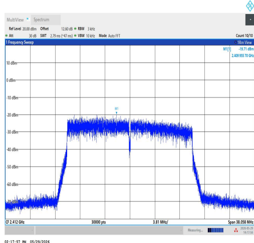
11AX20SISO-Ant1-2412-PASS
