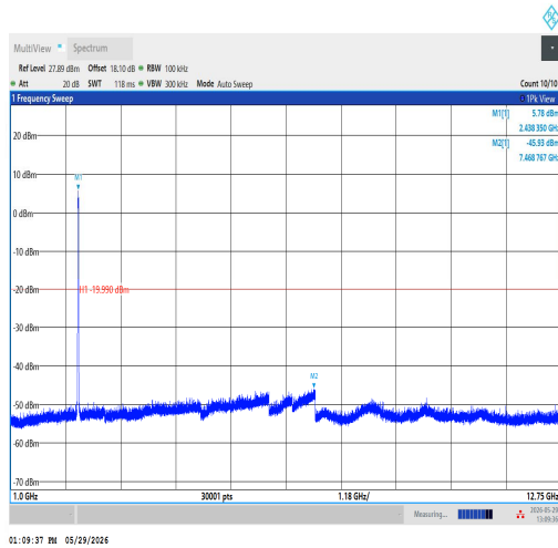
11G-Ant1-2437-1000~12750-PASS
