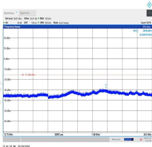
11B-Ant1-2437-12750~26500-PASS
