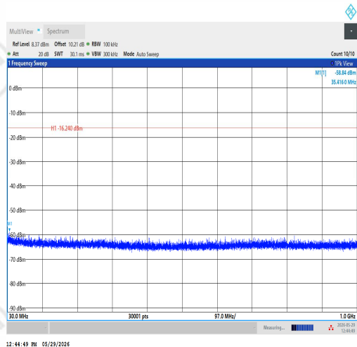
11B-Ant1-2462-30~1000-PASS
