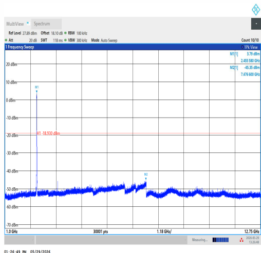
11N20SISO-Ant1-2462-1000~12750-PASS
