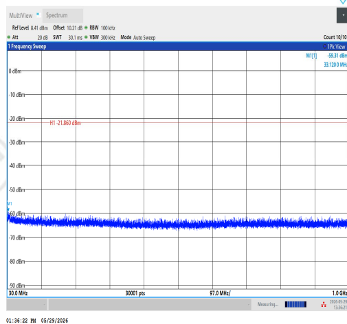
11N40SISO-Ant1-2437-30~1000-PASS
