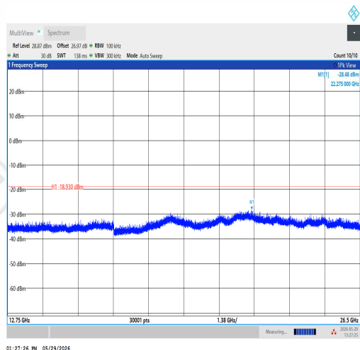
11N20SISO-Ant1-2462-12750~26500-PASS
