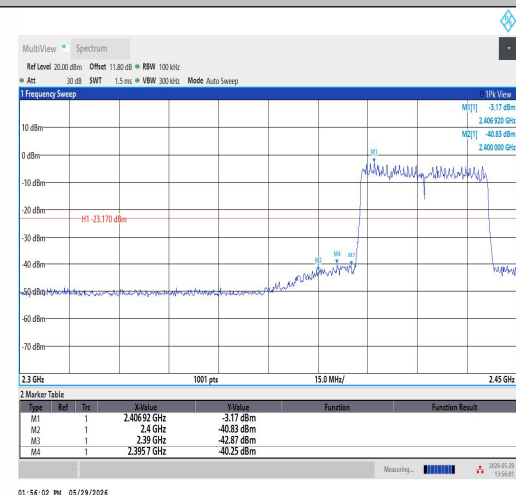
11AX40SISO-Ant1-2422-PASS
