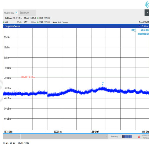
11AX20SISO-Ant1-2437-12750~26500-PASS
