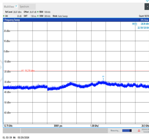
11AX20SISO-Ant1-2462-12750~26500-PASS
