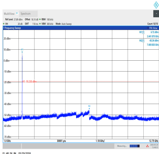
11AX20SISO-Ant1-2437-1000~12750-PASS
