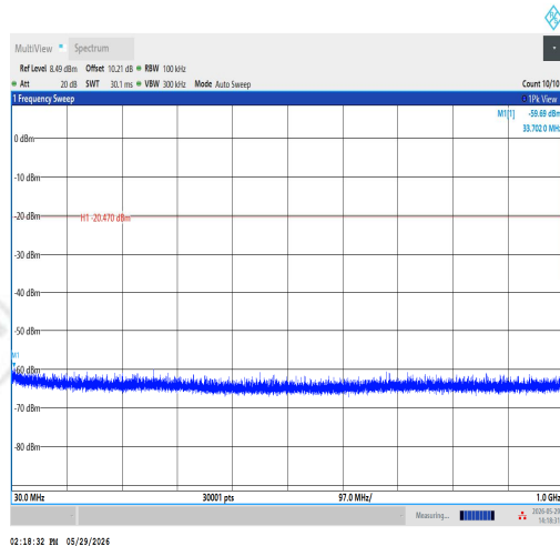
11AX20SISO-Ant1-2412-30~1000-PASS
