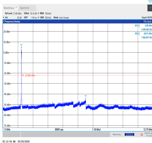
11AX40SISO-Ant1-2452-1000~12750-PASS
