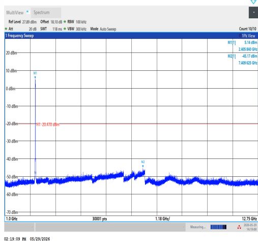
11AX20SISO-Ant1-2412-1000~12750-PASS
