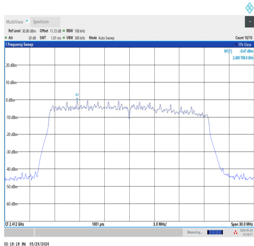
11AX20SISO-Ant1-2412-0~Reference-PASS
