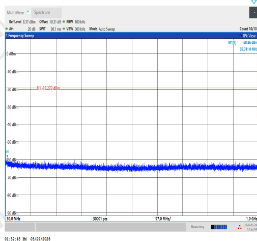
11AX20SISO-Ant1-2462-30~1000-PASS
