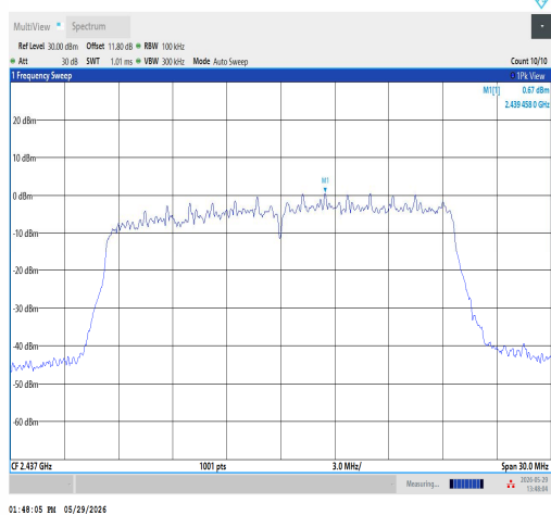
11AX20SISO-Ant1-2437-0~Reference-PASS
