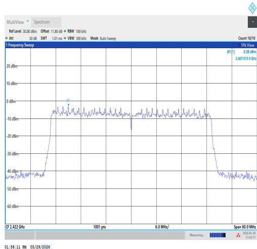
11AX40SISO-Ant1-2422-0~Reference-PASS
