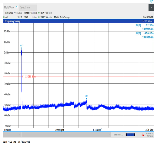
11AX40SISO-Ant1-2422-1000~12750-PASS
