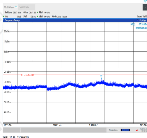
11AX40SISO-Ant1-2422-12750~26500-PASS
