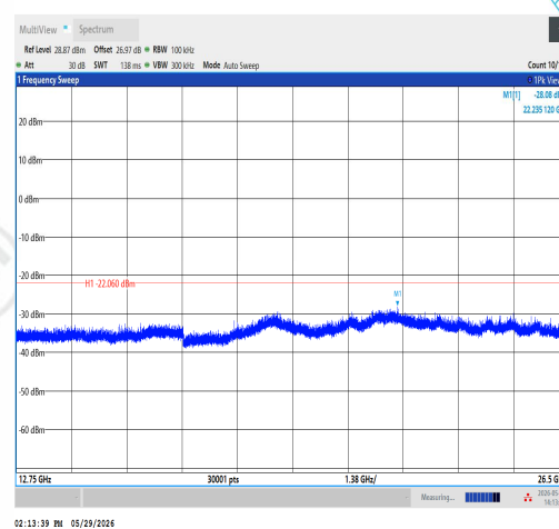
11AX40SISO-Ant1-2452-12750~26500-PASS
