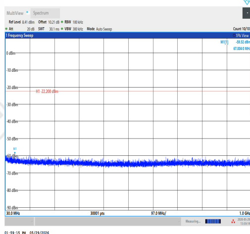
11AX40SISO-Ant1-2437-30~1000-PASS
