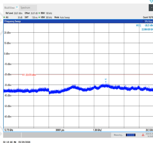
11AX20SISO-Ant1-2412-12750~26500-PASS
