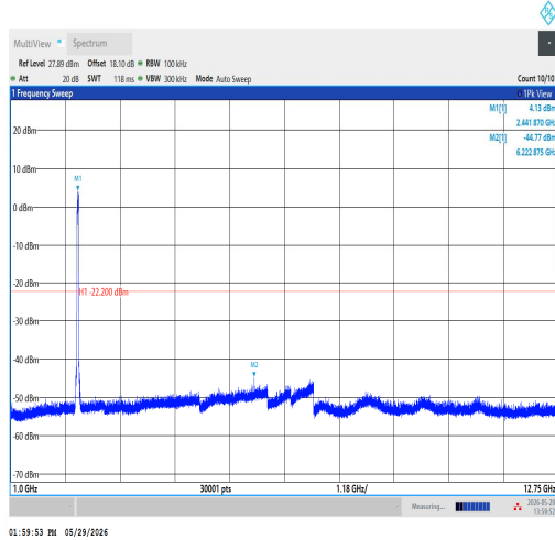
11AX40SISO-Ant1-2437-1000~12750-PASS
