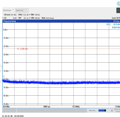
11AX40SISO-Ant1-2422-30~1000-PASS
