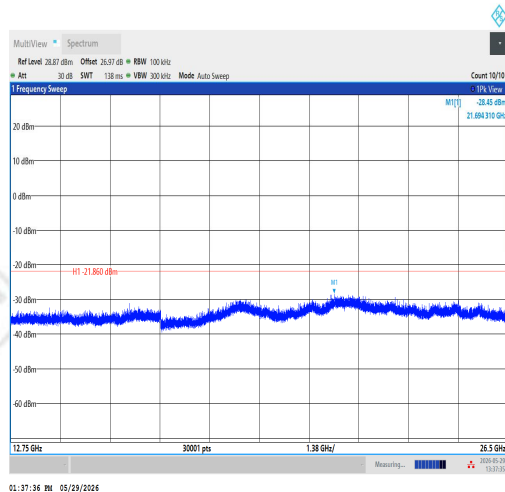
11N40SISO-Ant1-2437-12750~26500-PASS
