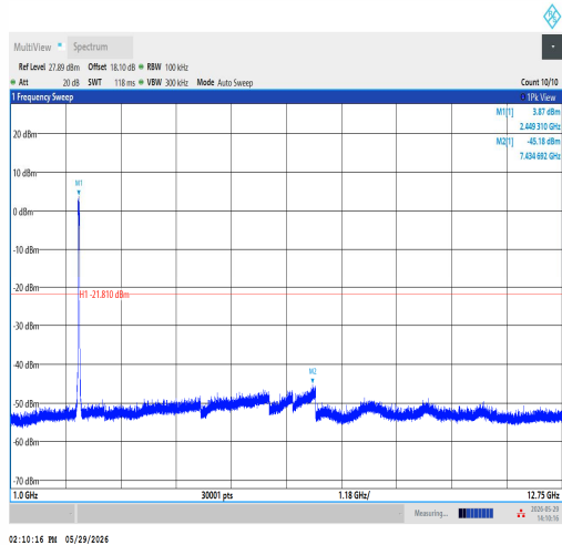
11N40SISO-Ant1-2452-1000~12750-PASS
