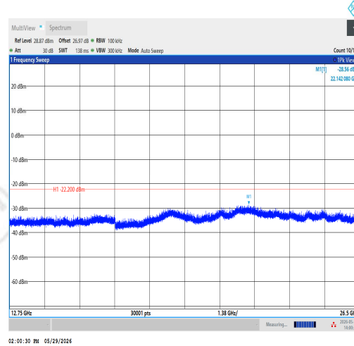
11AX40SISO-Ant1-2437-12750~26500-PASS
