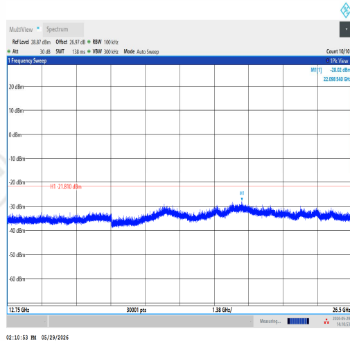
11N40SISO-Ant1-2452-12750~26500-PASS
