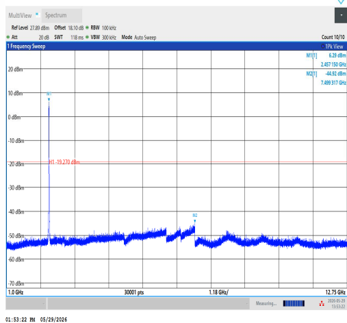
11AX20SISO-Ant1-2462-1000~12750-PASS
