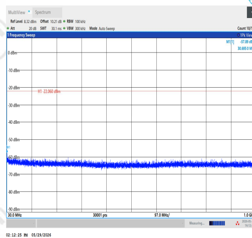
11AX40SISO-Ant1-2452-30~1000-PASS
