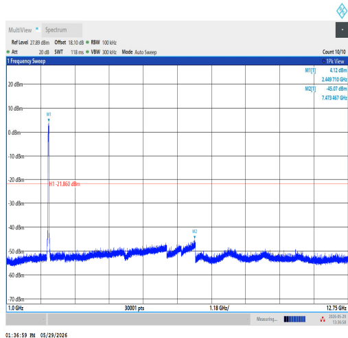
11N40SISO-Ant1-2437-1000~12750-PASS
