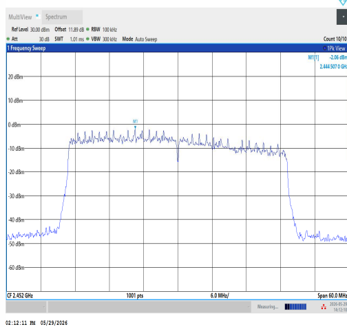
11AX40SISO-Ant1-2452-0~Reference-PASS
