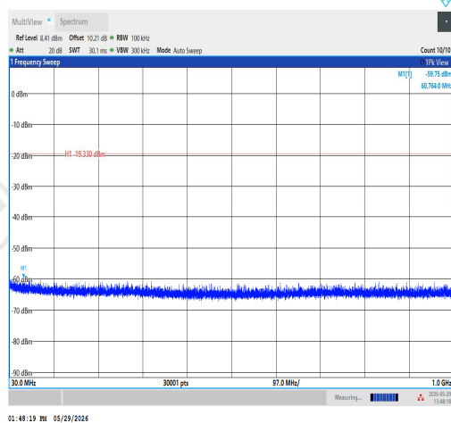
11AX20SISO-Ant1-2437-30~1000-PASS
