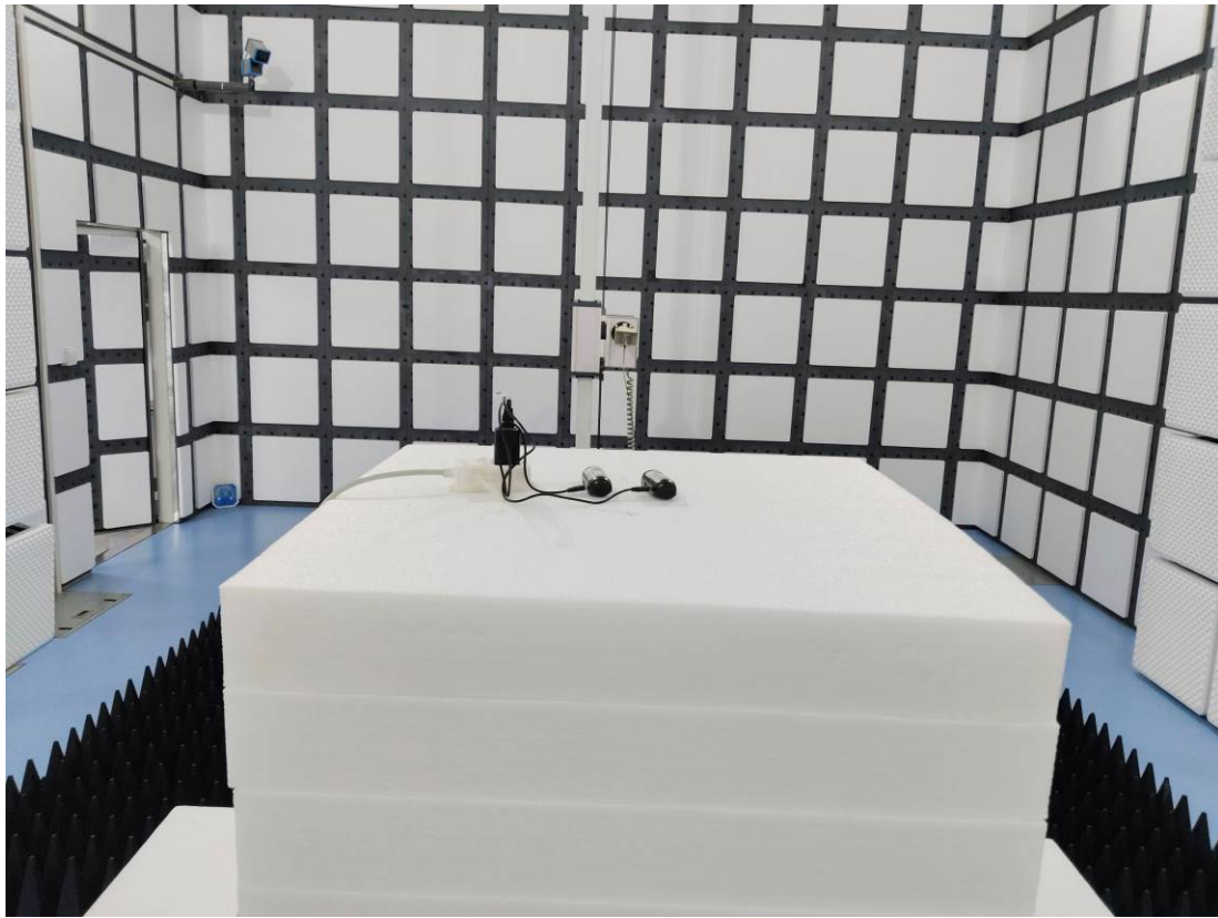
RE-FrontView (18 GHz-25 GHz)
