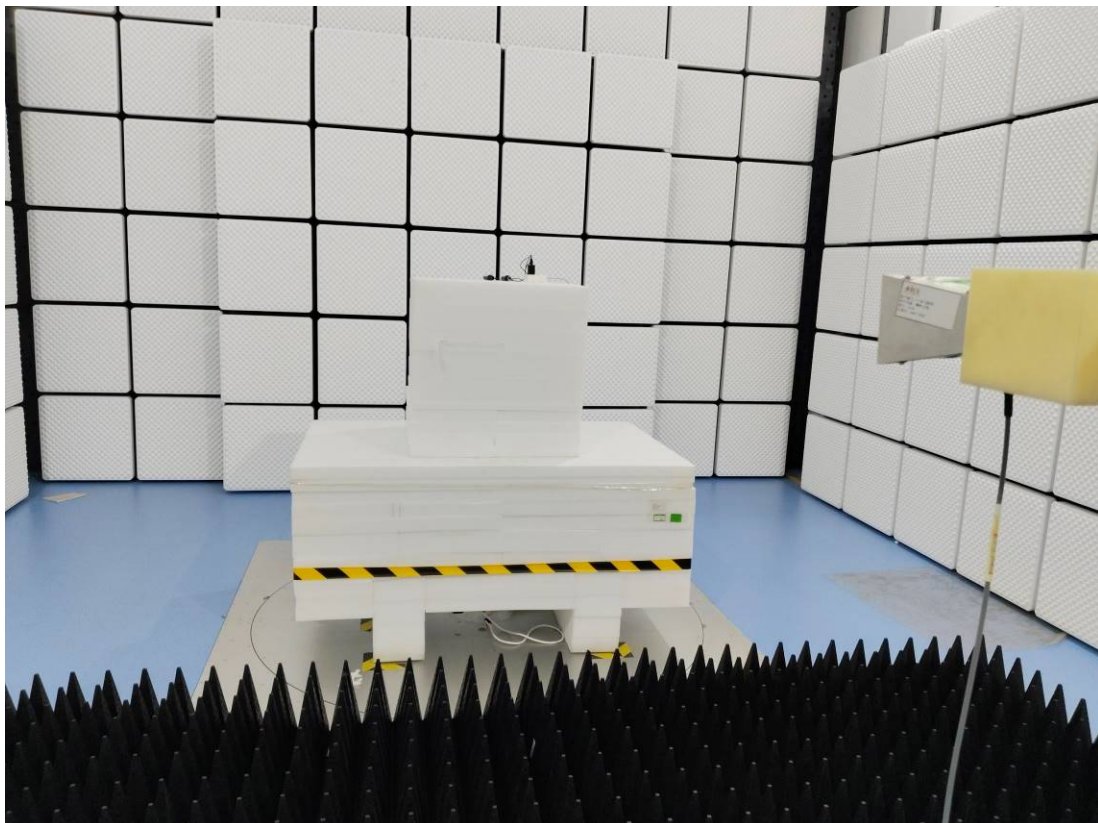
RE-Back View (18 GHz-25 GHz)
