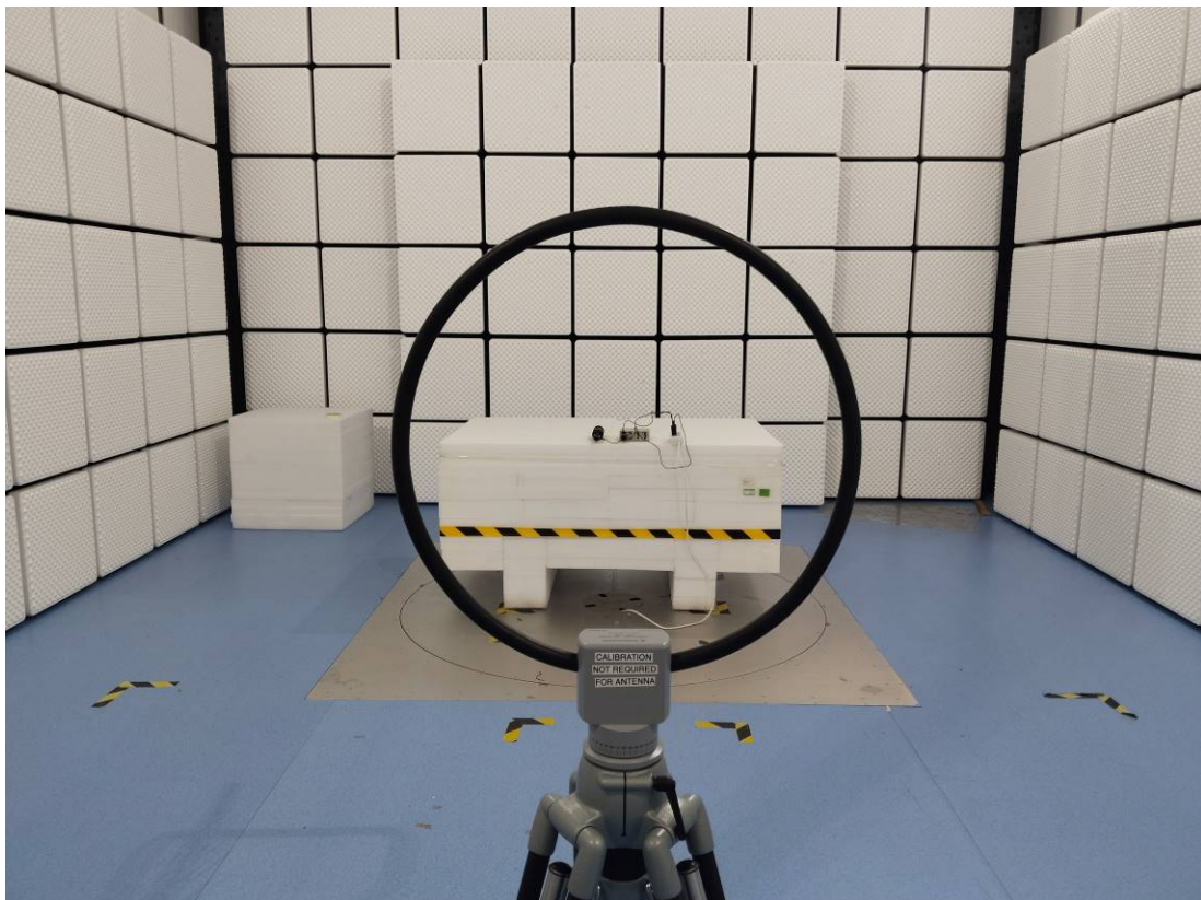
RE-Back View (9kHz~30MHz)
