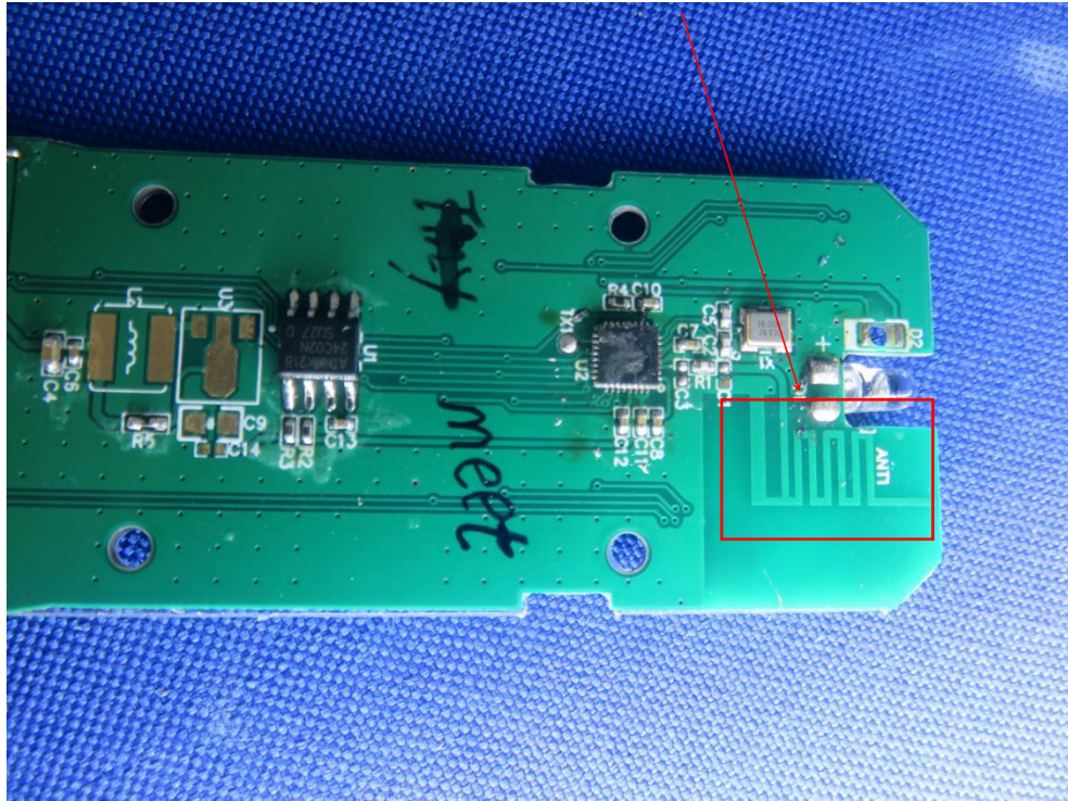
TX Remote control ANT
