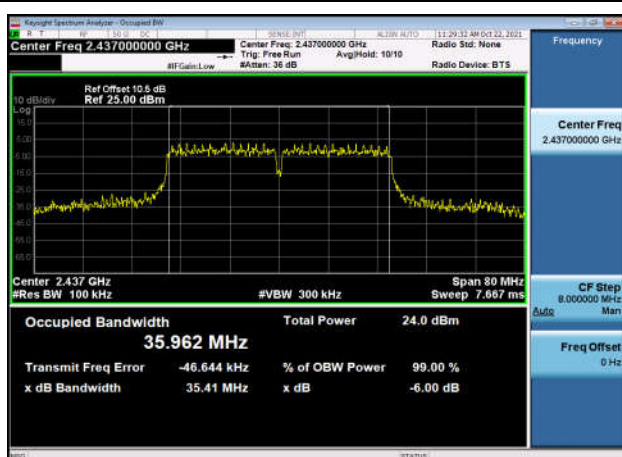
6dB Bandwidth-802.11n(HT40),2437MHz
