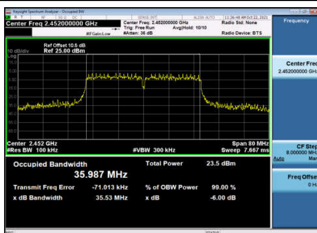
6dB Bandwidth-802.11n(HT40),2452MHz
