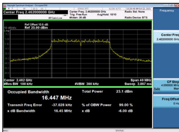
6dB Bandwidth-802.11g,2462MHz,Ant0
