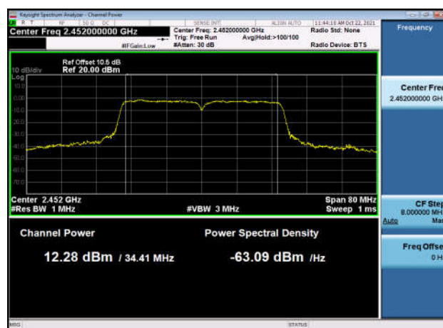
Output Power-802.11n(HT40),2452MHz
