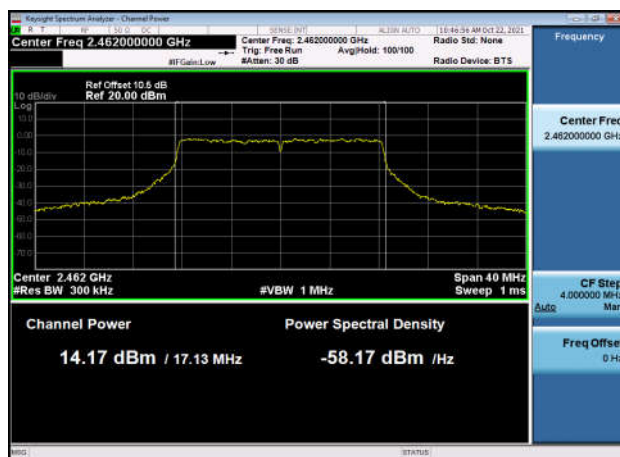
Output Power-802.11g,2462MHz,Ant0
