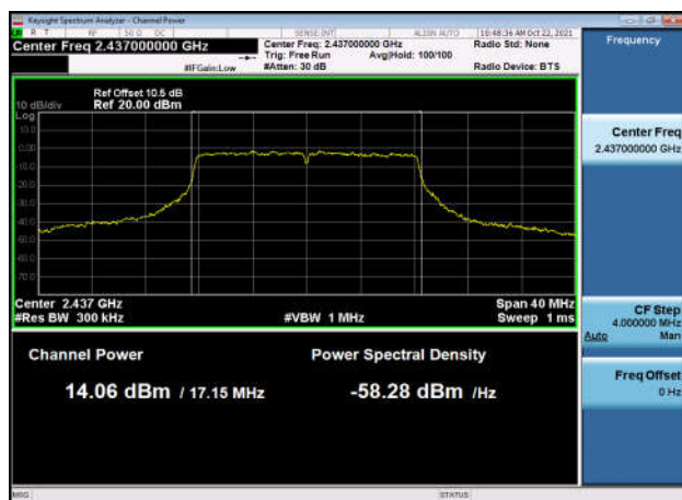
Output Power-802.11g,2437MHz,Ant0
