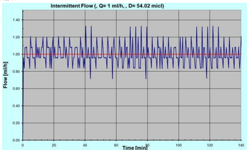
Figure 13.1. Delivery Startup Graph, First 2 Hours of Test Period, 1 mL/h
