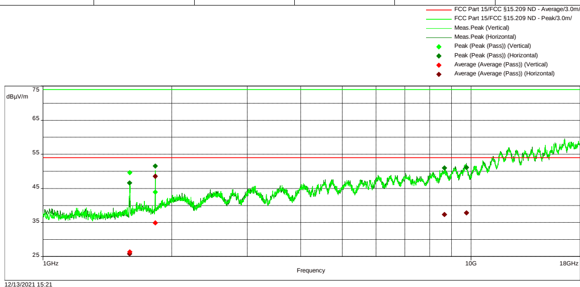
Figure 2-34 – RE Spurious Emissions 1-18 GHz – Mid Channel
