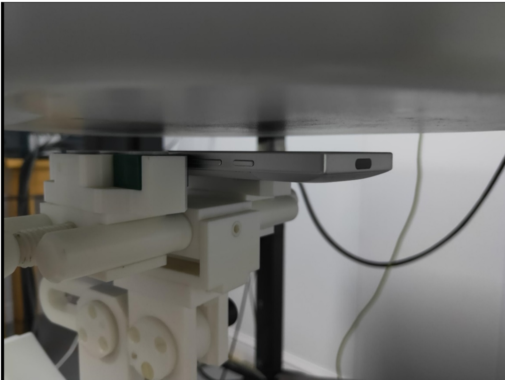
body-worn Back Side Setup Photo (10mm) (Hotspot open)
