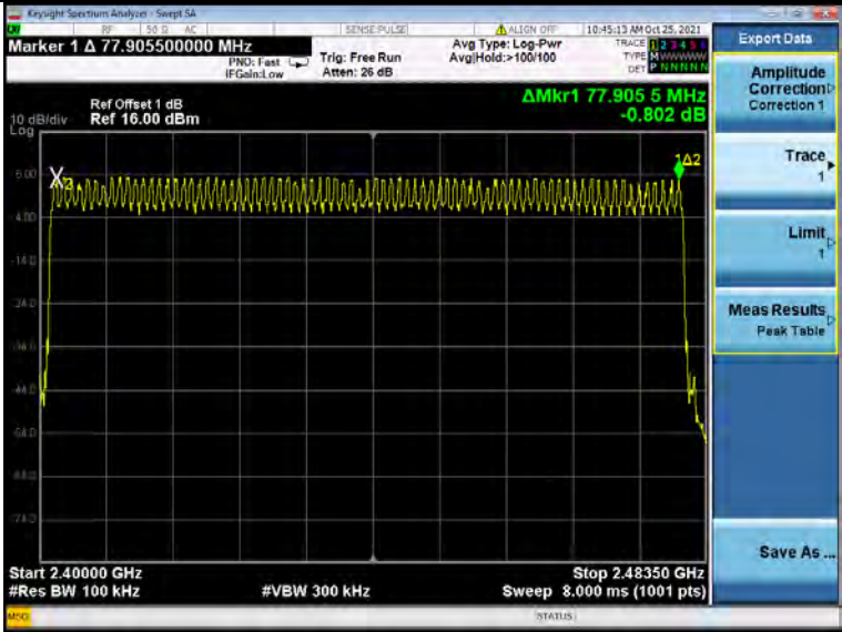
8DPSK Modulation
