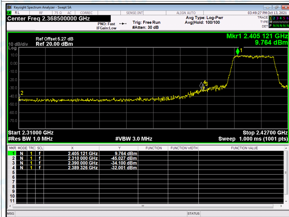
Restrict Band NVNT n(HT20) 2412MHz Ant1 Average
