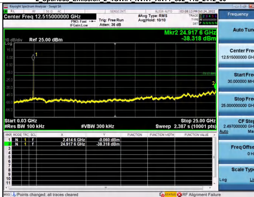
2_Spurious Emission_2_4GWiFi_NVNT ANT1 802_11b 2412_00
