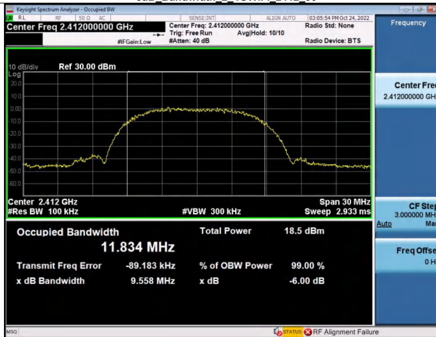
-6dB_Bandwidth_2_4WiFi_2412_00
