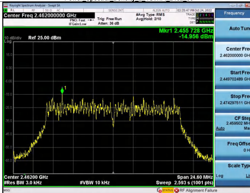
Power Spectral Density 2 4GWiFi 2462_00
