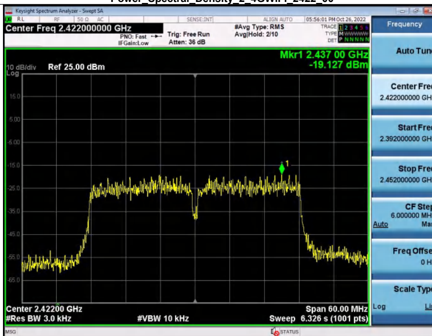
Power Spectral Density 2 4GWiFi 2422_00
