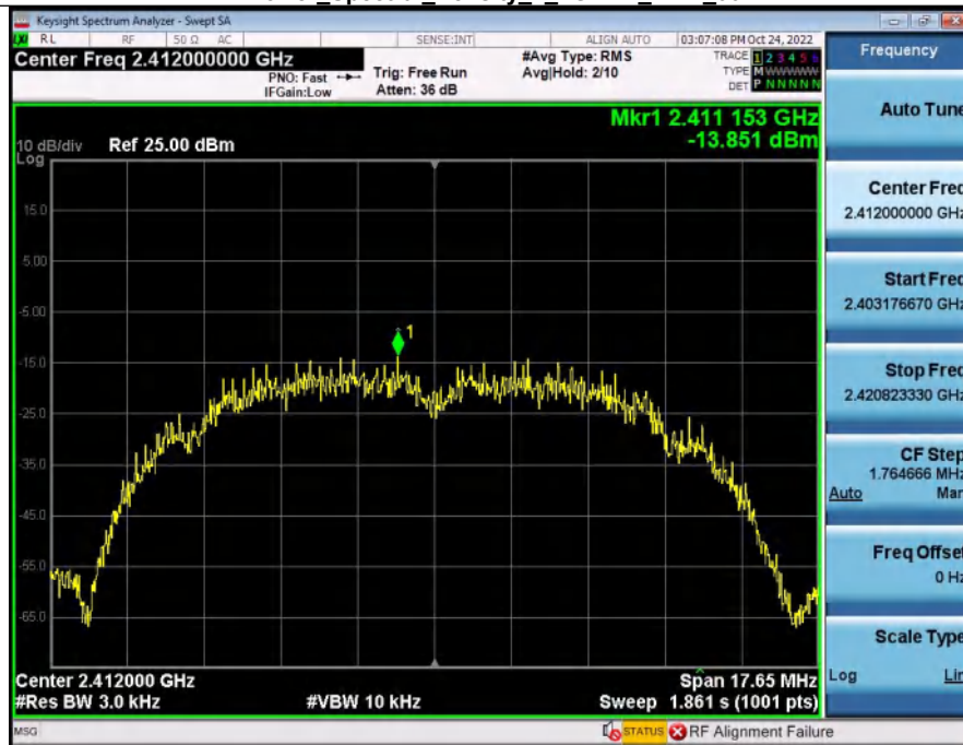
Power Spectral Density 2 4GWiFi 2412 00
