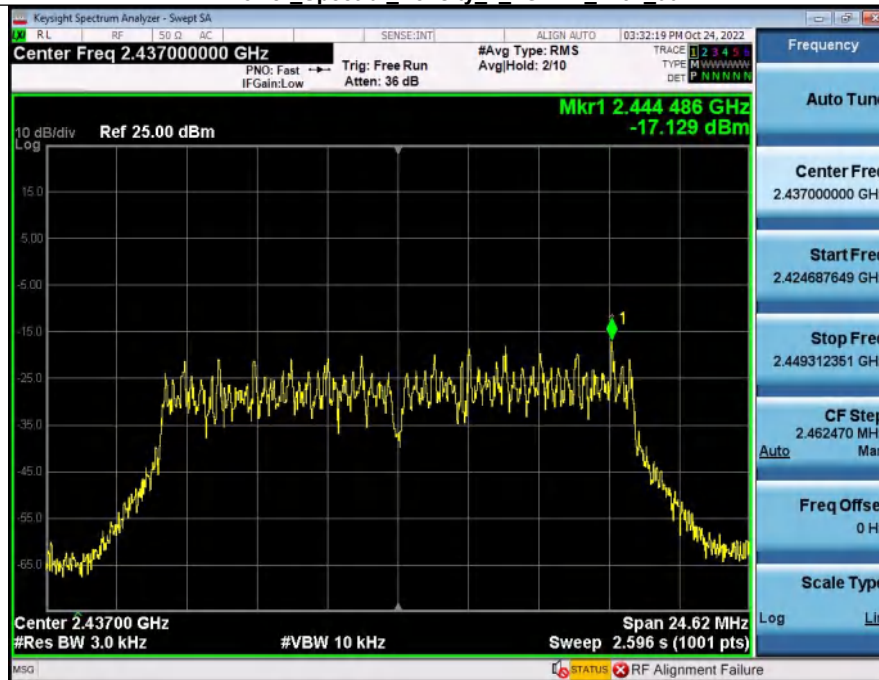
Power Spectral Density 2 4GWiFi 2437_00
