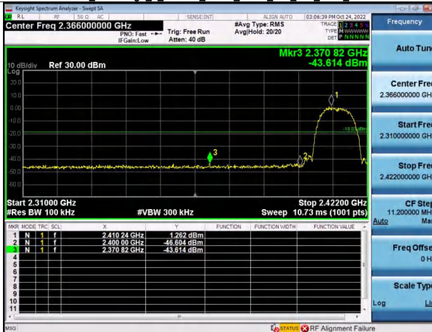
2_Bandedge_2_4GWiFi_NVNT_ANT1_802_11b_2412_00
