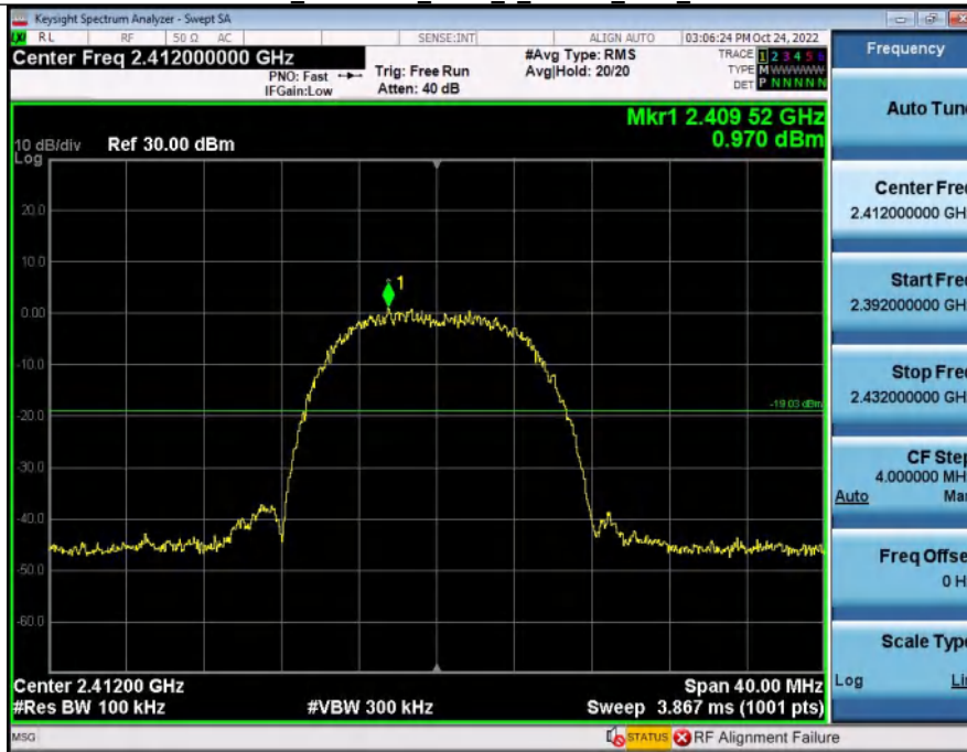
2_Bandedge_2_4GWiFi_NVNT_ANT1_802_11b_2412_00
