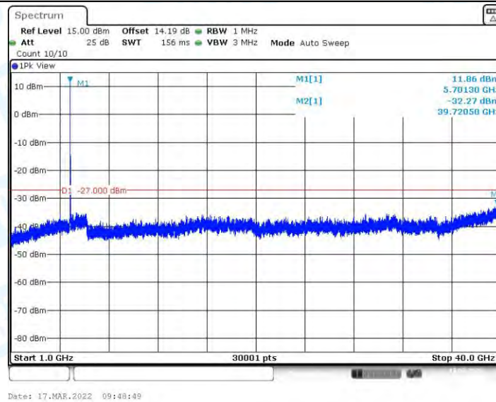
11N20SISO_Ant1_5700_1000~40000
