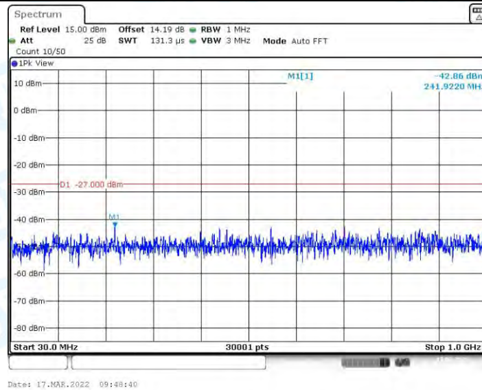
11N20SISO_Ant1_5700_30~1000
