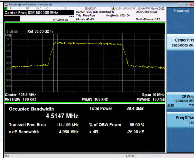
Band5-5MHz-QPSK-20525-25RB#0
