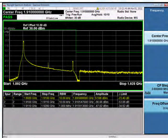
Band2-15MHz-QPSK-19125-1RB#74
