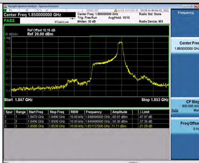
Band2-1.4MHz-QPSK-18607-6RB#0
