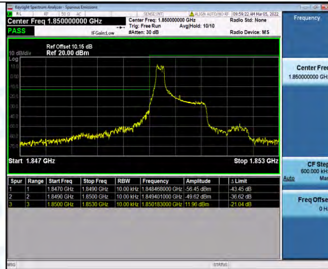
Band2-1.4MHz-16QAM-18607-1RB#5
