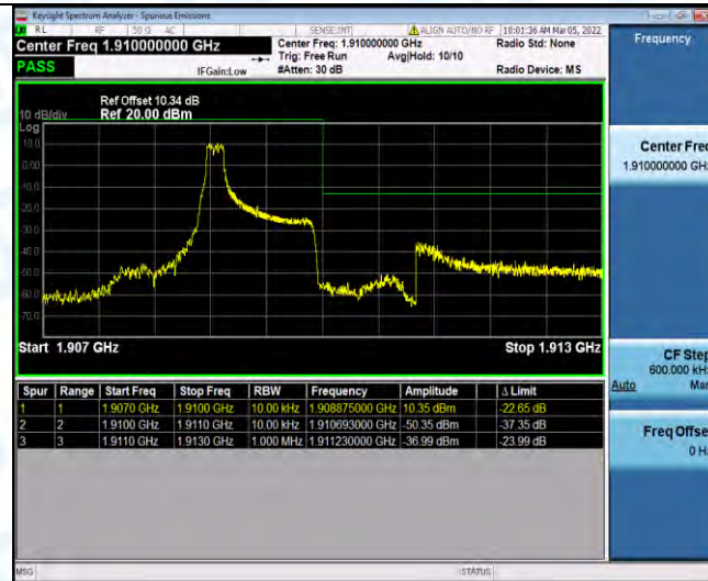
Band2-1.4MHz-16QAM-19193-1RB#5
