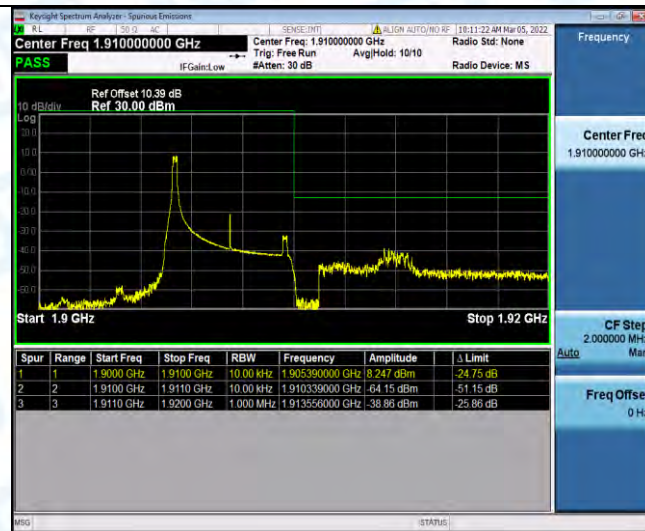
Band2-5MHz-16QAM-19175-1RB#24
