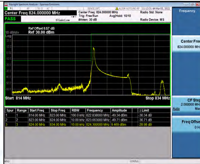
Band5-5MHz-16QAM-20425-1RB#24
