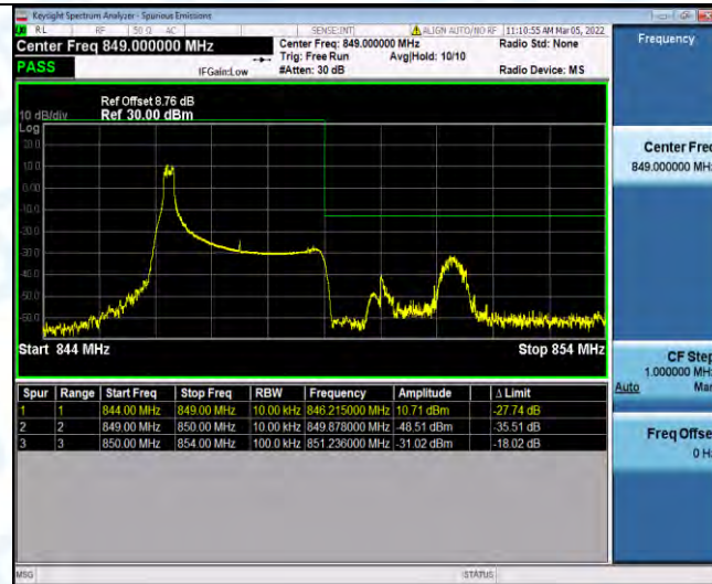
Band5-3MHz-16QAM-20635-1RB#14
