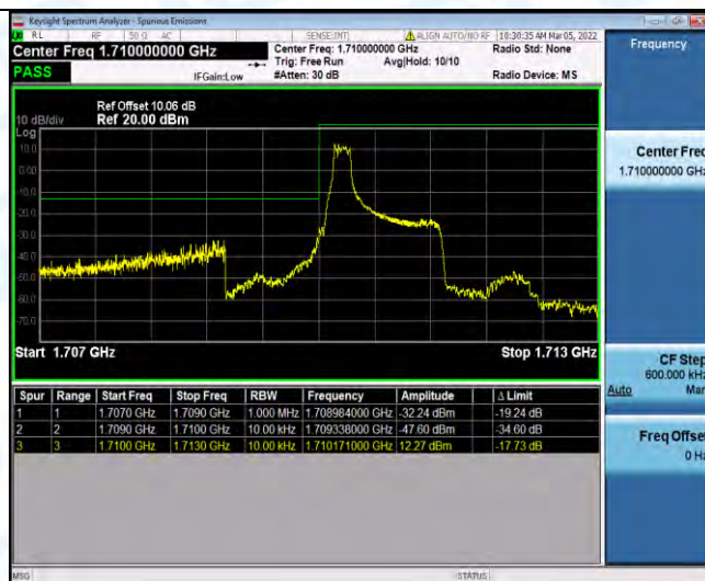
Band4-1.4MHz-QPSK-19957-1RB#5
