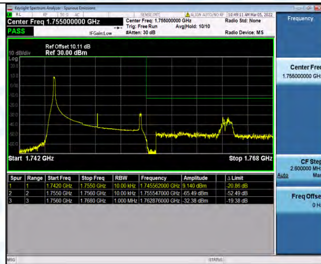
Band4-10MHz-16QAM-20350-1RB#49
