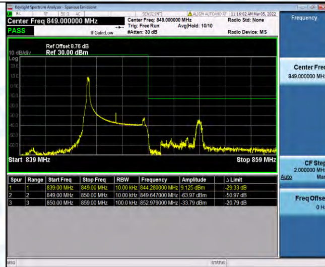
Band5-5MHz-16QAM-20625-1RB#24
