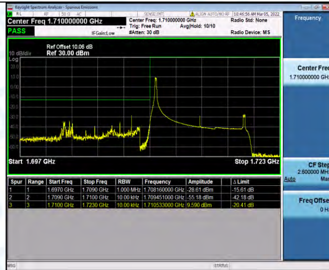
Band4-10MHz-16QAM-20000-1RB#49
