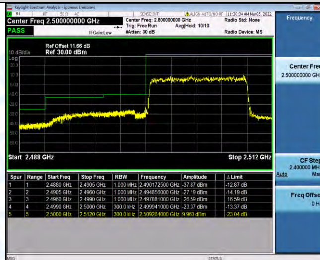
Band7-10MHz-QPSK-21400-1RB#0
