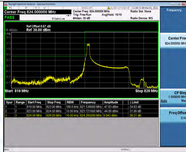
Band5-3MHz-16QAM-20415-1RB#14
