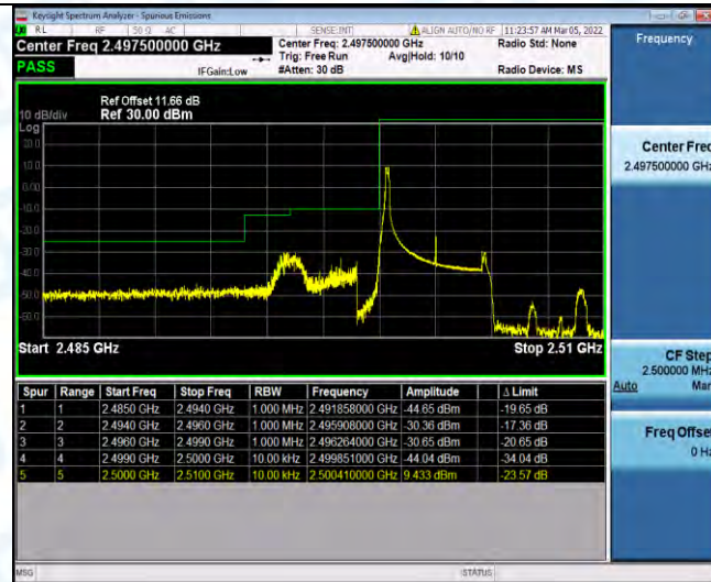
Band7-5MHz-16QAM-20775-1RB#24
