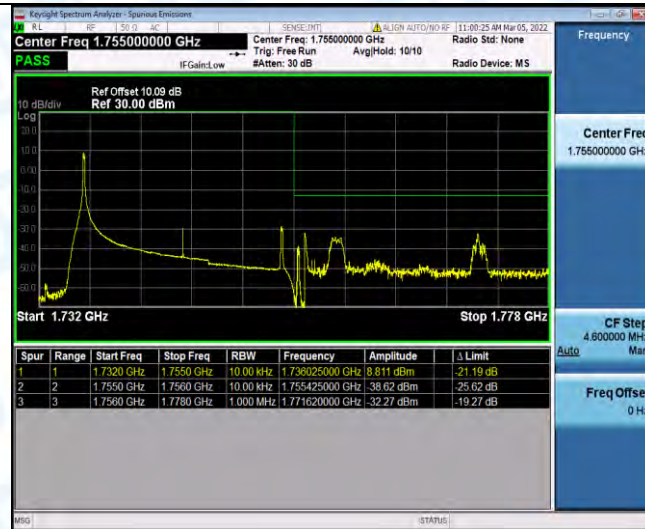
Band4-20MHz-16QAM-20300-1RB#99
