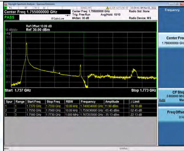
Band4-15MHz-QPSK-20325-1RB#74
