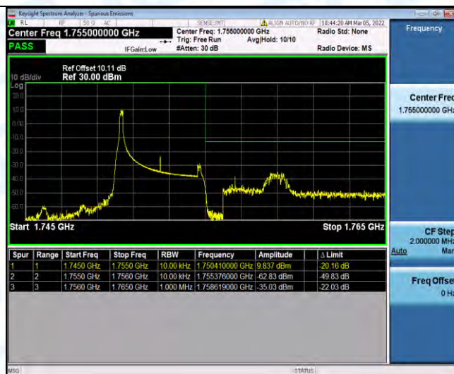
Band4-5MHz-16QAM-20375-1RB#24
