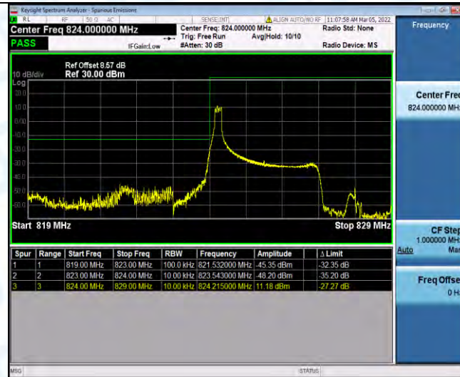
Band5-3MHz-QPSK-20415-1RB#14
