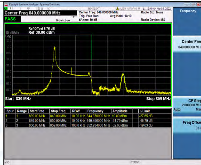
Band5-5MHz-QPSK-20625-1RB#24
