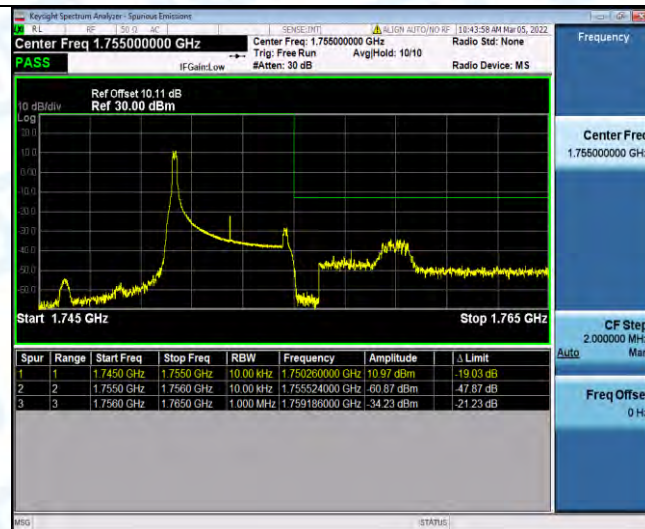
Band4-5MHz-QPSK-20375-1RB#24
