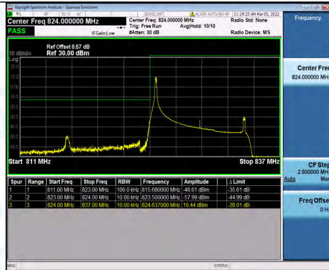
Band5-10MHz-QPSK-20450-1RB#49
