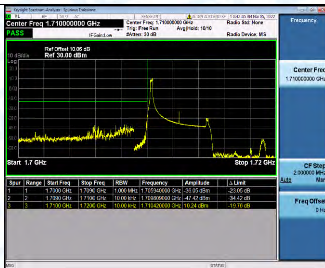
Band4-5MHz-16QAM-19975-1RB#24
