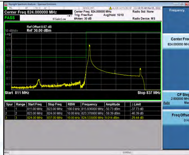
Band5-10MHz-16QAM-20450-1RB#49
