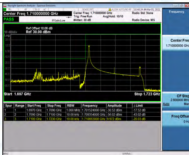
Band4-10MHz-QPSK-20000-1RB#49
