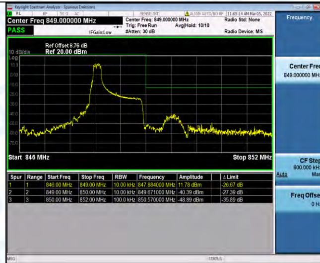
Band5-1.4MHz-QPSK-20643-1RB#5
