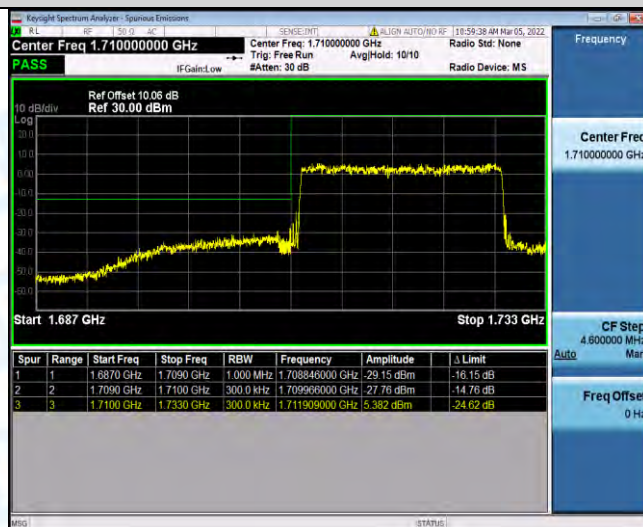
Band4-20MHz-16QAM-20300-1RB#0
