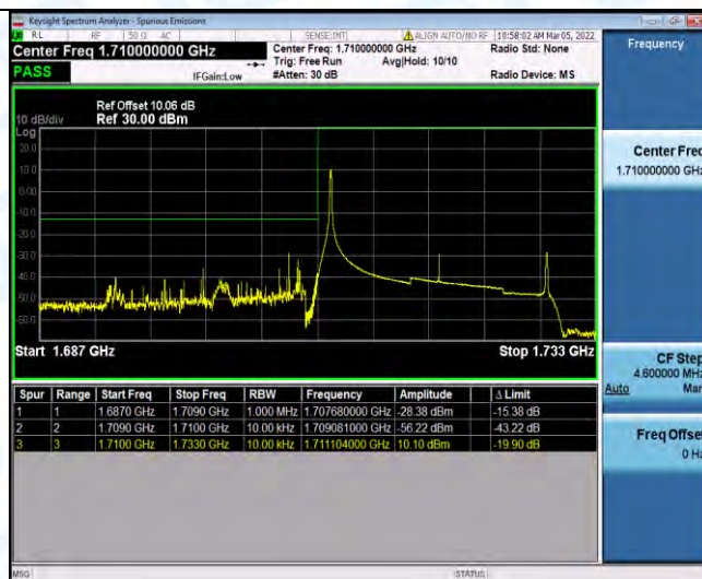
Band4-20MHz-16QAM-20050-1RB#99
