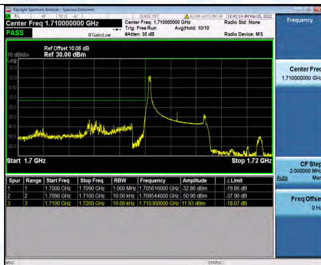
Band4-5MHz-QPSK-19975-1RB#24
