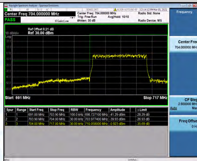
Band17-10MHz-QPSK-23800-1RB#0
