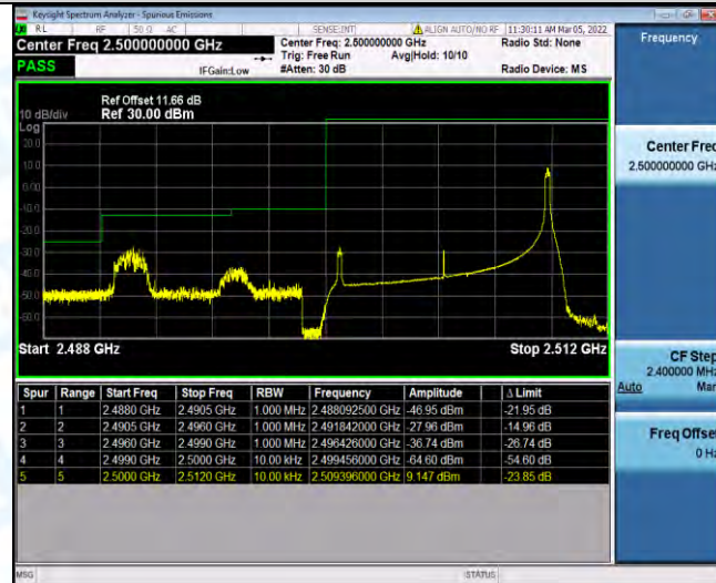
Band7-10MHz-16QAM-20800-50RB#0
