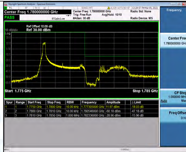
Band66-3MHz-QPSK-132657-1RB#14
