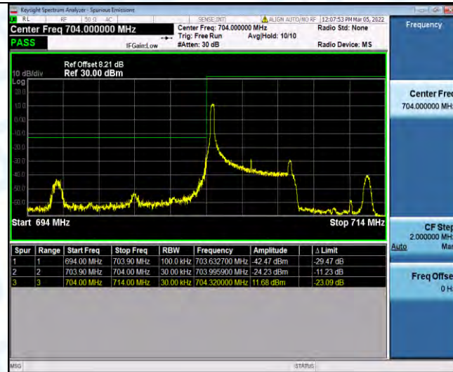
Band17-5MHz-16QAM-23755-1RB#24
