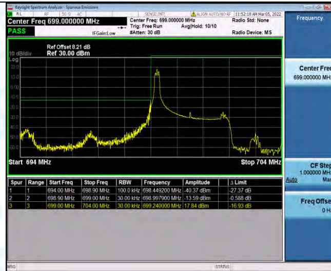
Band12-3MHz-QPSK-23025-1RB#14
