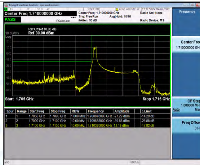
Band66-3MHz-16QAM-131987-1RB#14
