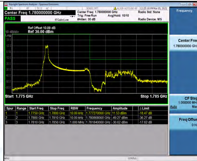
Band66-3MHz-16QAM-132657-1RB#14
