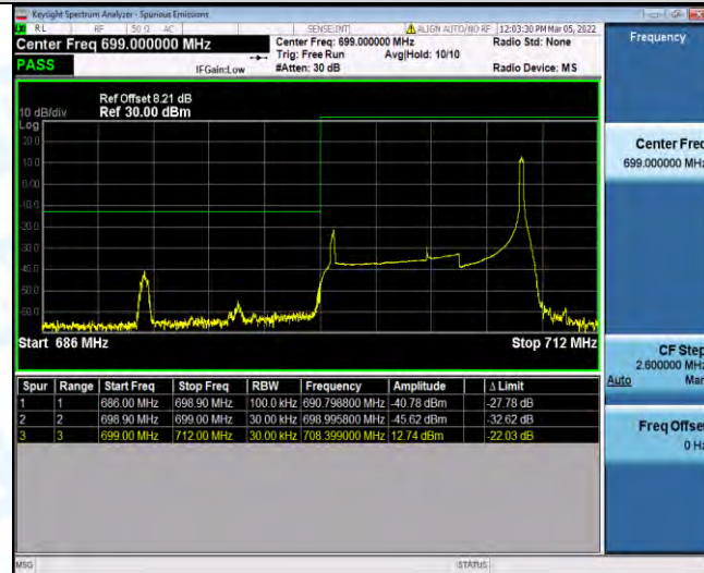
Band12-10MHz-16QAM-23060-50RB#0
