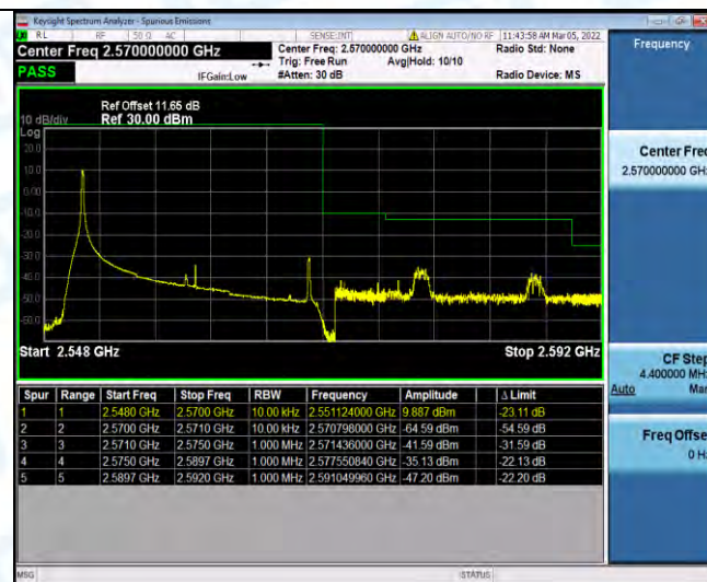
Band7-20MHz-QPSK-21350-1RB#99
