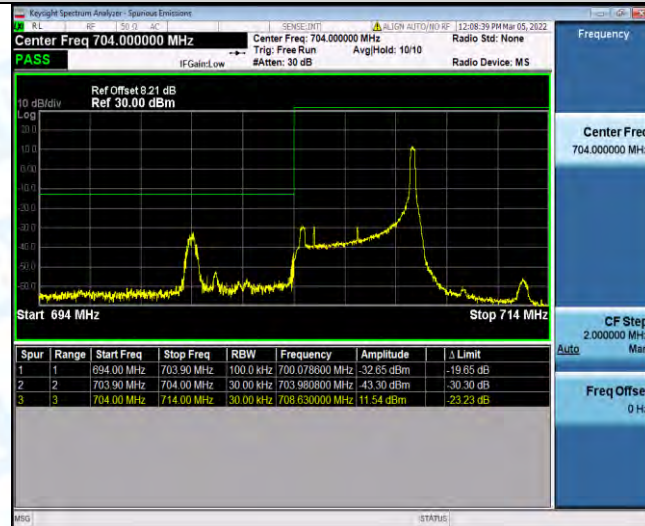
Band17-5MHz-16QAM-23755-25RB#0
