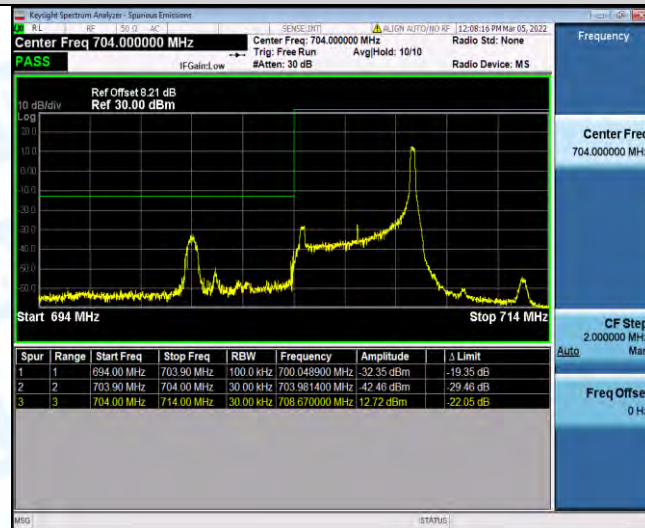
Band17-5MHz-QPSK-23755-25RB#0
