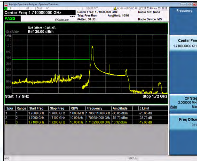
Band66-5MHz-16QAM-131997-1RB#24
