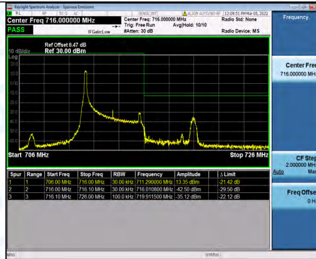
Band17-5MHz-QPSK-23825-1RB#24
