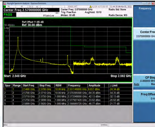
Band7-20MHz-16QAM-21350-1RB#99
