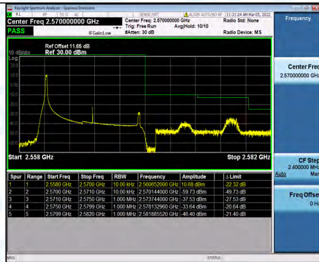
Band7-10MHz-QPSK-21400-1RB#49
