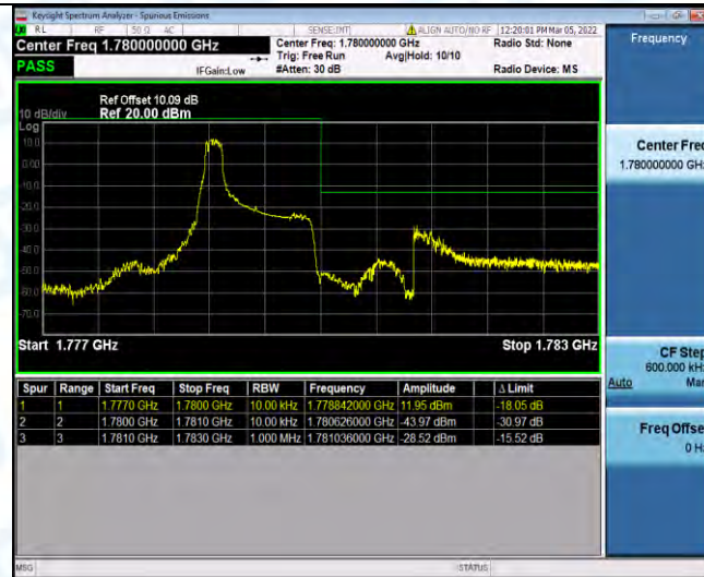
Band66-1.4MHz-QPSK-132665-1RB#5
