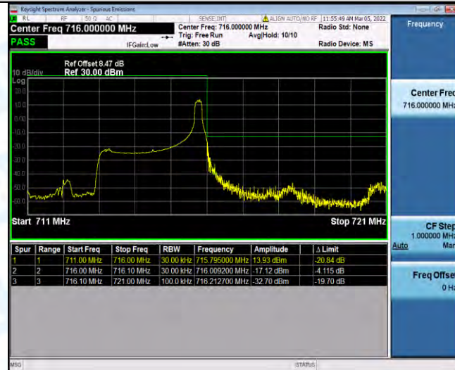
Band12-3MHz-16QAM-23165-15RB#0
