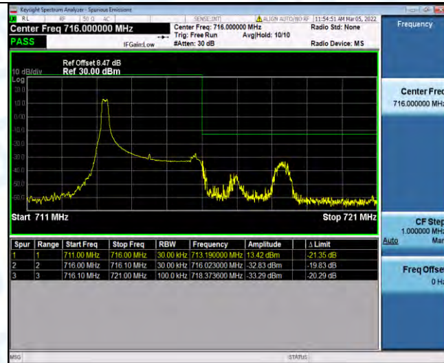
Band12-3MHz-16QAM-23165-1RB#14
