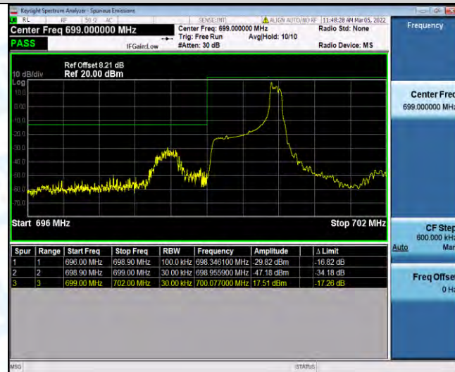
Band12-1.4MHz-16QAM-23017-6RB#0
