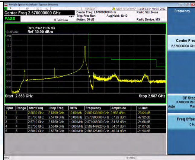
Band7-15MHz-QPSK-21375-75RB#0
