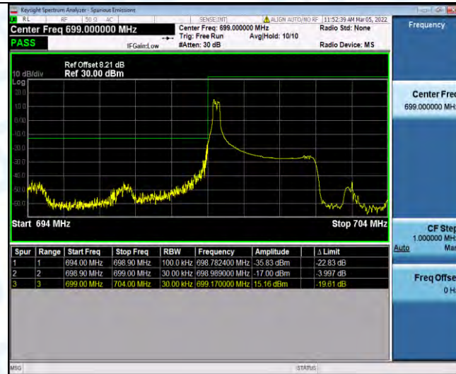
Band12-3MHz-16QAM-23025-1RB#14
