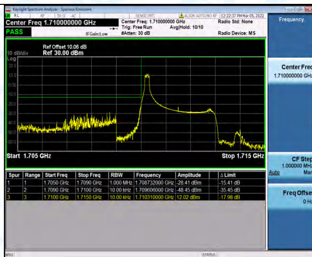
Band66-3MHz-QPSK-131987-1RB#14
