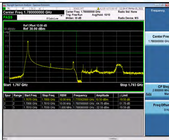
Band66-10MHz-QPSK-132622-1RB#49
