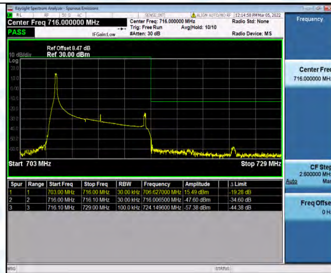
Band17-10MHz-QPSK-23800-1RB#49
