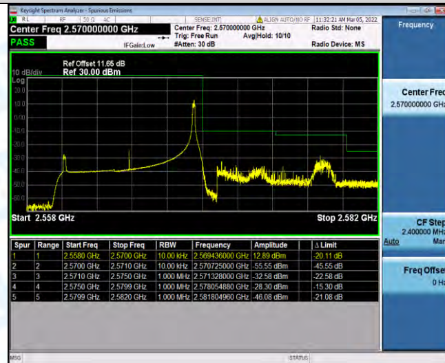
Band7-10MHz-QPSK-21400-50RB#0
