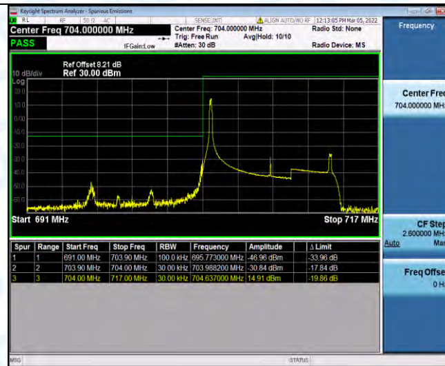
Band17-10MHz-16QAM-23780-1RB#49
