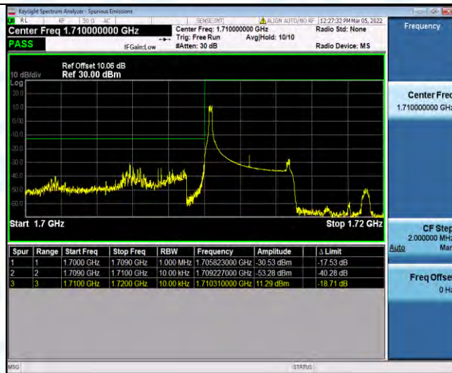
Band66-5MHz-QPSK-131997-1RB#24
