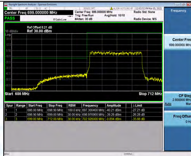
Band12-10MHz-QPSK-23130-1RB#0
