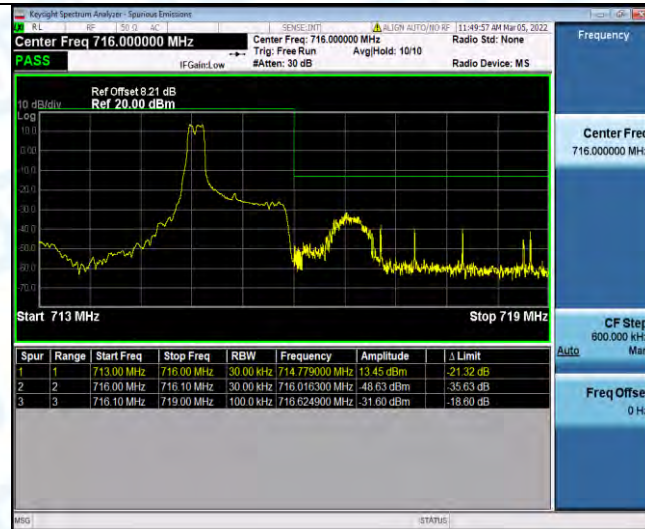
Band12-1.4MHz-16QAM-23173-1RB#5
