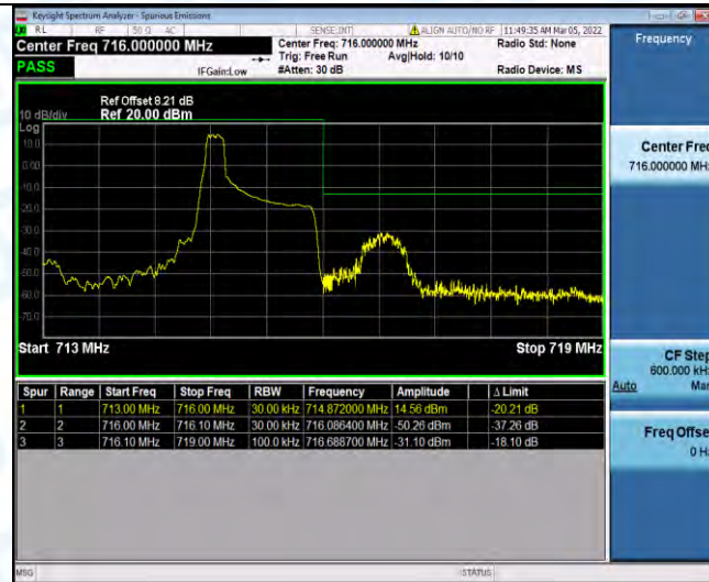
Band12-1.4MHz-QPSK-23173-1RB#5
