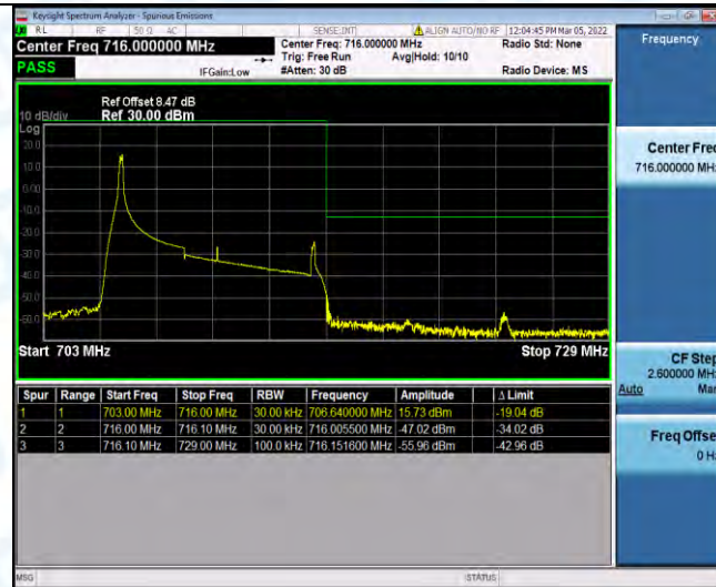
Band12-10MHz-QPSK-23130-1RB#49
