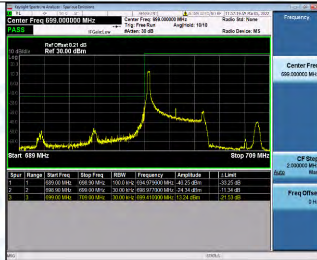
Band12-5MHz-QPSK-23035-1RB#24
