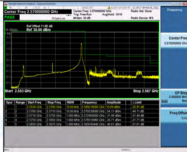
Band7-15MHz-16QAM-21375-75RB#0
