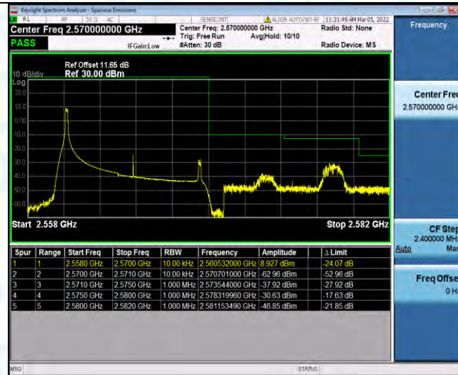
Band7-10MHz-16QAM-21400-1RB#49
