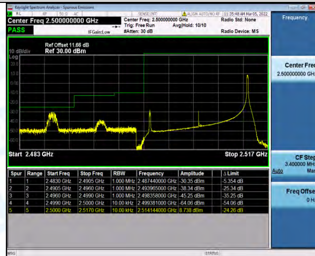
Band7-15MHz-QPSK-20825-75RB#0
