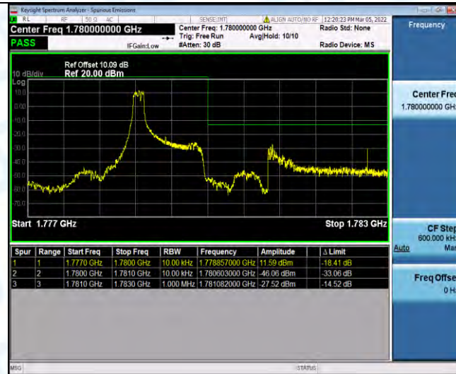
Band66-1.4MHz-16QAM-132665-1RB#5
