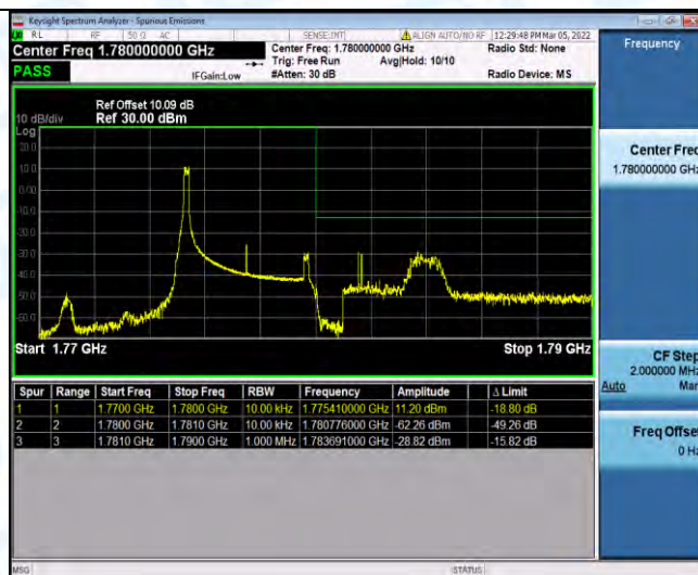
Band66-5MHz-QPSK-132647-1RB#24
