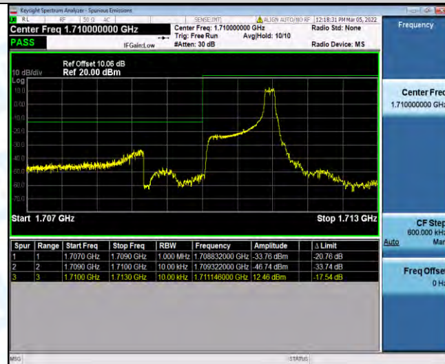
Band66-1.4MHz-QPSK-131979-6RB#0
