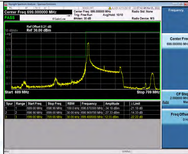
Band12-5MHz-16QAM-23035-1RB#24
