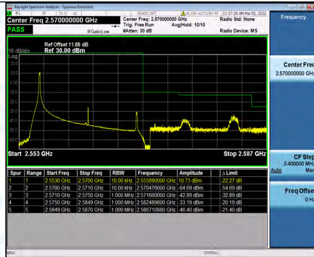
Band7-15MHz-QPSK-21375-1RB#74
