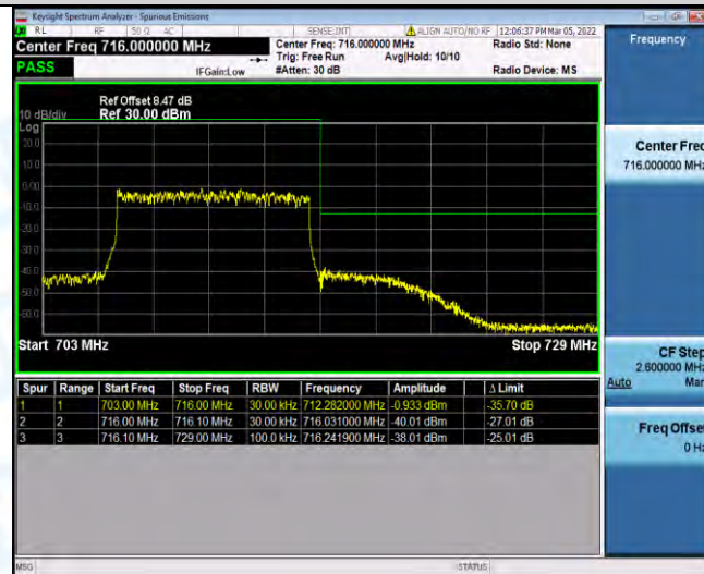
Band17-5MHz-QPSK-23755-1RB#0
