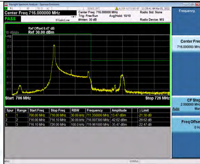
Band12-5MHz-QPSK-23155-1RB#24
