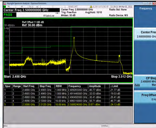
Band7-10MHz-16QAM-20800-1RB#49
