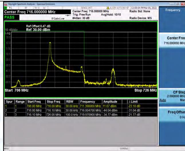
Band12-5MHz-16QAM-23155-1RB#24
