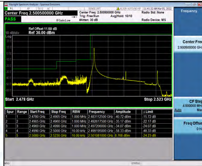
Band7-20MHz-QPSK-20850-1RB#99
