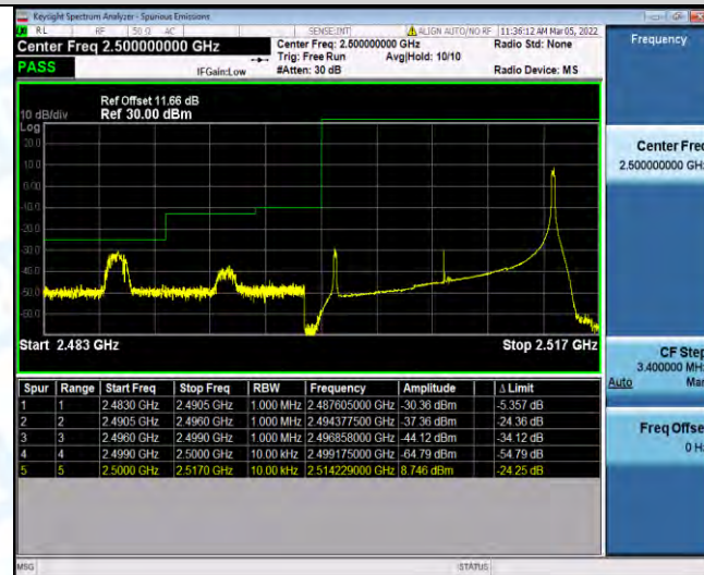
Band7-15MHz-16QAM-20825-75RB#0
