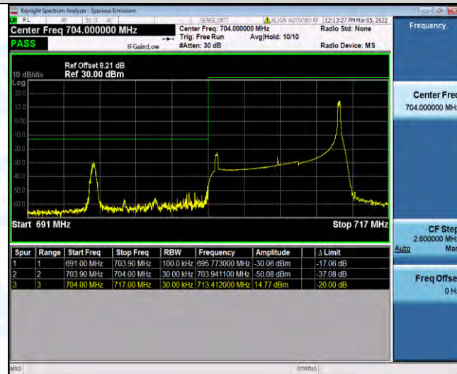
Band17-10MHz-QPSK-23780-50RB#0
