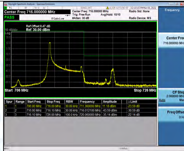
Band17-5MHz-16QAM-23825-1RB#24
