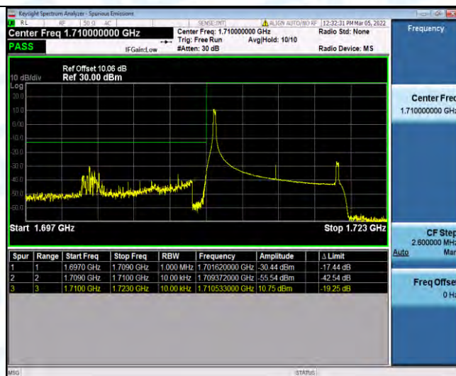
Band66-10MHz-QPSK-132022-1RB#49
