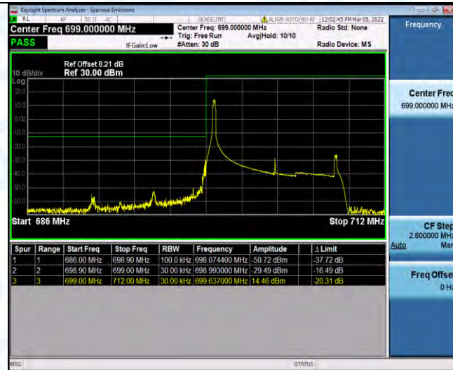
Band12-10MHz-16QAM-23060-1RB#49
