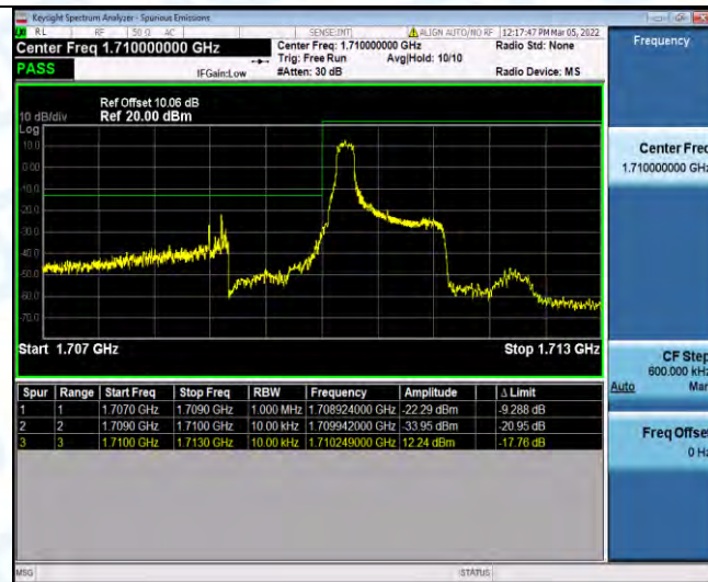
Band66-1.4MHz-QPSK-131979-1RB#5
