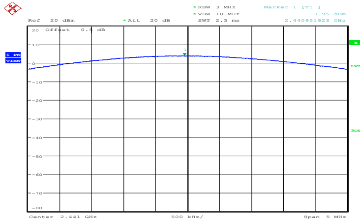
Middle channel 2441MHz
