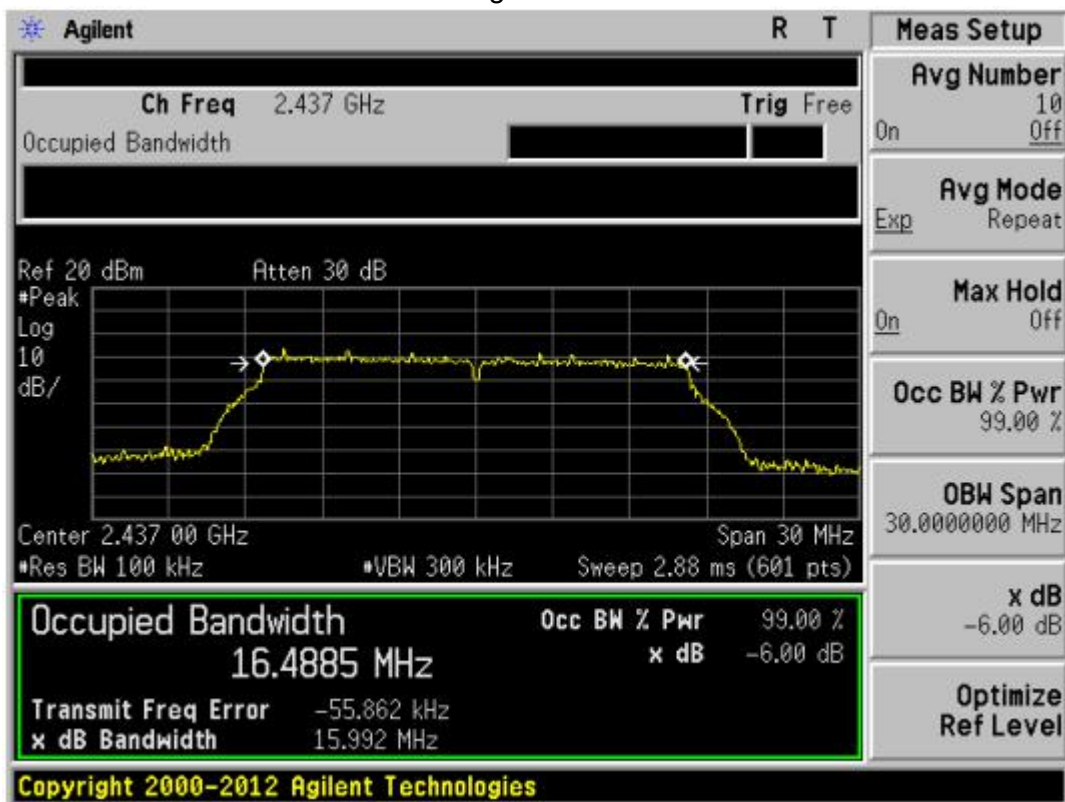
802.11g CH2437MHZ
