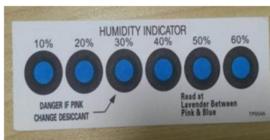
Figure 6-5 HIC for WBR1
