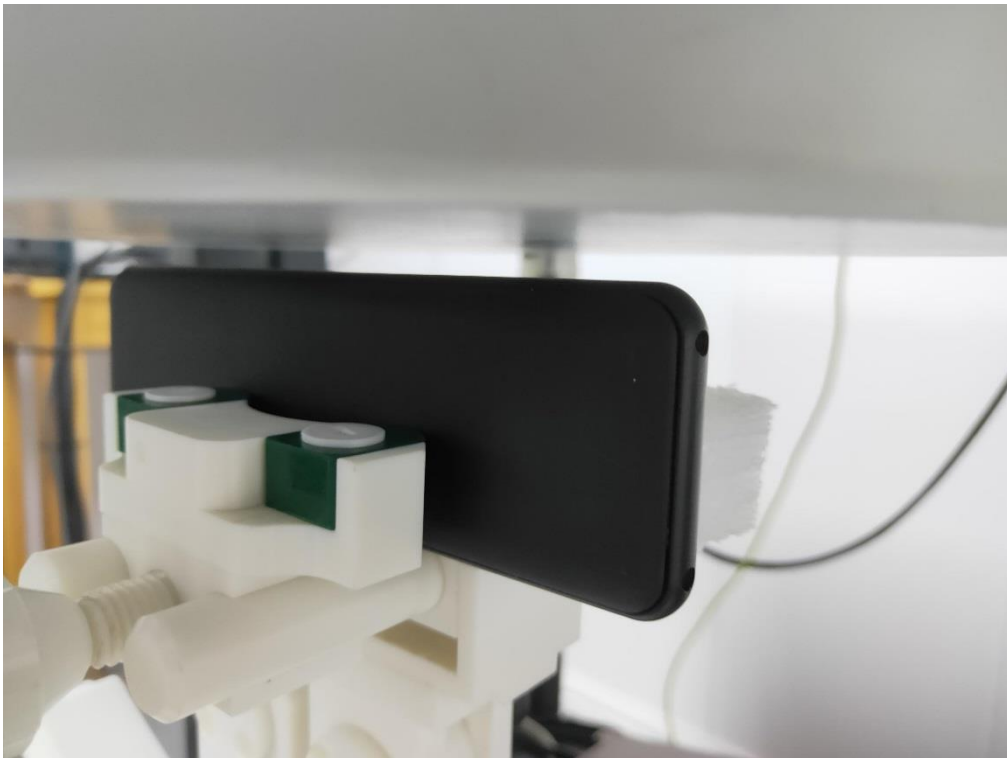
5mm body-worn Top Side Setup Photo
