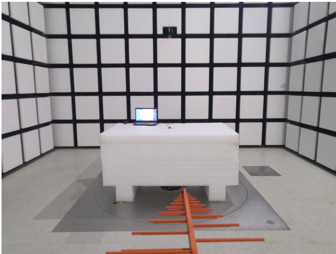
Radiated Emission Below 1GHz View X-C13SL-0
