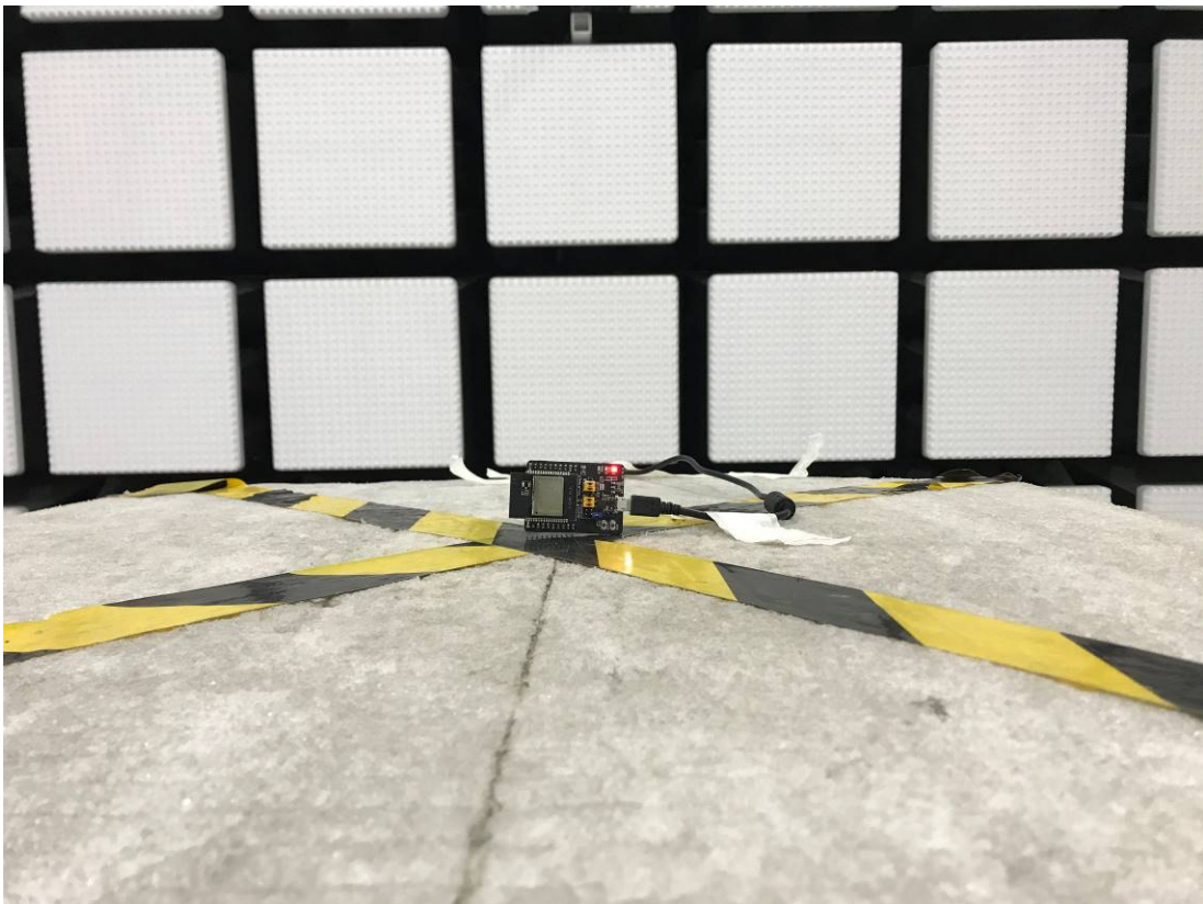
Radiated Emission Above 1GHz View X-C13SL-1
