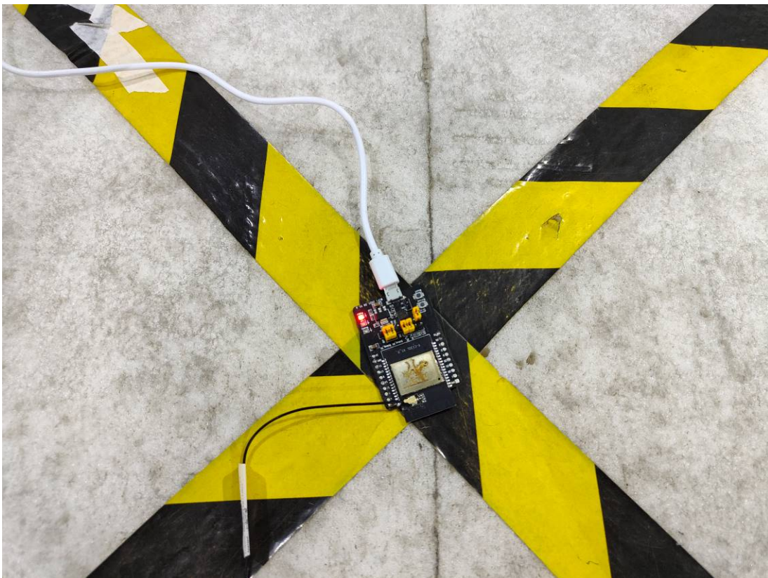
Radiated Emission Above 1GHz View X-C13SL-0
