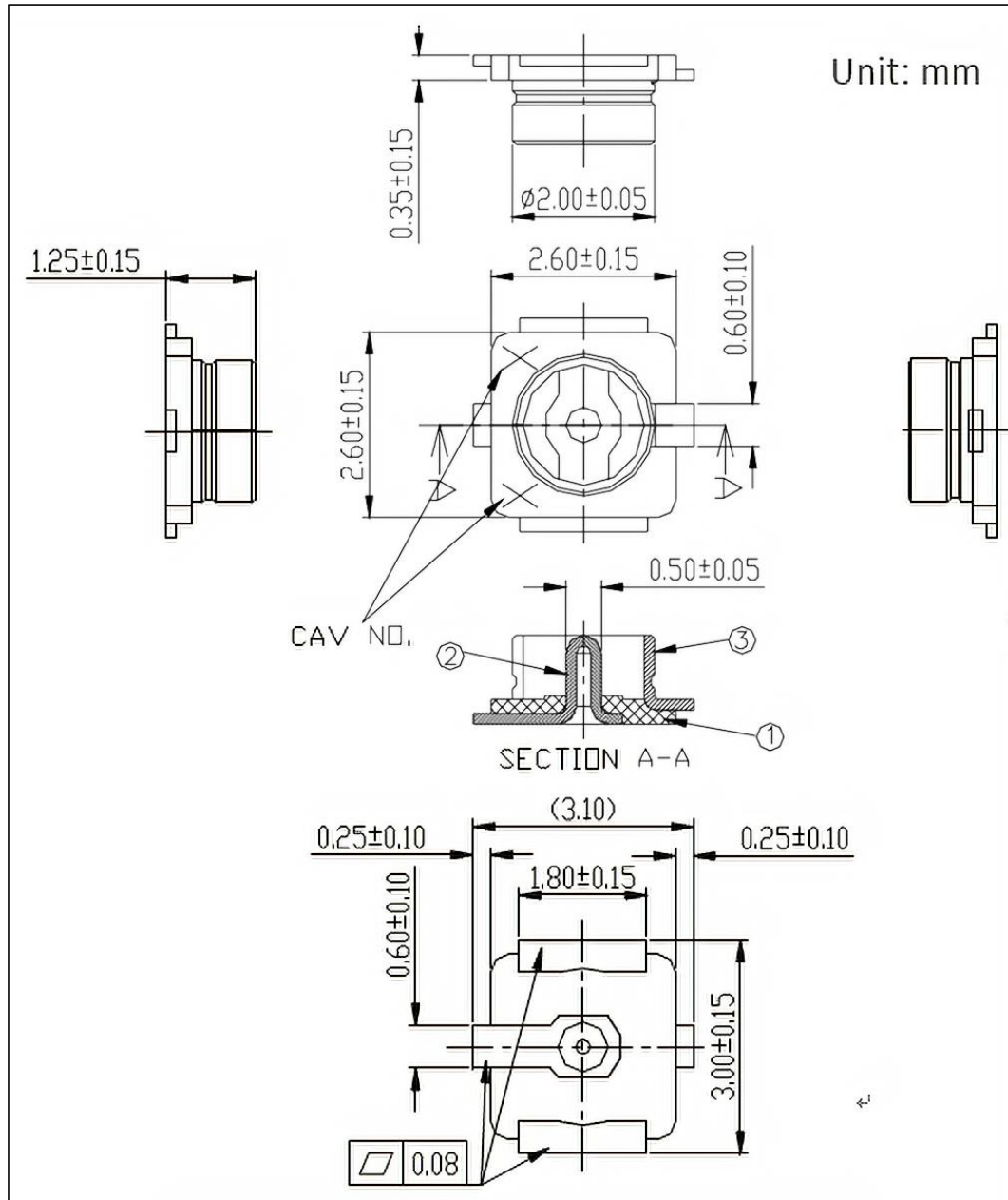
Figure 6. Dimensions of External Antenna Connector
