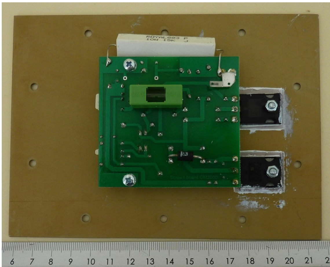
PCB - Screen board OM2000 (mounted on the metal plate at the bottom side of EUT)
