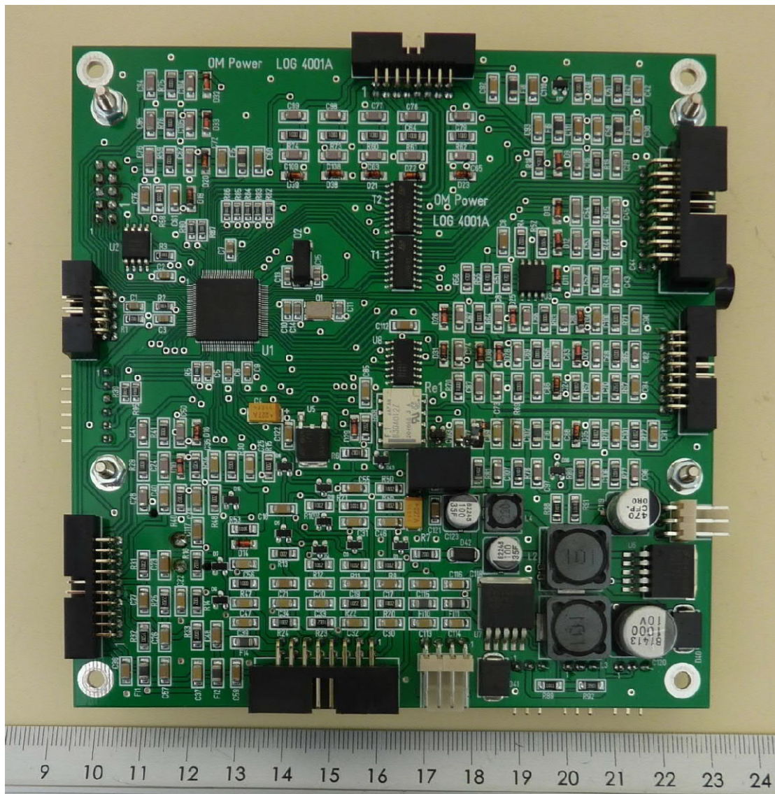
PCB – LOG 4001A, component side
