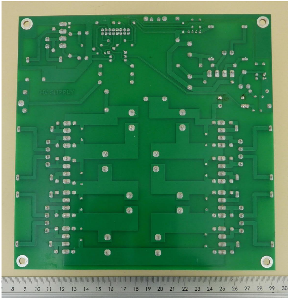
PCB – HV supply, bottom side
