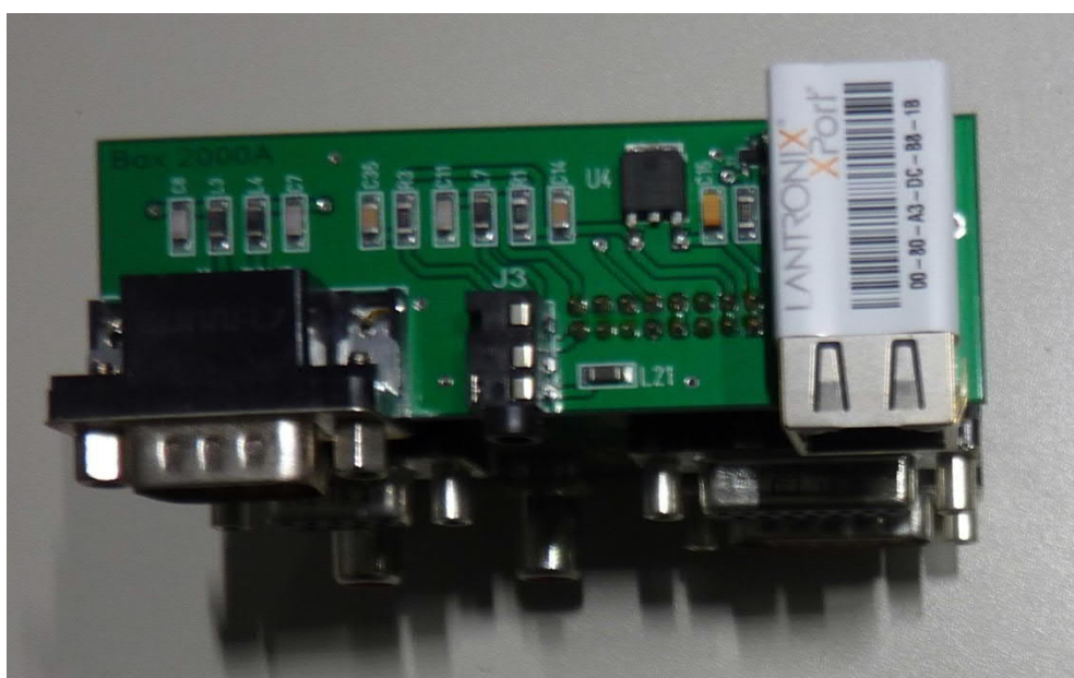
PCBs – BOX 2000A, connector side
