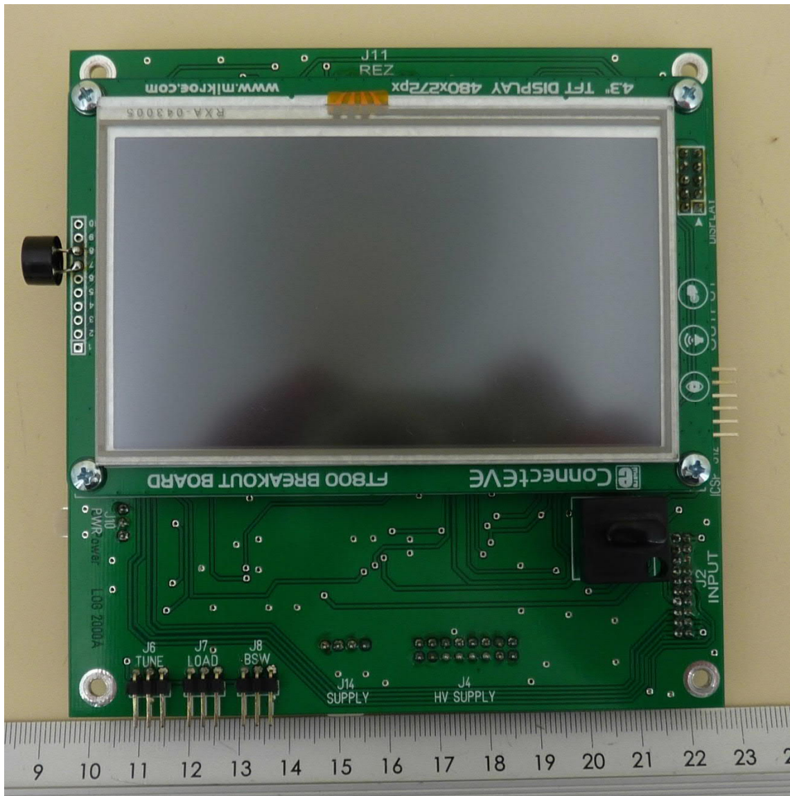
PCB – LOG 4001A, display side
