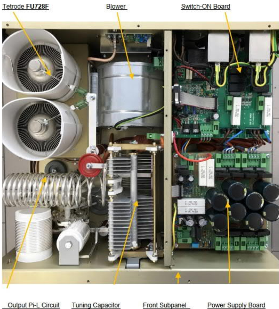
Top view on the opened OM4001A
