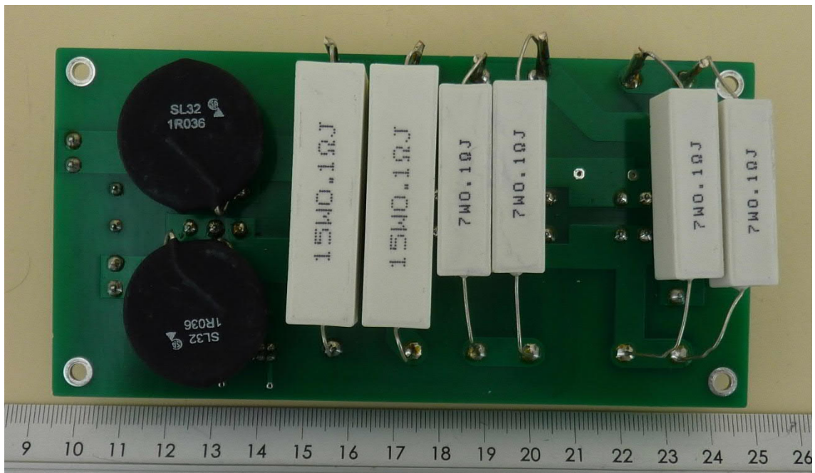
PCB – Heating control
