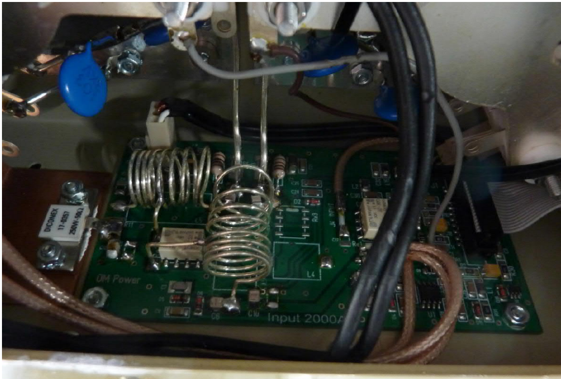
PCB - Input 2000A (Metal plate at the bottom side of EUT was removed)
