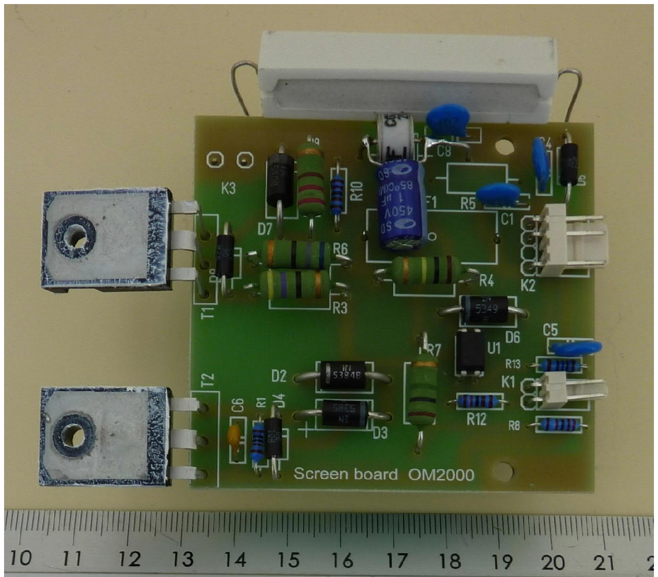
PCB - Screen board OM2000
