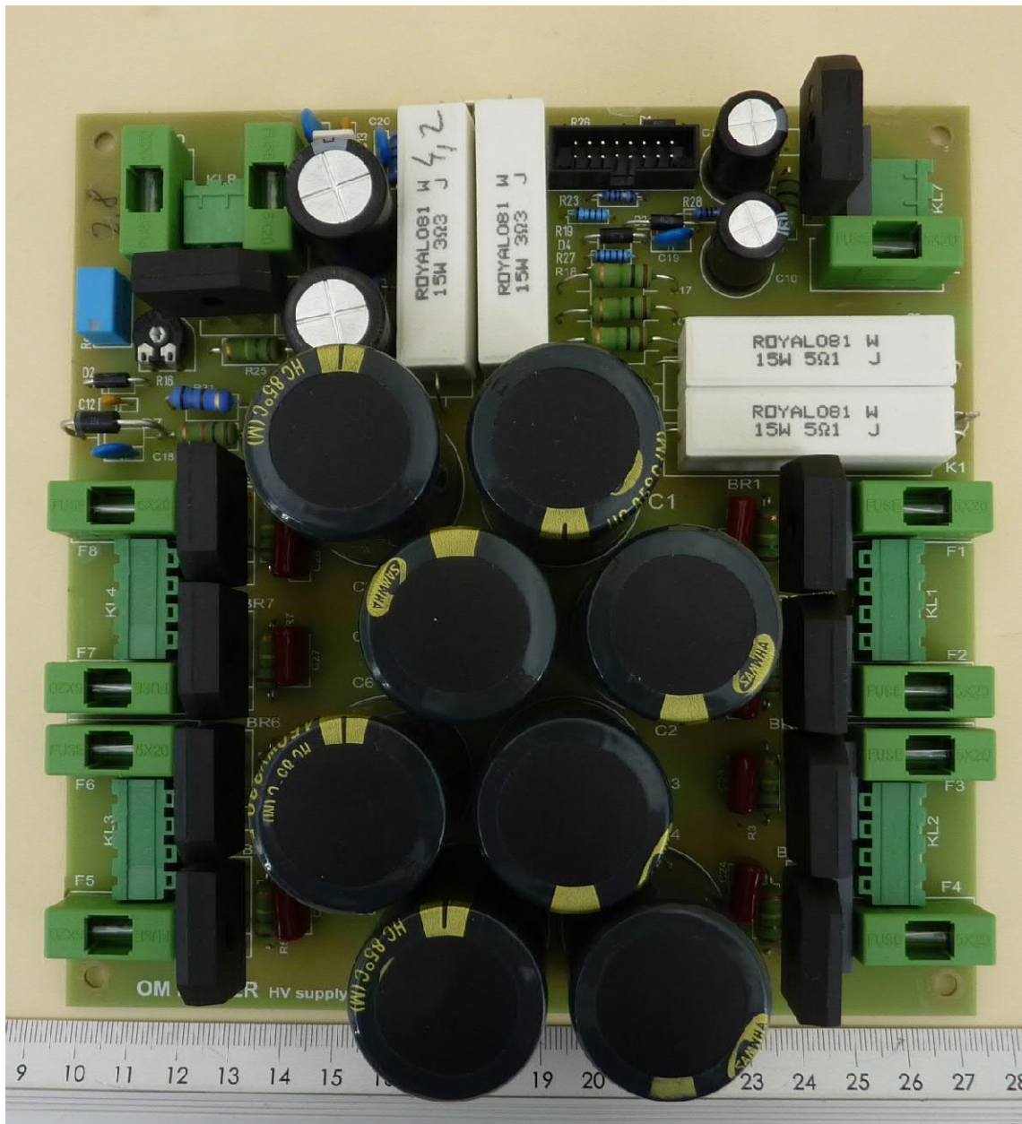
PCB – HV supply, component side
