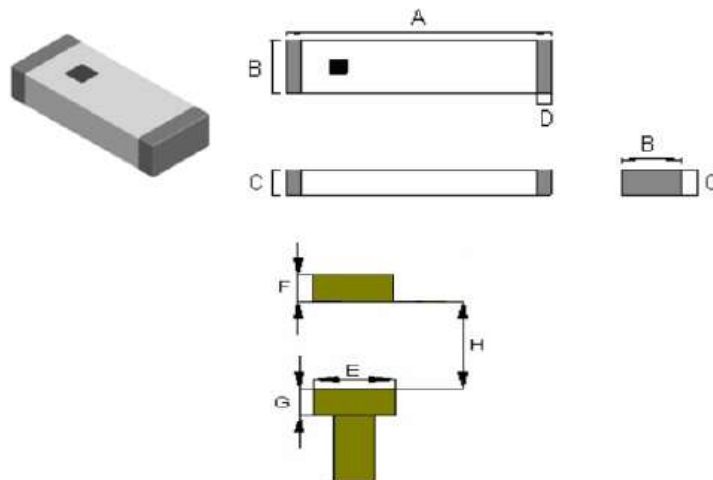
Product Dimensions and PCB Land Drawing (Unit: mm)
