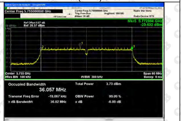
802.11ac(VH40)-5755
