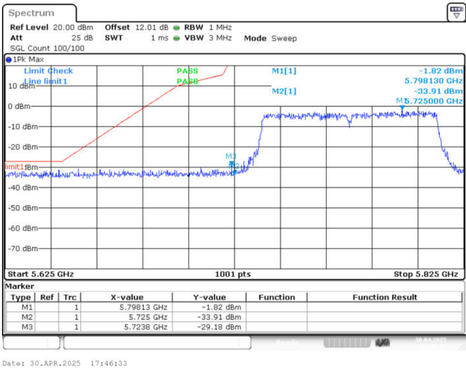
Band Edge NVNT ac80 5775MHz High Ant1
