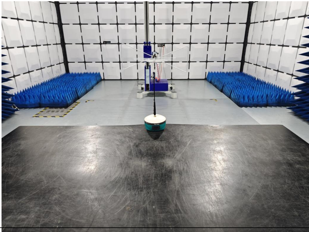
NCT TEST
